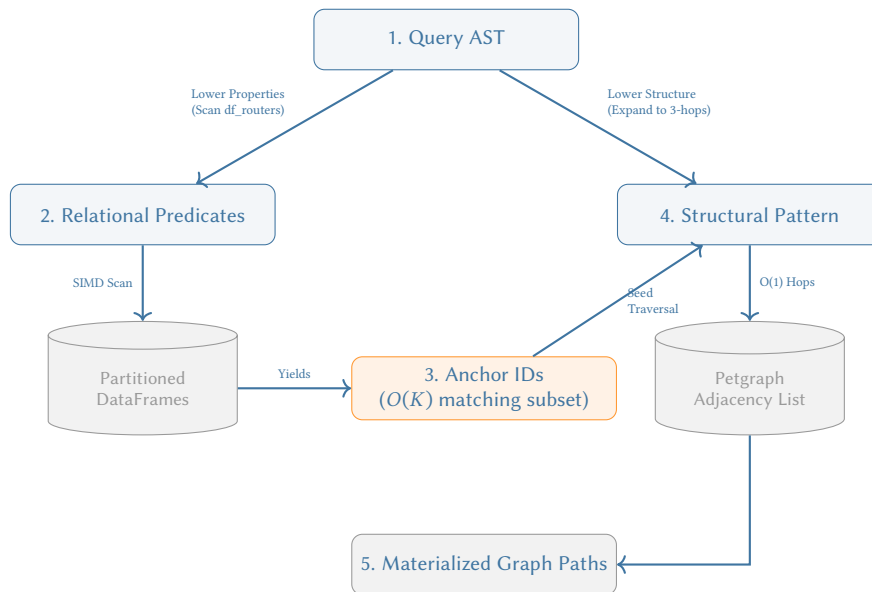
Figure 33. The Filter-First Hybrid Execution Pipeline. During the AST compilation phase, the engine splits the query. It executes highly-selective property predicates against partitioned columnar storage first , yielding a tiny subset of Anchor IDs. These anchors seed the expanded 3-hop structural graph traversal, guaranteeing that the engine never traces paths from irrelevant nodes.
