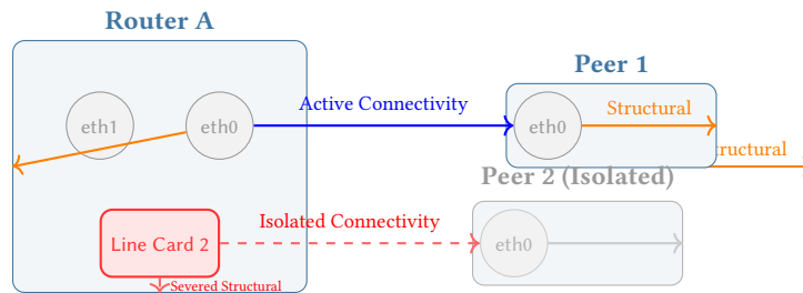
Figure 7. Blast Radius Propagation. When Line Card 2 fails, its outgoing Structural edge is severed. Consequently, the Connectivity connection to Peer 2 is isolated from the main device graph. Because eth0 and eth1 reside on different logical endpoints, their Structural edges remain intact, leaving the connection to Peer 1 unaffected. A naive (Router)-[CONNECTED_TO]->(Router) model cannot express this partial failure state.
