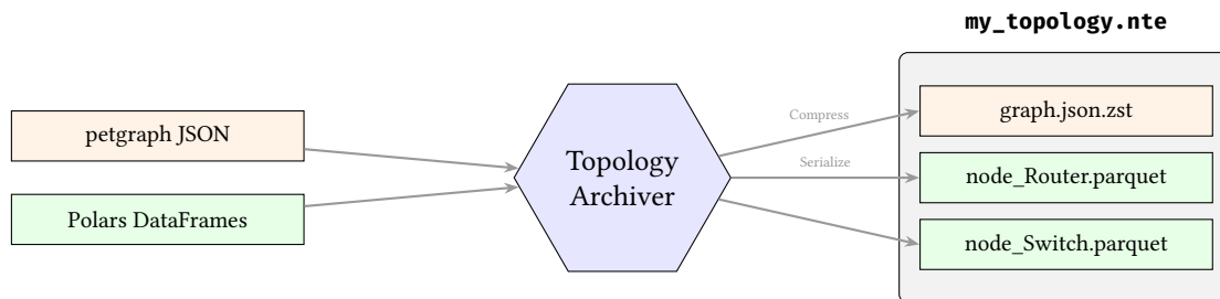
Figure 41. The .nte archive format. Structural graph data is compressed via zstd, while DataFrames are serialised directly to columnar Parquet files, all packaged into a standard ZIP archive.
