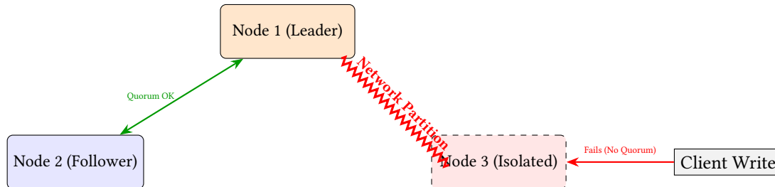
Figure 53. Split-Brain Resolution. In a partition, the isolated Node 3 rejects writes because it cannot replicate logs to a majority quorum. Nodes 1 and 2 continue processing safely.
