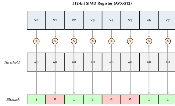
Figure 25. Hardware-Level Predicate Evaluation. A single AVX-512 instruction evaluates multiple property values in parallel, producing a bitmask that drives the subsequent graph traversal filter.
