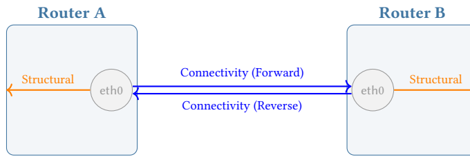
Figure 4. The Three-Hop Connectivity Pattern. To traverse from Router A to Router B, the path is: Router A \leftarrow Structural \leftarrow eth0 \rightarrow Connectivity \rightarrow eth0 \rightarrow Structural \rightarrow Router B. A bidirectional link is stored as two explicit directed Connectivity edges.
