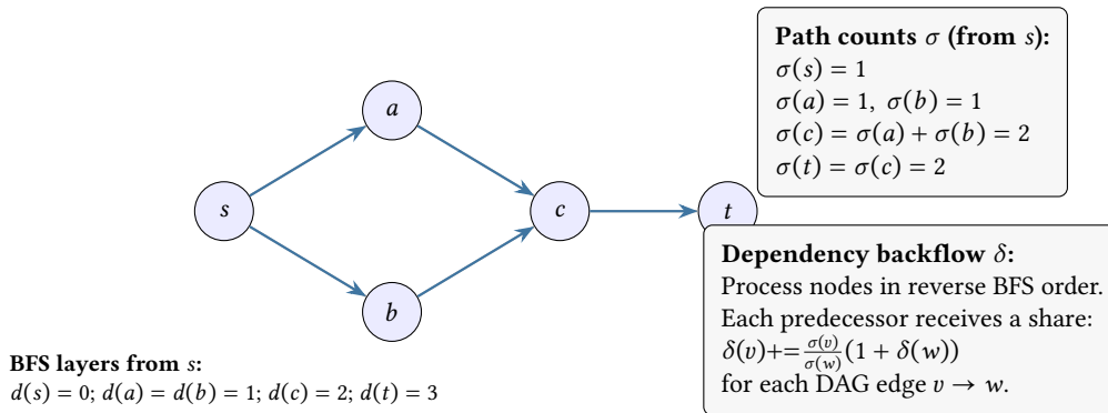
Figure 15. Brandes betweenness centrality as a conserved “flow” on the shortest-path DAG. The forward BFS counts how many shortest paths reach each node ( \sigma ). The reverse accumulation distributes dependency ( \delta ) back to predecessors in proportion to their contribution.
