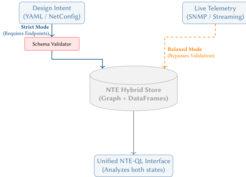
Figure 2. Bimodal Execution Architecture. Strict mode forces design intent through schema validation (ensuring the Endpoints model is perfectly adhered to). Relaxed mode bypasses validation, allowing live telemetry to stream directly into the engine. Both modes share the same unified NTE-QL interface.
