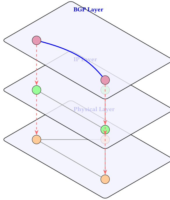
Figure 8. The 3D layered topology model. Logical overlays (BGP, IP) project down onto their physical underlays via structural dependencies.
