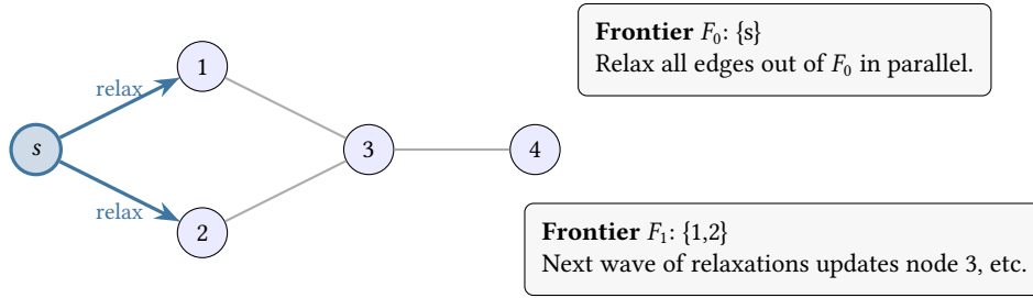
Figure 19. GPU SSSP as wavefront relaxation. Each iteration processes a frontier of active vertices and relaxes outgoing edges in parallel. This maps naturally onto GPU execution when adjacency is stored in compact buffers.
