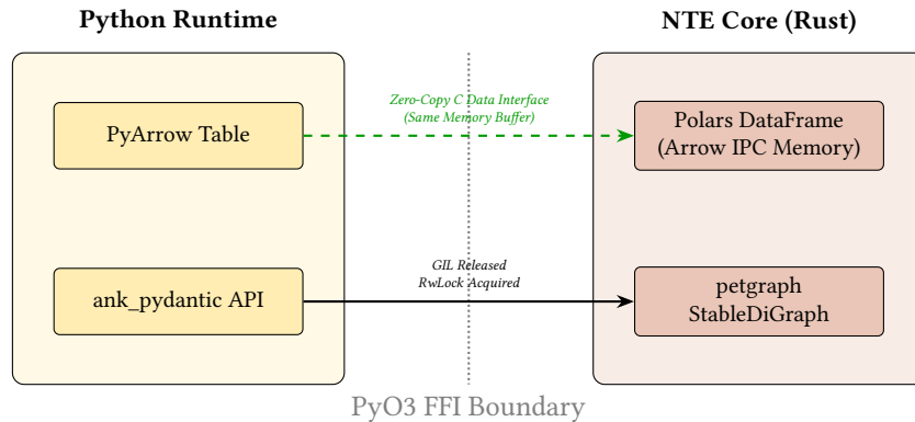
Figure 27. The FFI Zero-Copy Boundary. Unlike traditional RPC-based graph databases, NTE embeds directly in the Python process. The Arrow C Data Interface allows Python tools to read the Rust memory buffers without any serialization overhead.
