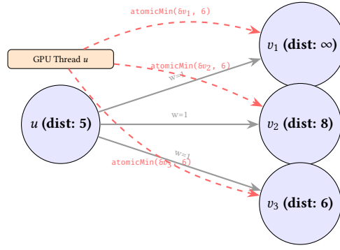
Figure 45. GPU SSSP relaxation. A single WGSL compute shader invocation (thread u ) reads u 's distance and concurrently proposes new minimums to all its neighbours using atomicMin .
