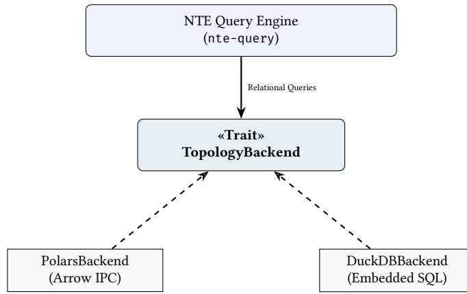
Figure 28. Trait-Based Abstraction. The core query engine interacts only with the TopologyBackend interface, allowing the physical columnar storage (Polars vs. DuckDB) to be swapped at compile time.
