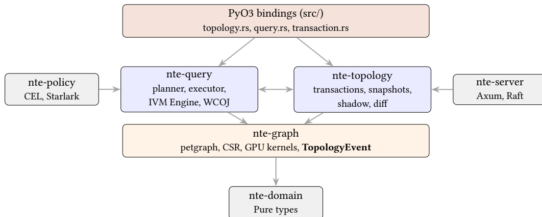
Figure 9. The Layered Crate Architecture. Shared foundation types (Events) are pushed down to nte-graph to enable clean, uni-directional dependency flow between the query engine and topology manager.
