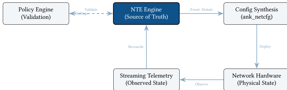
Figure 50. The Autonomous Closed-Loop Cycle. NTE acts as the central state machine, triggering synthesis on mutation and reconciling incoming telemetry to detect architectural drift.
