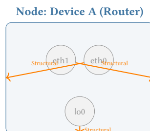
Figure 3. Nodes vs. Endpoints. The bounding box represents the Node . The circles represent Endpoints . The Structural edges represent ownership, explicitly pointing from the Endpoint to the parent Node.
