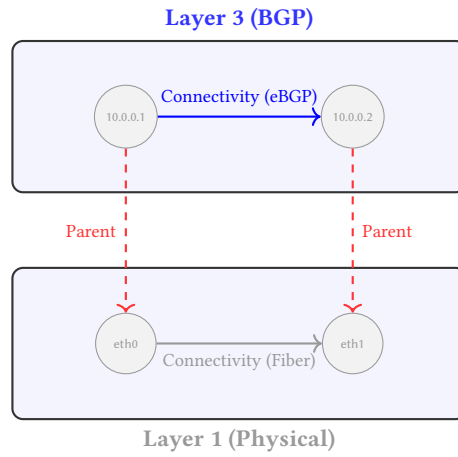
Figure 6. Cross-Layer Relationships. The L3 BGP Endpoints (IP addresses) are bound to the L1 Physical Endpoints (Ethernet ports) via Parent edges. If the eth0 port fails, the graph can traverse the incoming Parent edge to deterministically tear down the dependent BGP session.
