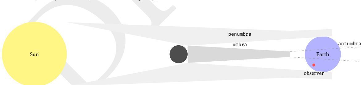
Figure 27. Eclipse shadow geometry (cross-section): the Moon casts an umbral cone (total shadow), penumbral cone (partial shadow), and antumbra (annular shadow region beyond the umbral vertex).
