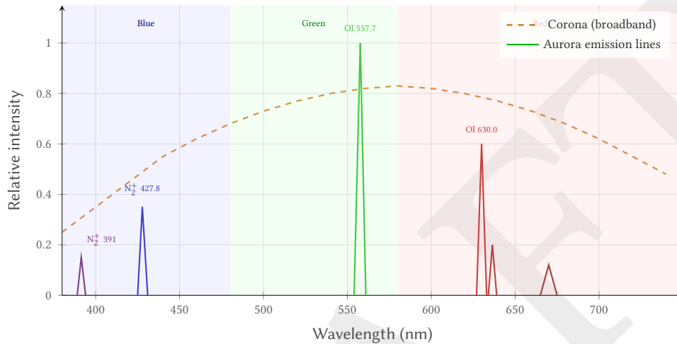
Figure 46. Spectral comparison: aurora produces discrete emission lines (dominant OI green at 557.7 nm, OI red at 630 nm, N 2 + blue at 427.8 nm) while the solar corona emits broadband continuum light. Bayer filter channel boundaries shown as background shading. The green channel’s sensitivity to the dominant 557.7 nm aurora line explains why green clips first.
