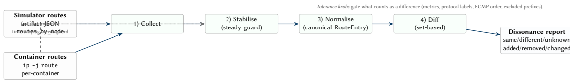
Figure 2. Routing dissonance as a four-stage pipeline with symmetric inputs. Stabilisation prevents convergence snapshots from becoming false positives; normalisation makes the diff vendor-independent.
