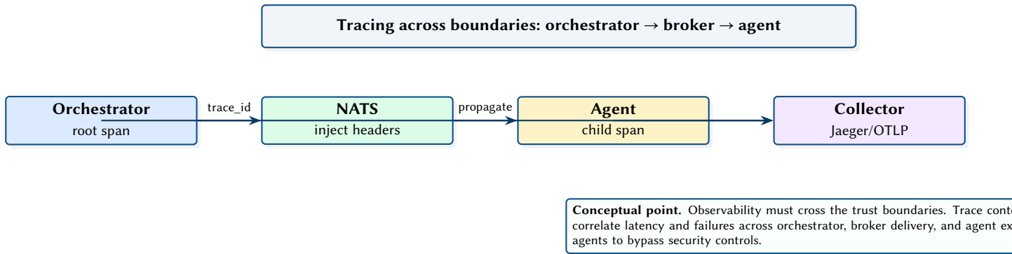
Figure 5. Distributed tracing across the orchestrator–broker–agent chain. Trace context propagates via message headers, enabling end-to-end latency attribution.
