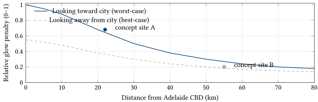
Figure 14. Concept: city glow penalty decreases with distance and improves when shooting away from the city. The UI uses this idea to explain why a site can be good for one azimuth and mediocre for another.
