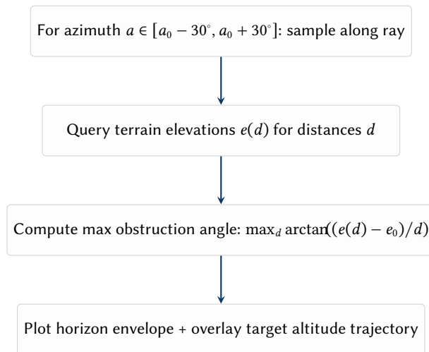
Figure 18. Horizon obstruction estimation pipeline used for the trajectory plot.
