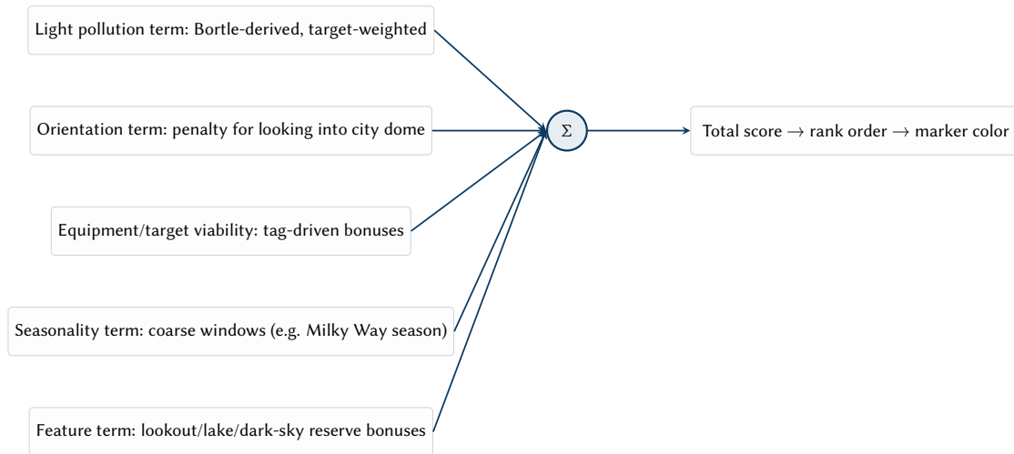
Figure 6. Conceptual structure of the heuristic site score.
