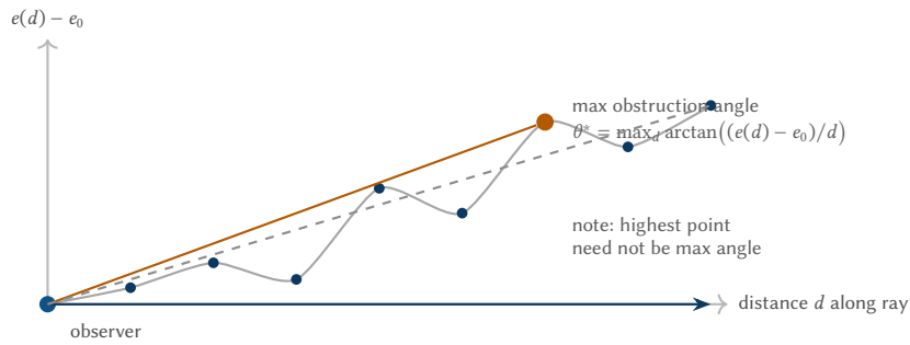
Figure 17. Horizon obstruction algorithm intuition (single ray). The app samples terrain elevations along a viewing ray and converts elevation differences into angles. The horizon envelope for a target azimuth is the maximum obstruction angle in a small azimuth sweep around the target.
