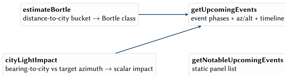
Figure 4. Astronomy module responsibilities and how they feed the UI.
