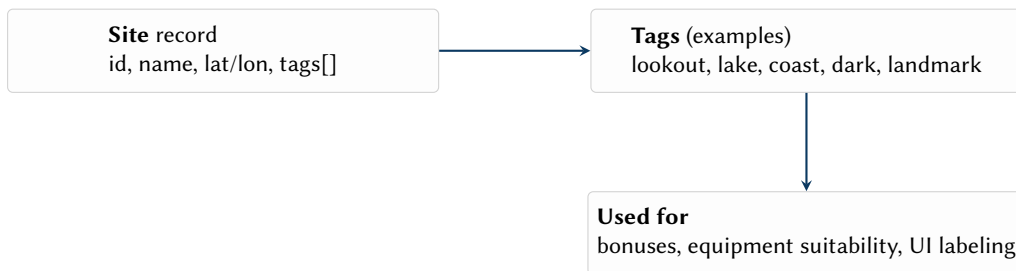
Figure 7. Site corpus modeling: minimal records, expressive tags.
