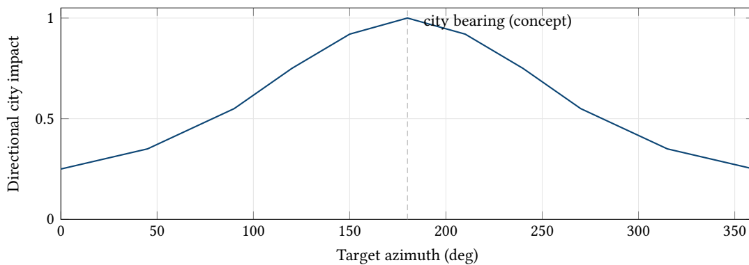
Figure 10. Concept: directional city-glow impact as a function of azimuth. This is the mechanism that allows the same site to score differently depending on where the camera points.
