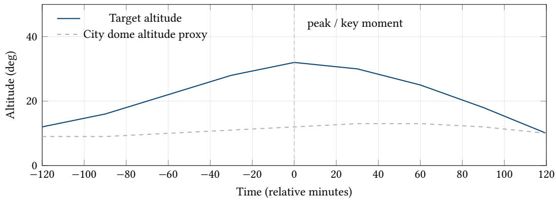
Figure 11. Concept: glow clearance at the time that matters. The UI compares an estimated dome height against the target altitude to identify when glare is likely to wash out contrast.
