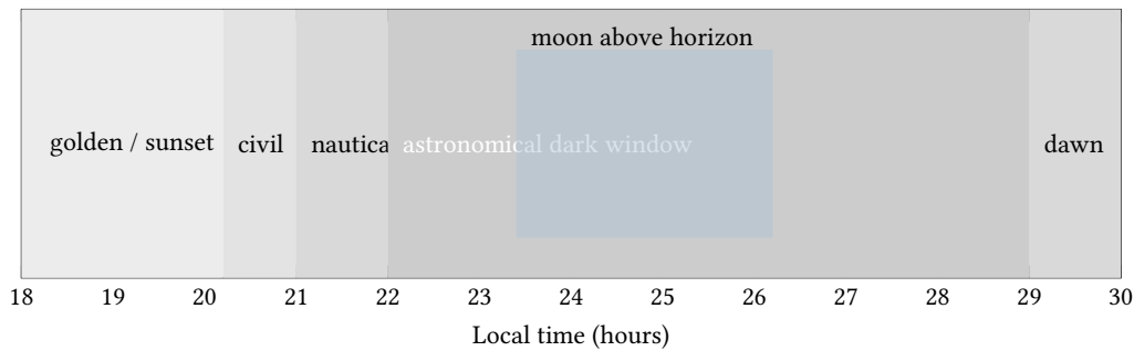
Figure 8. Concept: darkness timeline as a single banded view. The UI renders a concrete planning window (astronomical darkness) and overlays moonrise/moonset to avoid wasted travel time.
