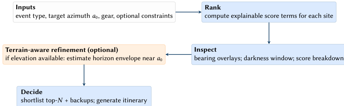
Figure 3. Algorithmic view of the planning loop. The system first computes a cheap, explainable score across the site corpus, then conditionally runs a more expensive terrain-aware horizon estimation only for candidate sites being inspected. This keeps the common case interactive while still answering the practical question: "will it be blocked at the time that matters?"
