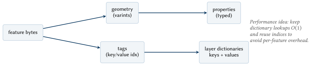
Figure 11. MVT bytes decomposition: geometry and tags; tag indices depend on layer-level key/value dictionaries.
