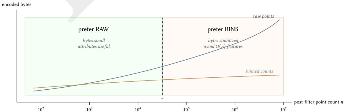
Figure 5. Bytes budget model: raw tiles grow with point count; binned tiles target a near-constant feature/byte budget.
