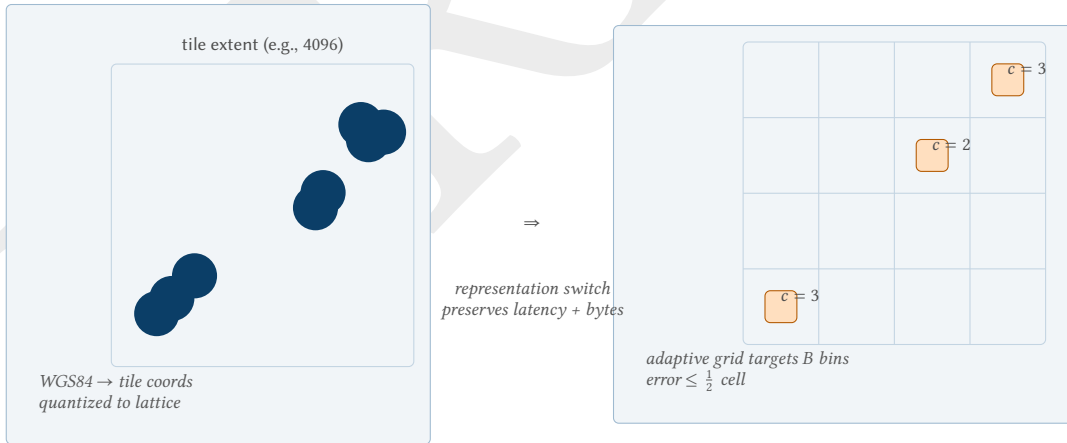
Figure 7. Algorithm geometry: point projection into tile space and the resulting adaptive grid bin representation.
