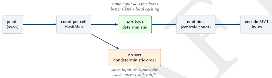
Figure 9. Performance/caching concept: determinism in bin emission improves cache hit rate and reduces downstream churn.
