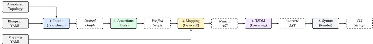
Figure 14. NetCfg compilation pipeline. High-level intent is progressively lowered through three distinct AST representations (Verified Graph, Neutral AST, Concrete AST) before serialisation.
