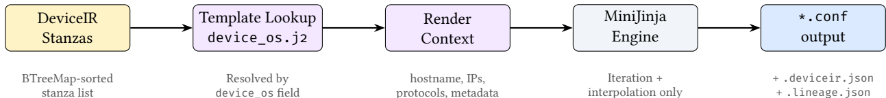
Figure 19. Template rendering pipeline. DeviceIR stanzas are resolved to a vendor template, combined with a render context, and emitted by the MiniJinja engine as configuration text plus audit artefacts.
