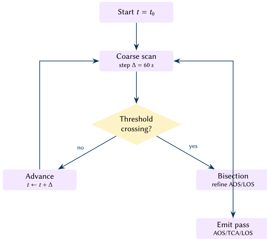
Figure 5. Pass prediction control flow: a coarse scan detects elevation threshold crossings; bisection refinement recovers sub-second AOS/LOS times.
