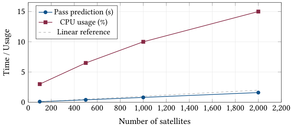
Figure 8. Resource scaling with satellite count. Both CPU usage (mid-range values) and pass prediction time scale linearly. The dashed line shows ideal linear scaling from the 100-satellite baseline.
