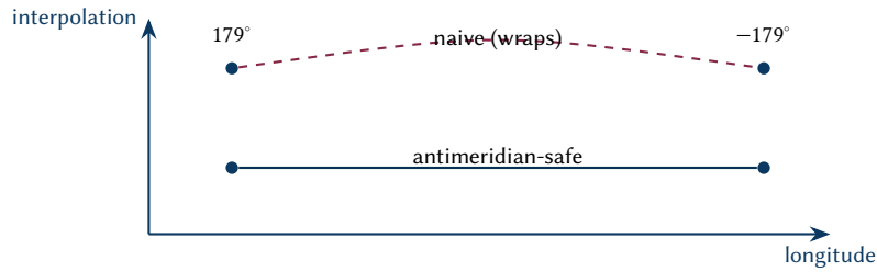
Figure 7. Antimeridian-safe longitude interpolation. Longitudes near \pm 180^\circ must be wrapped to follow the shortest path across the antimeridian.
