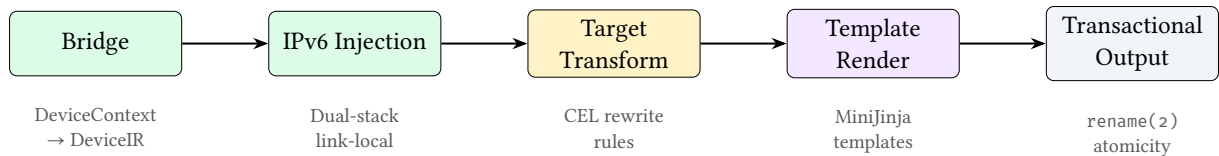
Figure 18. TSDM lowering pipeline. DeviceIR stanzas pass through bridge translation, optional IPv6 injection, target-specific AST rewriting, template rendering, and transactional file output.
