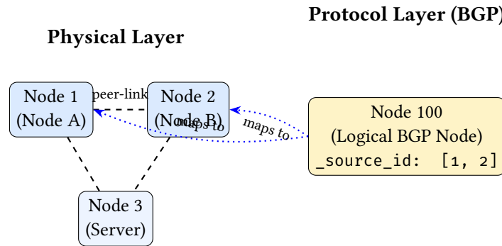
Figure 22. MLAG/vPC topology mapping. Two physical nodes collapse into a single logical protocol node via array _source_id .
