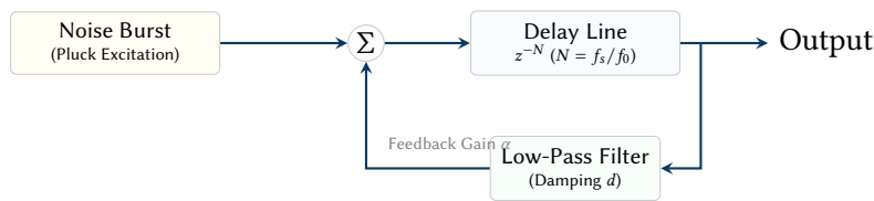
Figure 15. Karplus-Strong physical modeling architecture. A short burst of noise (the “pluck”) is fed into a delay line representing the string length. The output is fed back through a low-pass filter, causing higher frequencies to decay faster than fundamental frequencies, realistically simulating a plucked acoustic string.
