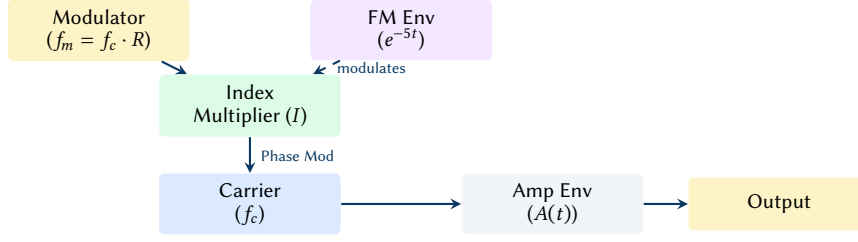
Figure 14. Lead synthesiser signal flow using 2-operator FM.
