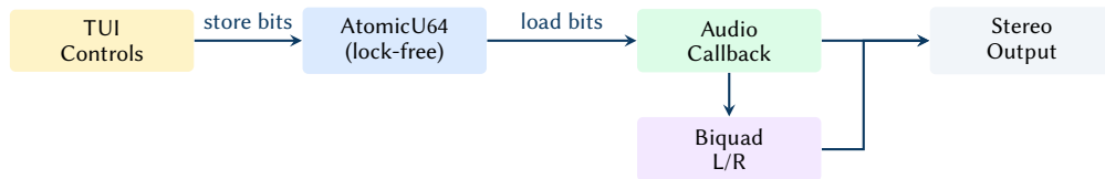
Figure 57. Lock-free live parameter path: the TUI stores f64 bit patterns into atomics; the audio callback loads them each block and updates the biquad filter only when thresholds are exceeded.
