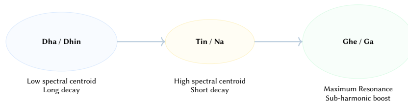
Figure 42. Mapping percussive syllables (bols) to spectral synthesis. The engine modifies the ADSR and filter bank of the percussive generator based on the syllable metadata attached to each event.
