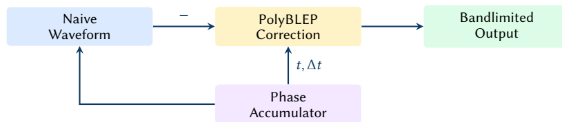
Figure 22. PolyBLEP anti-aliasing: the correction term is subtracted from the naive waveform at phase discontinuities.
