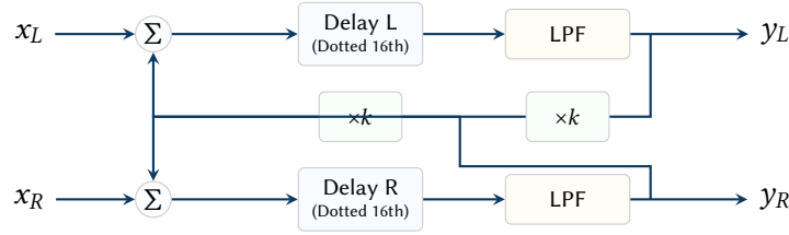
Figure 18. Ping-Pong Delay topology. Left and right channel inputs ( x_L , x_R ) are fed into independent delay lines. The output of each delay line is low-pass filtered (for analog-style damping), multiplied by the feedback coefficient k , and routed into the input sum of the opposite channel's delay line, creating a stereo bouncing effect.
