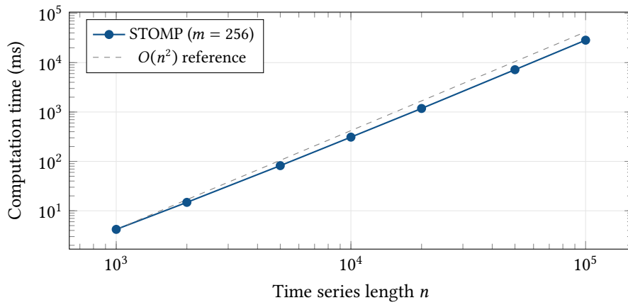
Figure 26. STOMP batch scaling. Measured times track ideal O(n^2) scaling closely across two orders of magnitude.
