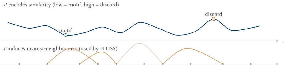
Figure 7. Downstream tasks as representations. Motifs and discords come from extrema in the profile vector P , while regime segmentation uses structure in the index vector I (nearest-neighbour arcs) as in FLUSS [7].
