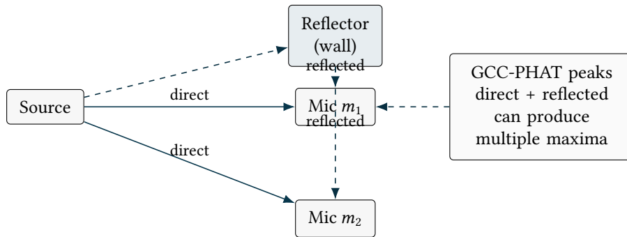
Figure 11. Multipath creates multiple plausible delays. Peak selection should be constrained by physically plausible bounds derived from array aperture and speed of sound.
