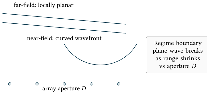
Figure 12. Near-field vs far-field is a model boundary. If the plane-wave assumption fails, DoA-only inference may be biased and a range-bearing model becomes appropriate.
