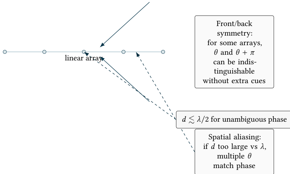
Figure 18. DoA identifiability constraints. Symmetry can cause 180-degree ambiguity; large inter-mic spacing can cause spatial aliasing at higher frequencies. Use geometry choices and auxiliary cues (asymmetry, higher-order arrays, or priors) to break ambiguity.
