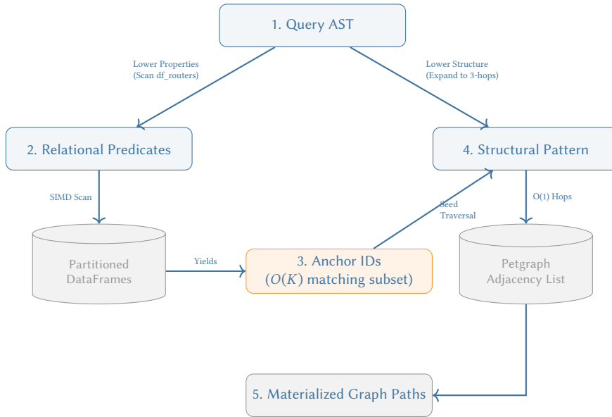
Figure 37. The Filter-First Hybrid Execution Pipeline. During the AST compilation phase, the engine splits the query. It executes highly-selective property predicates against partitioned columnar storage first , yielding a tiny subset of Anchor IDs. These anchors seed the expanded 3-hop structural graph traversal, guaranteeing that the engine never traces paths from irrelevant nodes.
