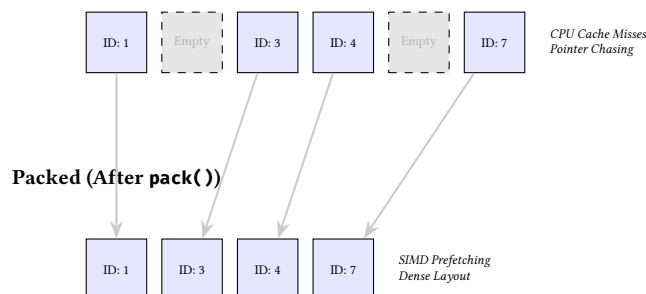
Figure 20. Memory Defragmentation (Graph Packing). The pack() operation removes tombstone slots from the internal adjacency arrays, restoring linear CPU cache locality and reducing memory overhead.
