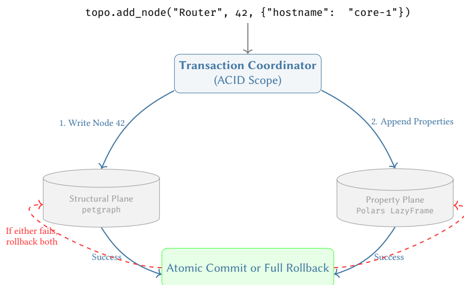
Figure 42. The Dual-Write Transaction Model. Mutations are coordinated atomically across the divergent storage engines. If a node is added to the graph but the properties fail schema validation in Polars, the entire transaction aborts, ensuring the digital twin never enters a split-brain state.
