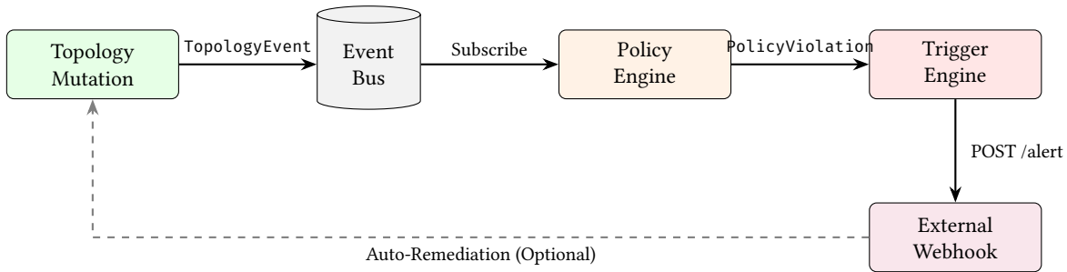
Figure 60. Proposed Reactive Topology workflow: Automated policy validation pushing events to the Trigger Engine rather than waiting for pull-based queries.
