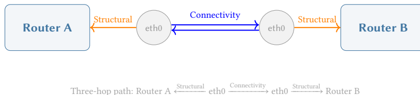
Figure 7. Connectivity edges between two devices. Each device connects via its Endpoint. A bidirectional link is stored as two explicit directed edges. The three-hop traversal path is shown below.
