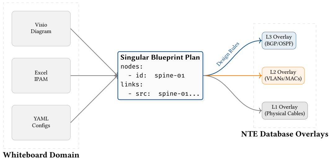
Figure 1. The W2P Strategy: Diverse whiteboard documents are aggregated into a singular formal Blueprint Plan, which the engine compiles and fans out into rigorous, multi-layered topology overlays.
