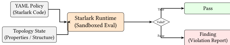
Figure 14. Starlark Policy Evaluation. The sandboxed runtime safely evaluates Python-like policy code against the topology state to generate deterministic compliance findings.
