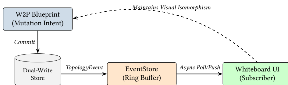
Figure 51. The Reactive Event Pipeline. Structural and relational changes are emitted as typed events, which bridge the physical storage layer back to the visual Blueprint domain.
