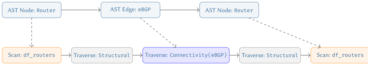
Figure 35. AST Compilation to Execution Plan. The semantic Cypher AST (top) is mathematically expanded by the Query Planner into a deterministic traversal plan (bottom) across the normalized Endpoints graph and partitioned DataFrames.
