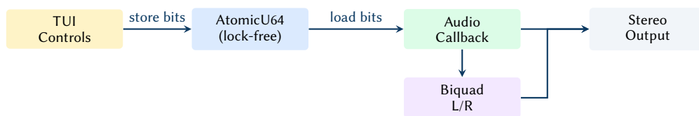
Figure 48. Lock-free live parameter path: the TUI stores f64 bit patterns into atomics; the audio callback loads them each block and updates the biquad filter only when thresholds are exceeded.
