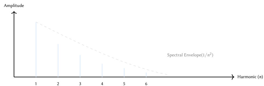
Figure 40. Additive synthesis model for the Shruti Box. The engine sums the first six harmonics of the tonic (Sa) and the fifth (Pa) with amplitudes decaying at a rate of 1/n^2 . A slow bellows-like amplitude LFO is applied to simulate the manual pumping of the instrument.
