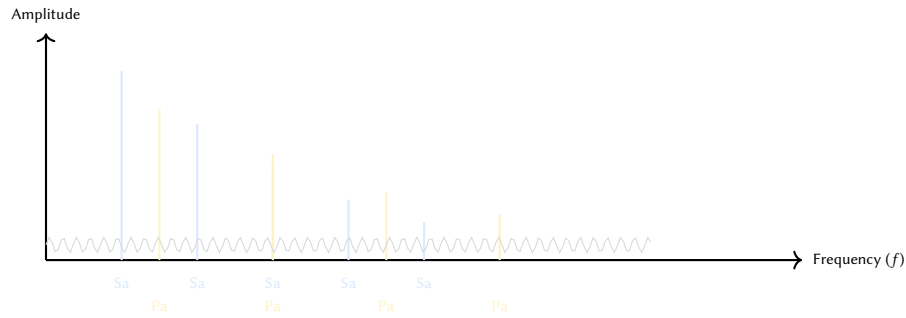
Figure 39. Harmonic spectrum of the Tanpura drone. The fundamental pitches (typically Sa and Pa) are accompanied by a dense series of upper partials that create a continuous, shimmering "bed" of sound. Overtone mimics this via multi-oscillator FM synthesis with slow phase modulations.
