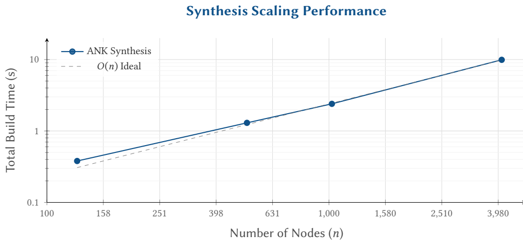
Figure 8. Synthesis Performance Metrics: ANK maintains linear complexity.
