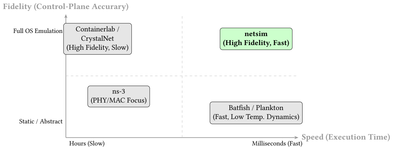
Figure 1. The Simulator Impedance Mismatch. netsim occupies the target quadrant for CI/CD pipelines: executing high-fidelity control-plane protocols (like OS emulation) but at deterministic, millisecond speeds (like static analysis).
