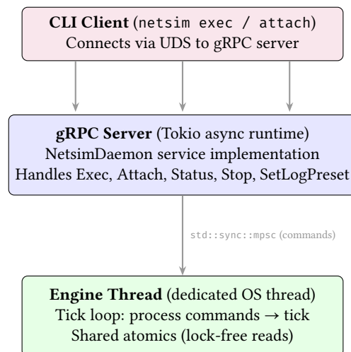
Figure 12. Daemon Concurrency Architecture. A Tokio-based gRPC server receives concurrent client connections and forwards commands to the strictly single-threaded Engine via channels.
