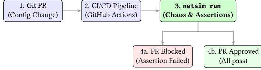
Figure 8. CI/CD Pipeline Integration. Declarative assertions allow netsim to automatically block PRs that would introduce routing loops or isolation, preventing operator-induced outages before deployment.
