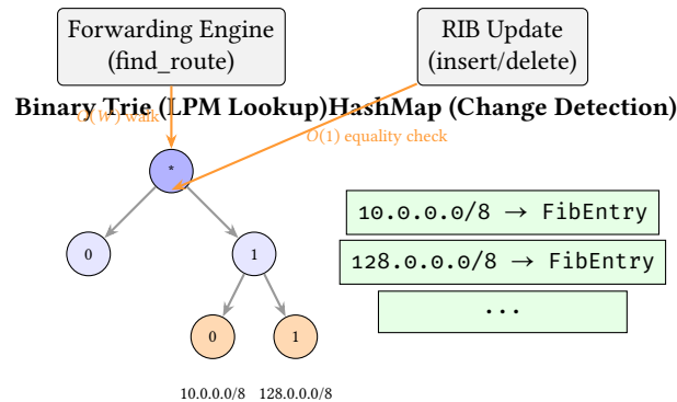
Figure 5. Dual-Index FIB Architecture. The Forwarding Engine uses the Binary Trie for fast Longest-Prefix-Match lookups, while RIB updates use the HashMap for O(1) exact-match change detection to avoid spurious convergence resets.
