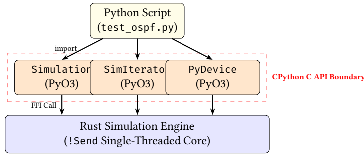
Figure 13. Python Bindings Architecture. The PyO3 wrappers expose the single-threaded Rust Engine directly to the Python interpreter, allowing zero-copy, in-process access to the simulation state.
