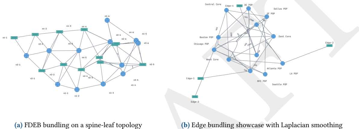
Figure 19. Force-directed edge bundling (FDEB) reduces visual clutter by grouping spatially compatible edges. Post-processing with Catmull-Rom splines and Laplacian smoothing produces clean, readable bundles.
