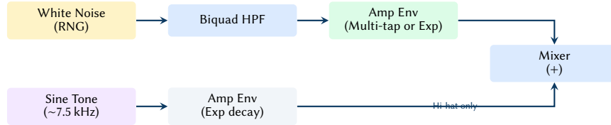
Figure 12. Percussion synthesis model. Hi-hats blend filtered noise with a metallic sine tone, while the clap relies entirely on a multi-tap noise envelope.
