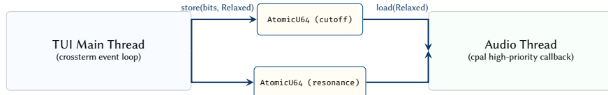
Figure 59. Lock-free concurrency model. The UI thread communicates with the real-time audio thread strictly through atomic variables, preventing priority inversion and guaranteeing that the audio callback never blocks waiting for a mutex.
