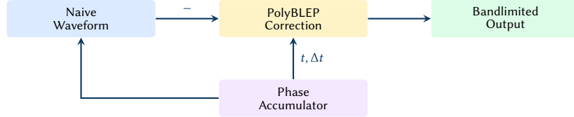
Figure 22. PolyBLEP anti-aliasing: the correction term is subtracted from the naive waveform at phase discontinuities.
