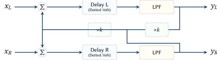
Figure 18. Ping-Pong Delay topology. Left and right channel inputs ( x_L, x_R ) are fed into independent delay lines. The output of each delay line is low-pass filtered (for analog-style damping), multiplied by the feedback coefficient k , and routed into the input sum of the opposite channel's delay line, creating a stereo bouncing effect.
