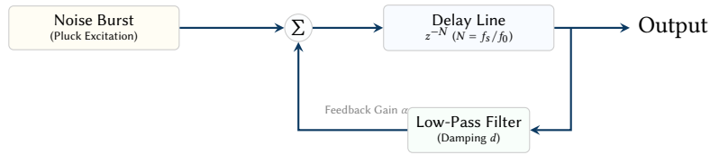
Figure 15. Karplus–Strong physical modeling architecture. A short burst of noise (the “pluck”) is fed into a delay line representing the string length. The output is fed back through a low-pass filter, causing higher frequencies to decay faster than fundamental frequencies, realistically simulating a plucked acoustic string.
