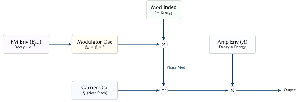
Figure 13. Two-operator FM Synthesis architecture. The modulator oscillator frequency ( f_m ) is a ratio ( R ) of the carrier pitch. The modulation depth (Index I ) is dynamically scaled by the macro energy level, meaning higher energy sections produce much brighter, richer sideband harmonics. The FM envelope ( E_{fm} ) creates a “pluck” or “wow” transient.
