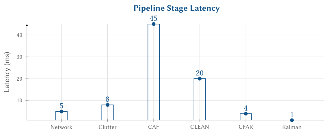
Figure 4. Real-time latency breakdown per beam (CIT = 100ms). The FFT-based CAF computation dominates processing time.
