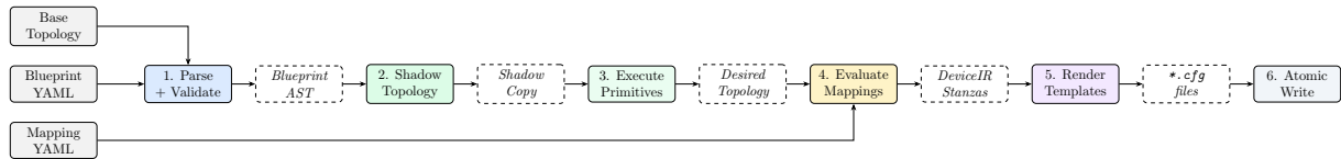
Figure 1: NetCfg compilation pipeline. Three inputs (base topology, blueprint, mapping) flow through six stages. The mapping document enters at stage 4, after primitive execution.
