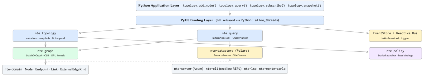
Figure 1: NTE system architecture. Solid arrows denote compile-time Rust crate dependencies; the dashed arrow indicates the runtime dual-write synchronisation path between nte-graph and nte-datastore .
