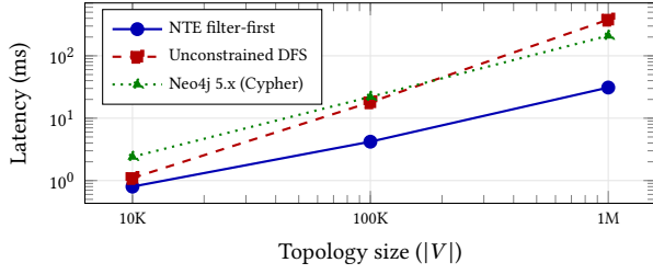
Figure 3: Median latency for a 2-hop property-filtered query (1% selectivity, \sigma = 0.01 ). NTE scales as O(\sigma n \cdot d) ; Neo4j’s row-oriented property store incurs a linear scan overhead.
