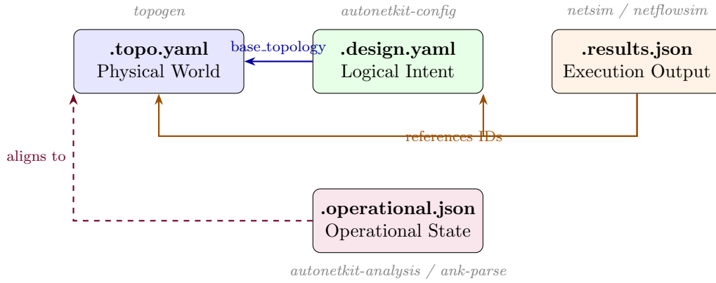
Figure 1: Sidecar file relationships. Solid arrows indicate direct references; dashed arrows indicate identity alignment.
