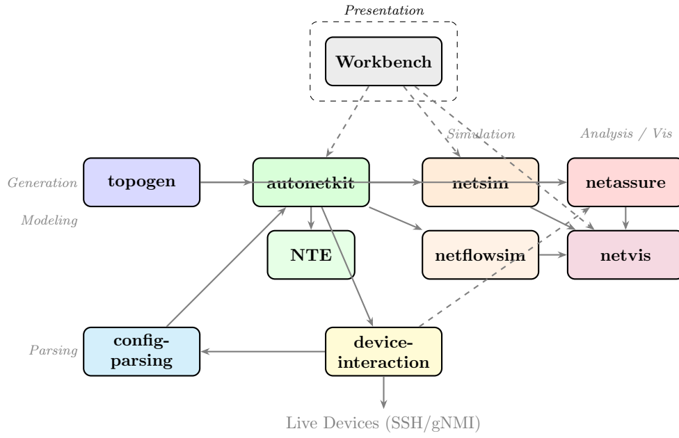
Figure 5: Ecosystem overview: ten tools in architectural layers with data flow arrows. Solid arrows are implemented; dashed arrows are planned.
