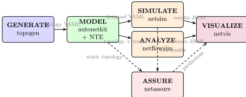
Figure 2: Data flow pipeline. Solid arrows are implemented; dashed arrows are planned or partially implemented.
