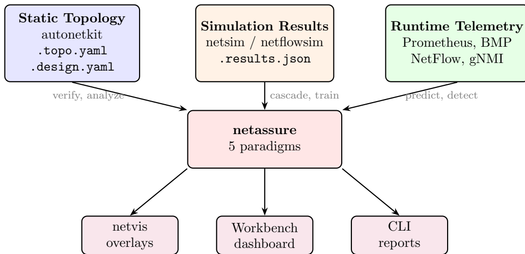
Figure 4: Multi-source analysis data flow: three data sources feed netassure, which produces insights for three consumer types.
