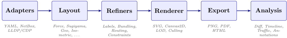
Figure 4: The NetVis six-layer pipeline.
