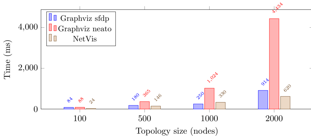
Figure 5: Comparative performance on identical spine-leaf topologies. NetVis includes the full pipeline (layout, labels, styling, SVG render); Graphviz includes layout and SVG output only. Apple M4 Pro, 24 GB RAM, best of 3 runs.
