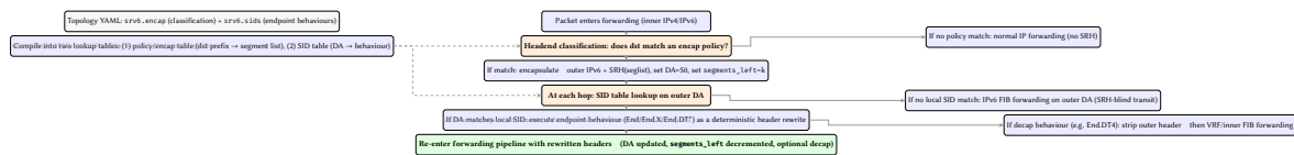
Figure 34. SRv6 Steering as a Two-Table Rewrite Pipeline. A headend policy classifies traffic and encapsulates it into an outer IPv6+SRH header; transit nodes interpret SRH only when the outer DA matches a local SID, executing endpoint behaviours as deterministic header rewrites that re-enter the normal forwarding pipeline.
