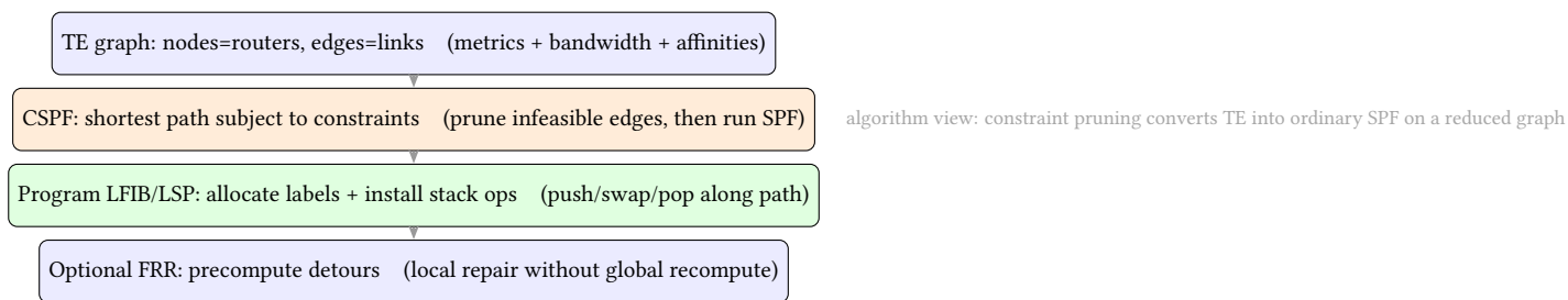
Figure 32. RSVP-TE as CSPF + Label Programming. Tunnel setup computes a constrained shortest path (CSPF) over the TE graph, then programs forwarding as deterministic label-stack rewrite operations along the chosen path.
