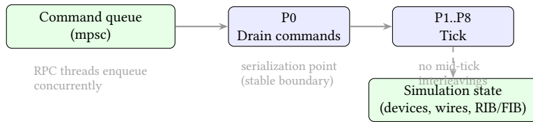
Figure 54. Commands as Tick-Boundary Transactions. External requests are concurrent, but their effects are serialized at P0. This prevents mid-tick observation of intermediate state and keeps the engine deterministic under interactive use.
