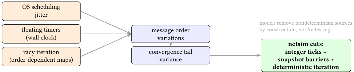
Figure 9. Determinism as Causal Cuts. Non-determinism in emulation typically arises from scheduling jitter, wall-clock timers, and order-dependent iteration. netsim removes these sources by construction (integer ticks, explicit snapshot/apply barriers, deterministic data structures), preventing message-order variation from propagating into convergence tail variance.
