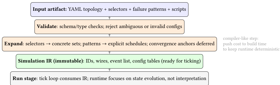
Figure 4. Build Stage as Compilation to an Immutable Simulation IR. The builder behaves like a compiler: it validates inputs, expands declarative constructs (selectors, failure patterns) into concrete sets and schedules, and emits an immutable intermediate representation consumed by the tick loop. This separation localizes complexity, makes errors early, and preserves determinism at runtime.
