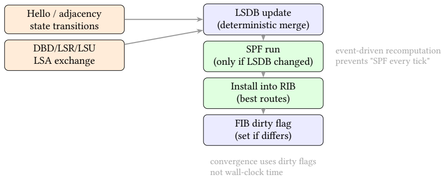
Figure 24. OSPF as Event-Driven Recomputation. Control-plane events (adjacency changes and LSA exchange) deterministically update the LSDB. SPF is triggered only when the LSDB changes, and route installation sets dirty flags only on real differences. This couples fidelity (RFC state machines) with performance (no unnecessary SPF) and with robust convergence detection (no false resets).
