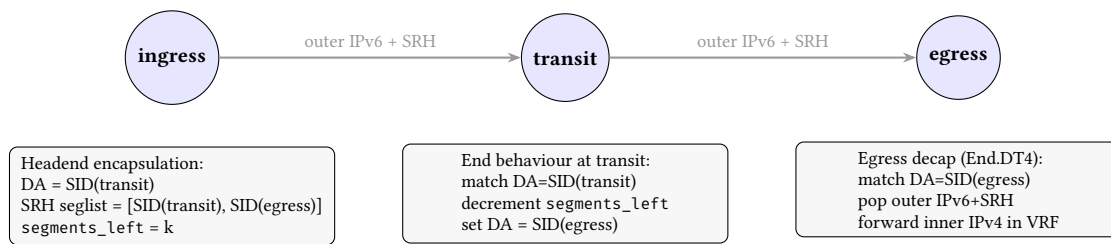
Figure 59. SRv6 Traffic Steering (Example 7) as a Deterministic DA Sequence. The ingress classifies and encapsulates traffic into an SRH segment list; the transit router executes End to advance to the next segment; the egress executes a decapsulation behaviour (End.DT4) to rejoin IPv4 forwarding.
