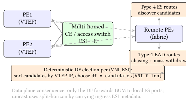
Figure 50. EVPN Multi-Homing as Deterministic Control/Data Coupling. Type-4 routes discover the candidate set for an Ethernet Segment (ESI). A deterministic DF election per VNI selects which PE forwards BUM to local ES ports, while split-horizon prevents loops by dropping frames that would hairpin back onto the same ESI.
