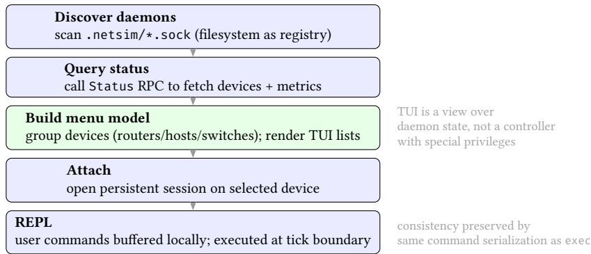
Figure 57. TUI Selector as a Discovery + View Pipeline. The filesystem provides a local daemon registry via UDS paths. The TUI builds a device selection model from Status and then enters attach/REPL mode without changing the underlying determinism guarantees.
