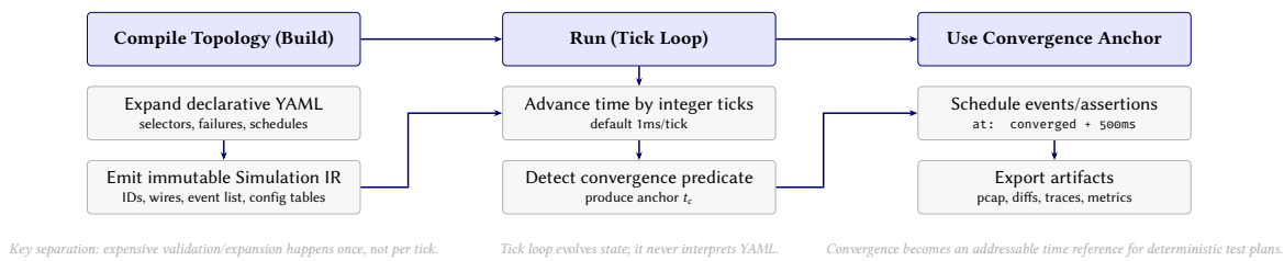
Figure 3. Convergence-first execution model. netsim behaves like a compiler: it first expands topology YAML into an immutable Simulation IR, then runs a deterministic tick loop to produce a named convergence time anchor t_c , which downstream schedules and assertions reference.
