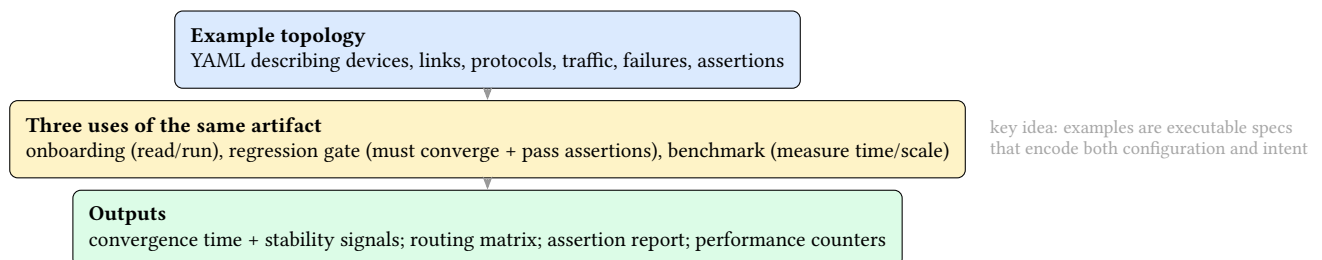
Figure 60. Examples as Executable Specifications. One topology artifact supports three workflows: learning, regression gating, and benchmarking. Determinism makes example outcomes (including time-to-stable) comparable across runs.
