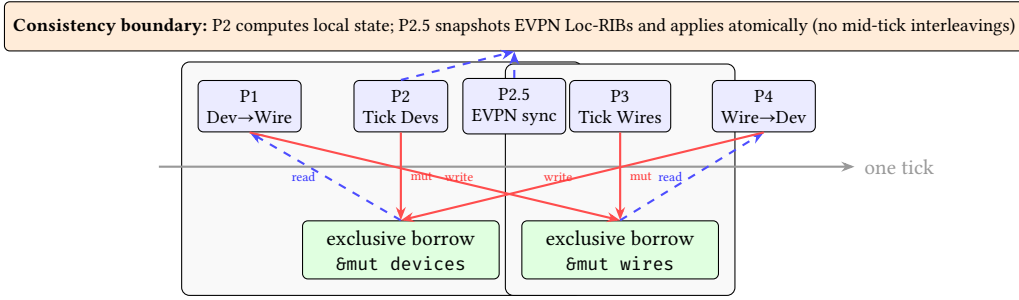
Figure 8. Borrow Windows and Consistency Boundaries. The engine alternates exclusive mutable access to devices and wires. Phases P1 and P4 form the synchronization boundary, while P2.5 introduces an explicit snapshot/apply barrier for EVPN to preserve determinism under parallel ticking.
