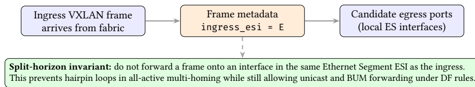
Figure 51. Split-Horizon as an Invariant. EVPN all-active multi-homing relies on explicit ESI metadata to prevent frames from being forwarded back onto the same Ethernet Segment, eliminating hairpin loops without requiring timing-dependent heuristics.
