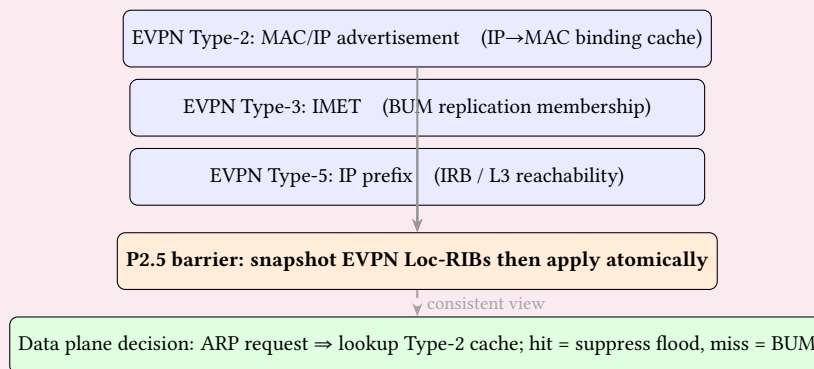
Figure 48. EVPN Control/Data Coupling via a Deterministic Barrier. Route types (2/3/5) update control-plane reachability. Phase P2.5 provides a snapshot/apply barrier so data-plane behavior (ARP suppression, BUM handling) reads a consistent EVPN cache, avoiding ordering-dependent mid-tick effects.
