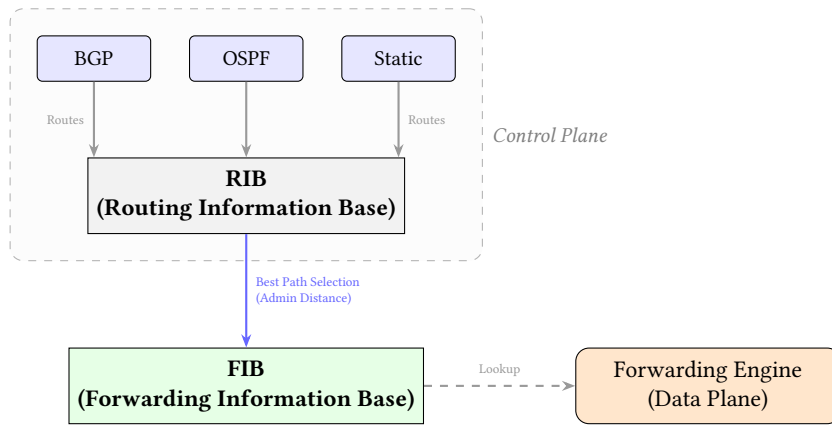
Figure 18. RIB/FIB Separation. Multiple routing protocols populate the global RIB. The router executes best-path selection based on Administrative Distance to program the active FIB used by the forwarding engine.
