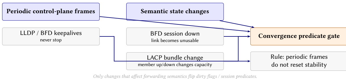
Figure 36. Periodic protocols vs convergence. netsim deliberately separates “packets keep flowing” (LLDP/BFD keepalives) from “routing state keeps changing” by excluding periodic keepalives from quiescence/convergence gates, while still treating semantic session transitions (e.g., BFD down) as immediate convergence-resetting events.
