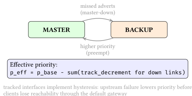
Figure 38. VRRP as an Election With Dynamic Priority. VRRP failover is driven by timeouts (missing advertisements) and by a deterministic priority function that can incorporate tracked uplink state. This view makes the key behavior explicit: gateway ownership moves when either timeouts fire or effective priority changes.
