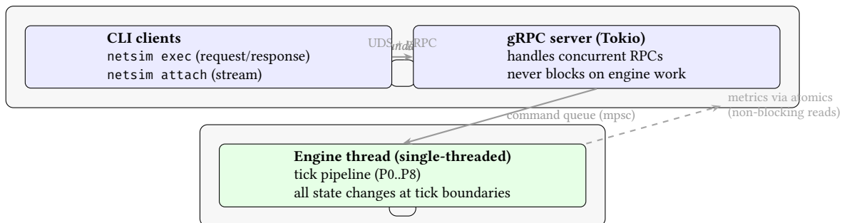
Figure 53. Daemon Architecture as a Consistency Boundary. Concurrency is handled at the RPC layer; determinism comes from funneling all mutations through a single-threaded tick loop. Commands serialize at tick boundary P0, producing a clear observable state model.
