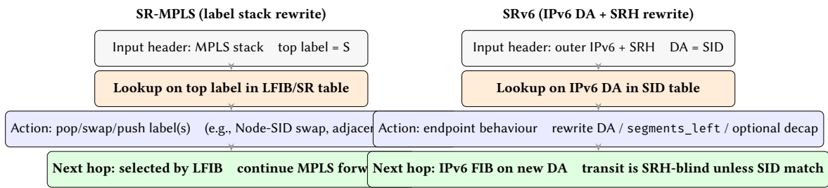
Figure 35. SR-MPLS vs SRv6 as the Same Rewrite Semantics. Both variants implement segment routing as repeated application of a hop function: look up the active segment identifier (top label vs IPv6 DA) and apply a local rewrite (label-stack ops vs SRH/DA update) before continuing normal forwarding.
