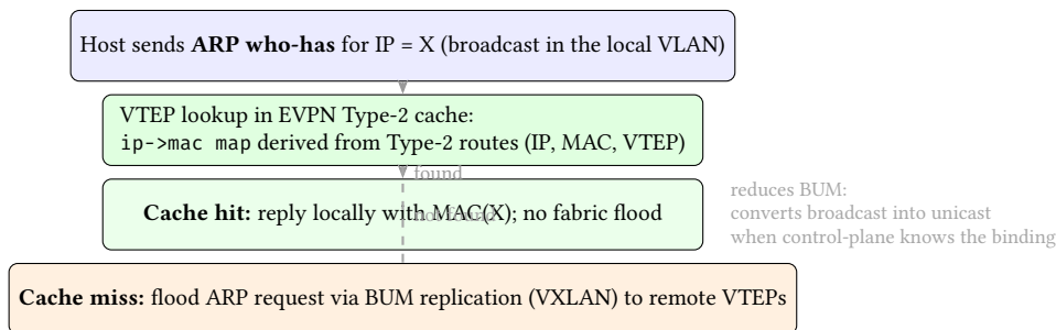
Figure 46. ARP Suppression as a Cache Lookup. EVPN Type-2 routes provide an IP→MAC binding cache at the VTEP. On an ARP request, a cache hit produces a local reply and avoids BUM flooding across the VXLAN fabric; cache misses fall back to normal flood semantics. This shows ARP suppression as an algorithmic optimization (lookup + conditional behavior) rather than a special-case protocol.
