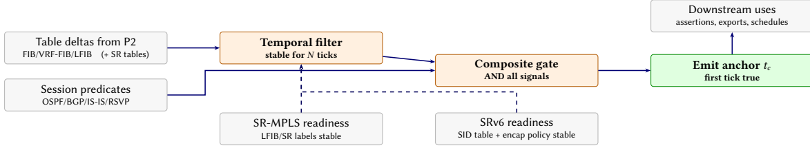
Figure 14. Where Segment Routing Fits in Convergence Gates. Segment routing adds forwarding-semantics tables: SR-MPLS expresses segments as label-stack rewrite rules (LFIB), while SRv6 expresses them as (encap policy, SID table) driving deterministic header rewrites. Their stability can be treated like other table-stability signals and included in the same N -tick temporal filter before the composite convergence predicate declares t_c .
