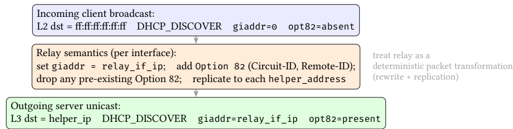
Figure 39. DHCP Relay as Packet-Transformation Semantics. The relay converts a local broadcast into one or more unicasts toward helper addresses, while rewriting giaddr and appending Option 82. Framing relay behavior as a deterministic rewrite rule makes it easy to reason about security (dropping untrusted Option 82) and about correctness across VRFs and L3 boundaries.
