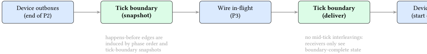
Figure 7. Determinism as a Happens-Before Graph. The tick loop induces an explicit partial order: device computations happen before wire advancement, which happens before delivery into inboxes. Tick-boundary snapshots act as synchronization points, preventing mid-tick observation and eliminating scheduling-dependent interleavings.
