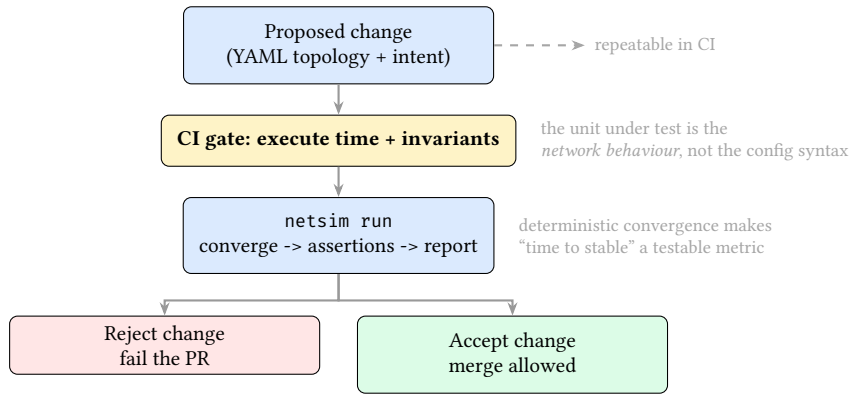
Figure 41. CI Integration as a Behavioural Gate. The topology file encodes both configuration and intent. CI runs netsim to convergence and evaluates assertions, turning routing safety (no loops, no isolation, bounded convergence time) into an automatic merge gate.
