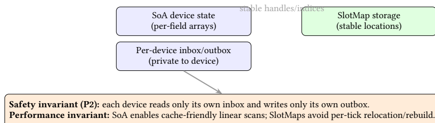
Figure 5. SoA + SlotMap as an Algorithmic Constraint. netsim stores per-device state in structure-of-arrays form and uses stable storage (SlotMaps) so device indices and references persist across ticks. This makes per-tick parallel evaluation ( Rayon par_iter_mut ) safe (no aliasing across devices) and fast (cache-friendly scans), while keeping the tick loop free of object reconstruction overhead.
