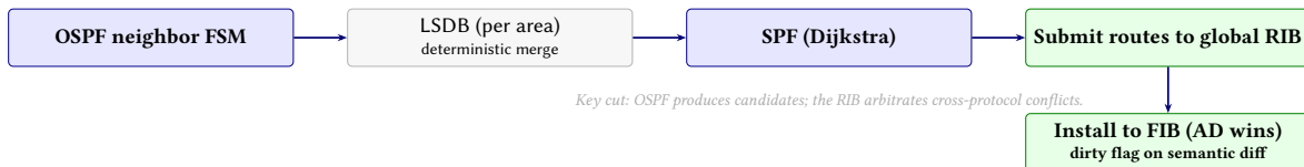
Figure 25. OSPF in the global routing pipeline. OSPF maintains adjacency state and the LSDB, runs SPF only when the LSDB changes, and submits candidate routes into the global RIB. Final forwarding state is installed into the FIB by administrative-distance arbitration, and convergence is driven by semantic diffs (dirty flags), not by timer expiry.
