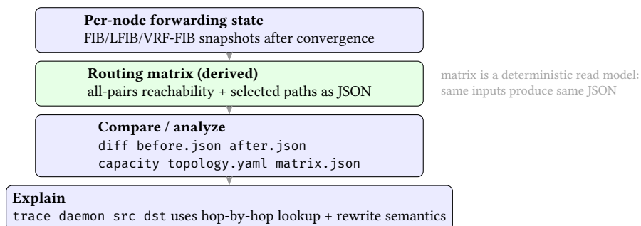
Figure 52. Routing Matrix as a Derived Artifact. Many analysis commands operate on a deterministic, post-convergence snapshot of forwarding state that is exported as a routing matrix. This makes diffs and capacity analysis meaningful and repeatable.
