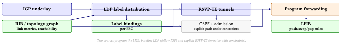
Figure 31. MPLS control-plane to data-plane pipeline. IGP builds the underlay graph, LDP produces label bindings for FECs, and RSVP-TE computes explicit constrained paths. Both feed a single LFIB programming step that installs the label-stack rewrite rules used by forwarding.
