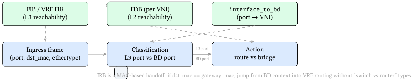
Figure 43. Unified L2/L3 Router as a Conceptual Model. Rather than branching on device type, the data plane classifies each ingress by port-to-bridge-domain membership and then selects an action (route via FIB/VRF or bridge via per-VNI FDB). IRB is a deterministic MAC-based handoff from L2 to L3.
