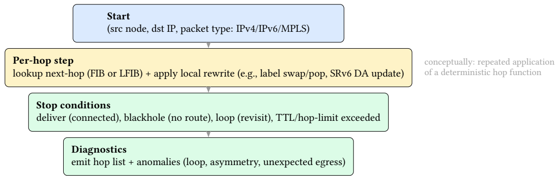
Figure 10. Path Trace as a Hop Function with Rewrite Semantics. Tracing is not a separate simulator mode: it repeatedly applies the same per-hop forwarding semantics (lookup + rewrite) and reports clear termination and anomaly conditions.
