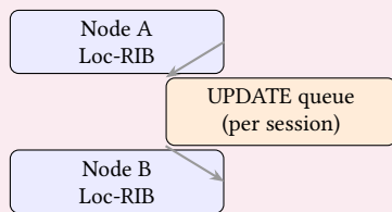
Figure 47. EVPN Synchronisation as a Consistency Model. Per-message queuing exposes the simulation to ordering-dependent behaviour. netsim instead snapshots all EVPN Loc-RIBs once per tick (Phase P2.5) and applies the same snapshot everywhere, providing a deterministic barrier that preserves “simultaneous” control-plane state replication.
