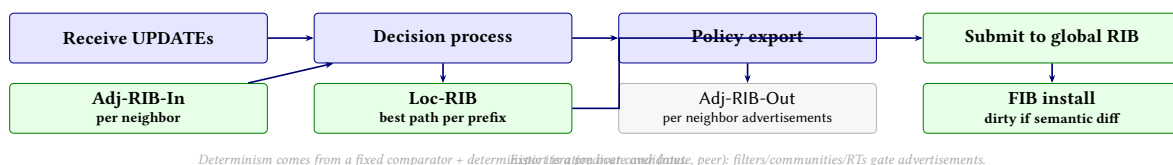
Figure 28. BGP as a dataflow pipeline. Updates enter Adj-RIB-In, a deterministic decision process produces the Loc-RIB, and export policy decides what each peer sees (Adj-RIB-Out). Loc-RIB winners are submitted to the global RIB for administrative-distance arbitration and FIB installation.
