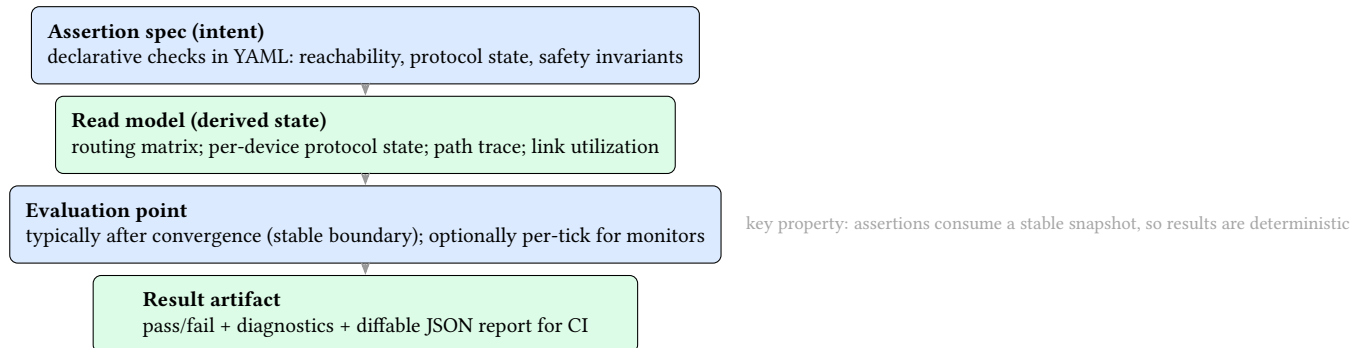
Figure 40. Assertions as Properties Over a Read Model. Assertions encode intent, but they are evaluated over derived, snapshot-stable artifacts (routing matrix, protocol state) at a well-defined point in time, producing CI-friendly, diffable results.
