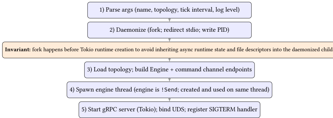
Figure 56. Daemon Startup as an Ordered Initialization with Invariants. The sequence is designed to preserve deterministic engine ownership (!Send) while providing async RPC service, and to keep OS-level process semantics (fork + fd handling) from contaminating runtime state.
