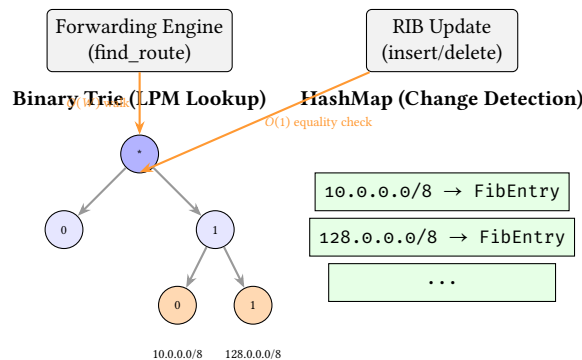
Figure 20. Dual-Index FIB Architecture. The Forwarding Engine uses the Binary Trie for fast Longest-Prefix-Match lookups, while RIB updates use the HashMap for O(1) exact-match change detection to avoid spurious convergence resets.
