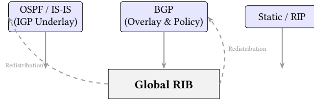
Figure 23. Control Plane Protocol Interactions. Protocols independently compute routes and submit them to the Global RIB, which arbitrates conflicts using administrative distance. The RIB can also redistribute routes back into protocols.
