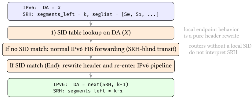
Figure 33. SRv6 Packet Walk as a Header-Rewrite Semantics. A local SID match triggers endpoint behavior that deterministically rewrites (DA, segments_left ) and loops back into the IPv6 forwarding pipeline. Routers without a matching local SID forward on the outer DA only.
