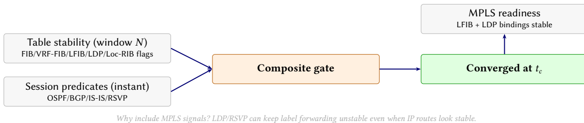
Figure 62. Where MPLS/RSVP gates enter convergence. Convergence is not just IP FIB stability: LFIB and label bindings are part of the same fixed point, so the convergence predicate includes both table-stability windows and session-state checks.
