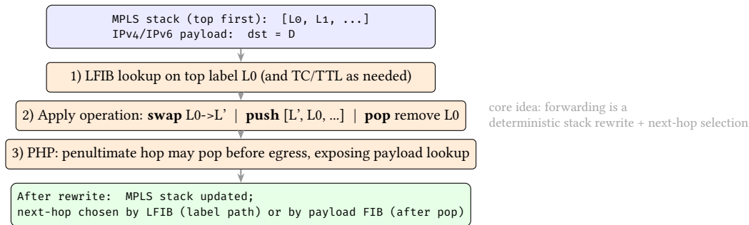
Figure 30. MPLS Forwarding as Label-Stack Rewrite Semantics. The data plane selects an LFIB entry by the top label and then applies a local rewrite (push/swap/pop). PHP is a controlled pop that exposes the payload for final FIB lookup.
