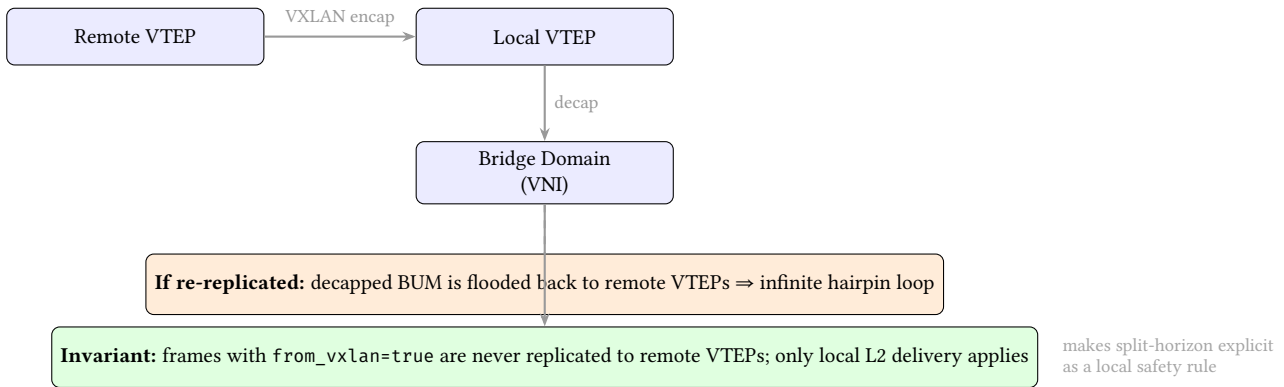
Figure 44. VXLAN Hairpin Prevention as an Invariant. The from_vxlan=true flag marks decapsulated frames so that the local VTEP applies a strict split-horizon rule: do not replicate back onto the VXLAN fabric. This prevents infinite BUM loops without relying on timing or message ordering, aligning with netsim’s determinism goals.
