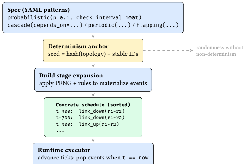
Figure 42. Chaos Scheduling as Deterministic Expansion. The input is a declarative pattern spec; the output is a concrete, stably-ordered event list. A seeded PRNG provides randomized scenarios while preserving exact replayability across runs.
