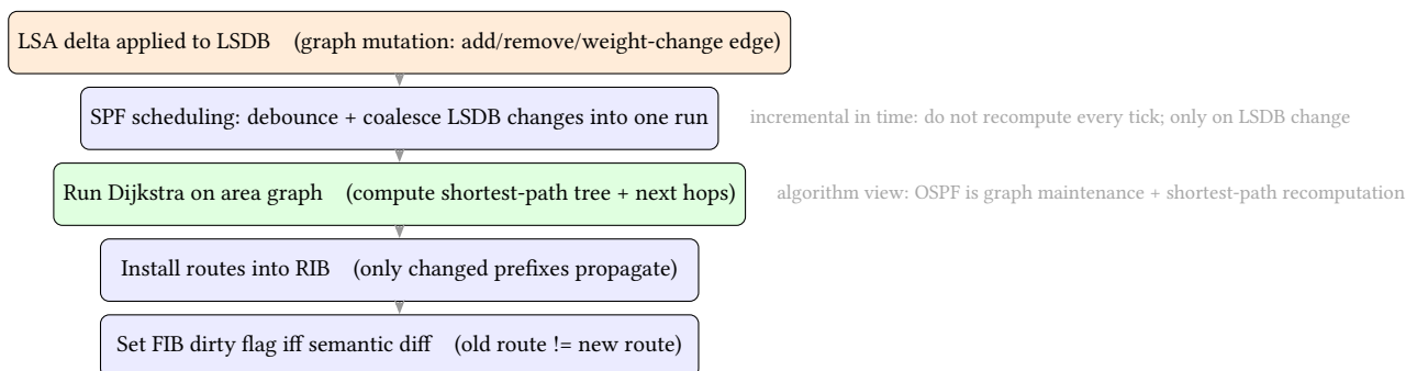
Figure 26. OSPF SPF as Graph Recompute on LSDB Deltas. An LSDB change mutates the area graph. netsim coalesces changes and runs Dijkstra only when needed, then installs only semantically changed routes into the RIB/FIB pipeline (dirty flags flip only on real diffs).
