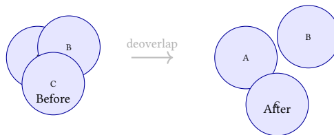
Figure 47. DeoverlapRefiner: applies a repulsive spring force between overlapping node bounding boxes, pushing them apart until the configured minimum margin is satisfied.
