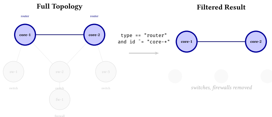
Figure 57. Filter DSL in action. The expression type == "router" and id ~= "core-* matches only the two core routers (highlighted). All non-matching nodes and their incident edges are removed from the rendered output. The filter supports boolean operators, attribute comparisons, and glob patterns.
