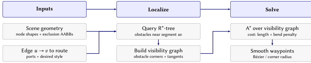
Figure 44. SmartRoutingRefiner as a three-step algorithm: (1) local obstacle selection via an R*-tree query, (2) visibility-graph construction over obstacle features, (3) shortest-path search (A*) followed by spline smoothing. This separates correctness (obstacle avoidance) from aesthetics (curve shape).
