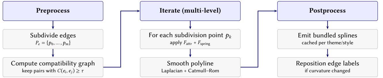
Figure 41. Bundling as a pipeline: compatibility graph construction gates which edges interact; the iterative solver updates only subdivision points; smoothing converts a polyline into a visually stable spline.
