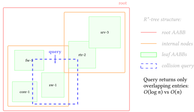
Figure 39. R*-tree spatial index for label collision detection. Occupied regions (node shapes, existing labels, edge exclusion zones) are inserted as axis-aligned bounding boxes. A candidate label position is tested by querying the tree for intersections— O(\log n) per query vs. O(n) brute force.
