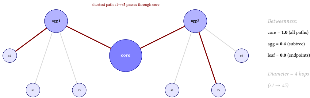
Figure 56. Graph analytics: betweenness centrality visualized. Node size encodes centrality—the core router sits on every shortest path between the two subtrees (centrality 1.0), making it the critical transit point. Aggregation nodes score 0.4 (bridging their subtrees); leaf nodes score 0.0. Graph diameter (longest shortest path) is 4 hops.
