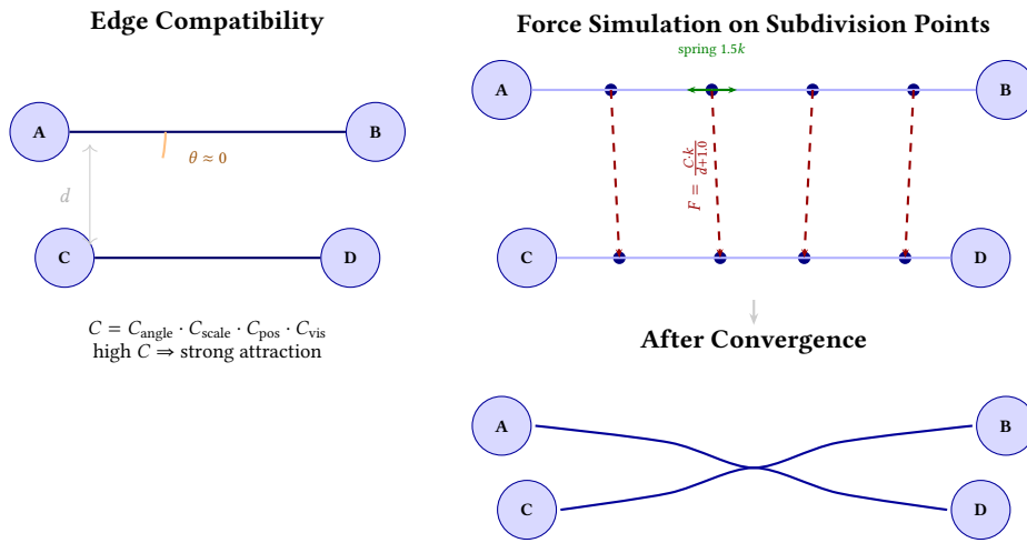
Figure 42. FDEB force-directed edge bundling. Top left: edge compatibility scoring—nearly parallel, co-located edges receive high compatibility C . Top right: subdivision points along each edge are subject to attraction forces (red, F = Ck/(d+1) ) toward corresponding points on compatible edges, and spring forces (green, 1.5k ) that preserve edge shape. Bottom: after convergence, compatible edges merge into a shared bundle through the midpoint, fanning out to their respective endpoints.
