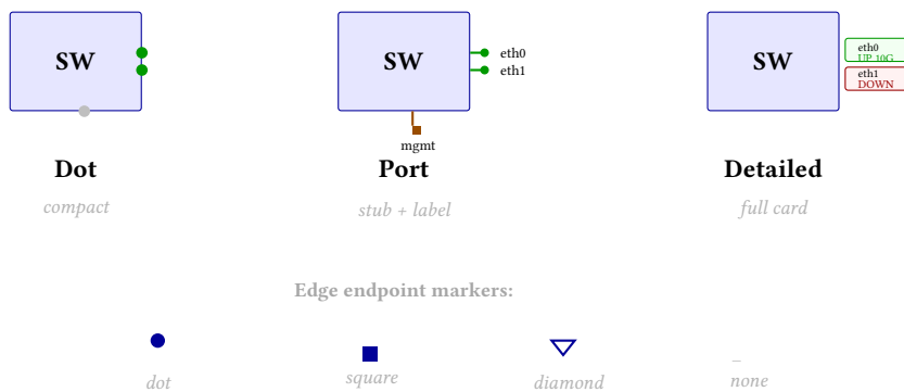
Figure 32. Interface rendering modes. Dot: compact circles on the node boundary. Port: rectangular stubs with labels. Detailed: full interface cards with status and speed. Four marker types control the edge endpoint symbol.
