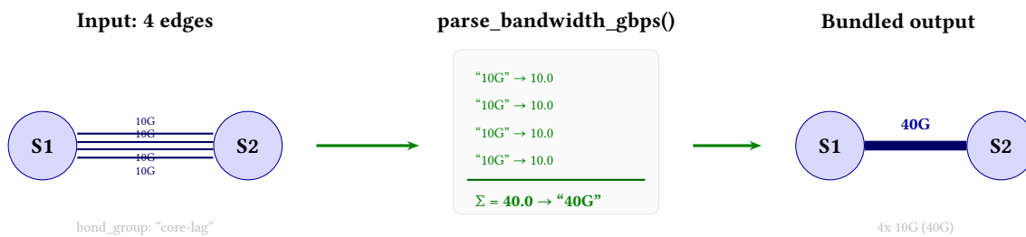
Figure 29. Automatic bandwidth aggregation. Four edges sharing bond_group : “core-lag” have their bandwidth labels parsed by parse_bandwidth_gbps() , which recognizes SI suffixes (M/G/T). The totals are summed and formatted: Bundled mode shows only “40G”; other modes show “4x 10G (40G)”.
