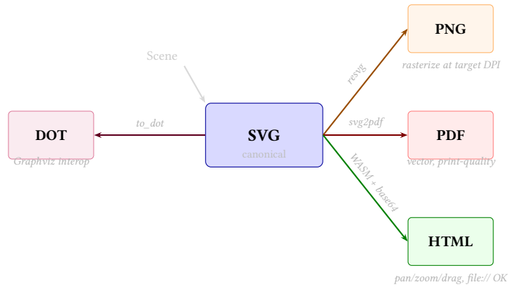
Figure 63. Export format pipeline. SVG is the canonical intermediate representation. resvg rasterizes to PNG at configurable DPI; svg2pdf produces vector PDF for print; the HTML exporter embeds WASM as base64 for interactive pan/zoom/drag openable from file:// ; DOT export enables Graphviz interoperability.
