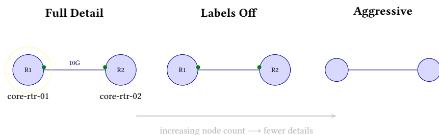
Figure 62. Level of detail (LOD) progressive suppression. As topology size grows past profile thresholds, labels, edge labels, interface markers, and visual effects are progressively hidden to maintain render performance and visual clarity.
