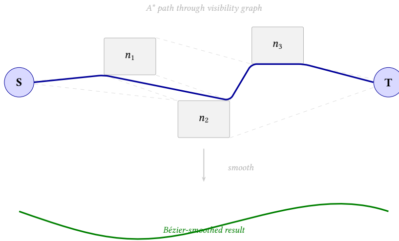
Figure 45. SmartRoutingRefiner. An R*-tree query identifies obstacles near each edge. A visibility graph connects obstacle corners; A* finds the shortest obstacle-free path. Waypoints are smoothed to Bézier splines for natural-looking curves.
