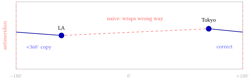
Figure 19. Antimeridian wrapping. An edge from Tokyo to Los Angeles naively crosses the full map width (red dashed). NetVis detects the projected discontinuity ( >150 px jump) and renders two segments: one exiting at +180^\circ and a 360^\circ -shifted copy entering at -180^\circ .
