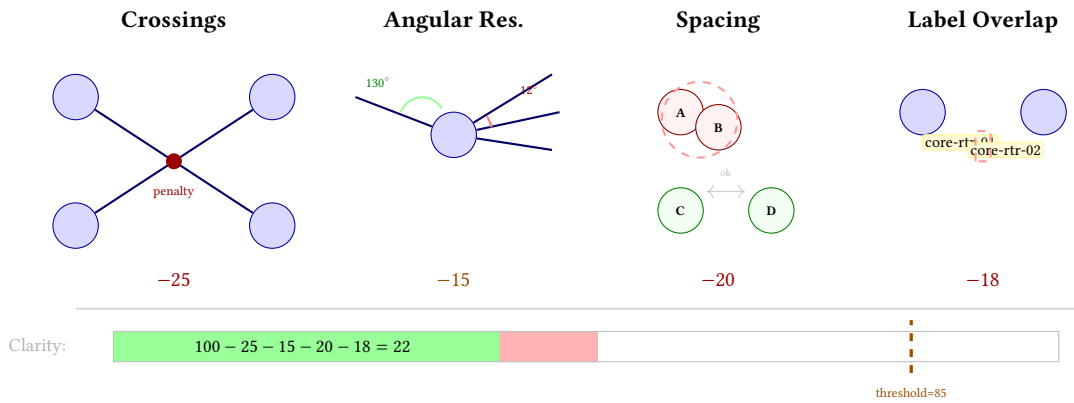
Figure 59. Clarity score: four quality factors illustrated spatially. Each panel shows the visual defect and its penalty. Edge crossings, narrow angular resolution, overlapping nodes, and colliding labels all subtract from 100. CI/CD pipelines gate on a configurable threshold (default: 85; this example scores 22—a clear failure).
