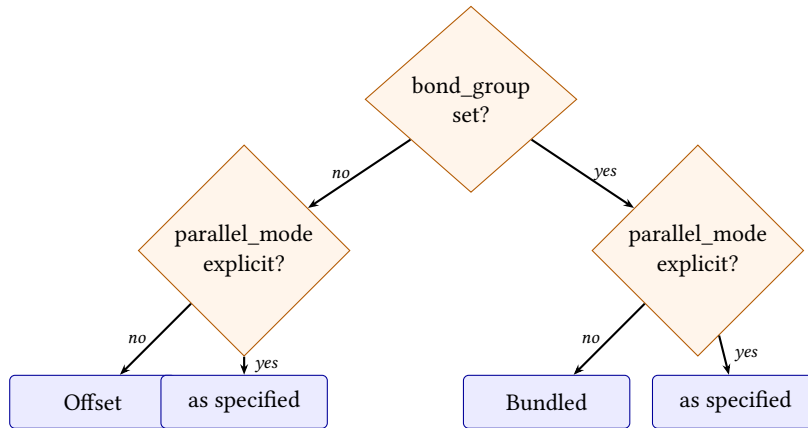
Figure 28. Parallel edge mode selection logic. Bond groups default to Bundled; non-bonded parallel edges default to Offset. An explicit parallel_mode always overrides the default.
