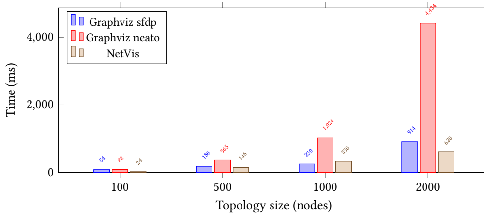
Figure 67. Comparative performance on identical spine-leaf topologies. NetVis includes the full pipeline (layout, labels, styling, SVG render); Graphviz includes layout and SVG output only.
