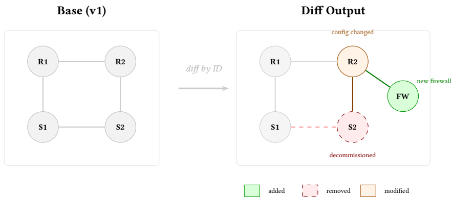
Figure 49. Topology diffing by example. The base topology (v1) is compared to a new version by matching node and edge IDs. The diff output color-codes changes: S2 was decommissioned (red/dashed), R2's config changed (amber), and a new firewall was added (green). Unchanged elements remain gray.
