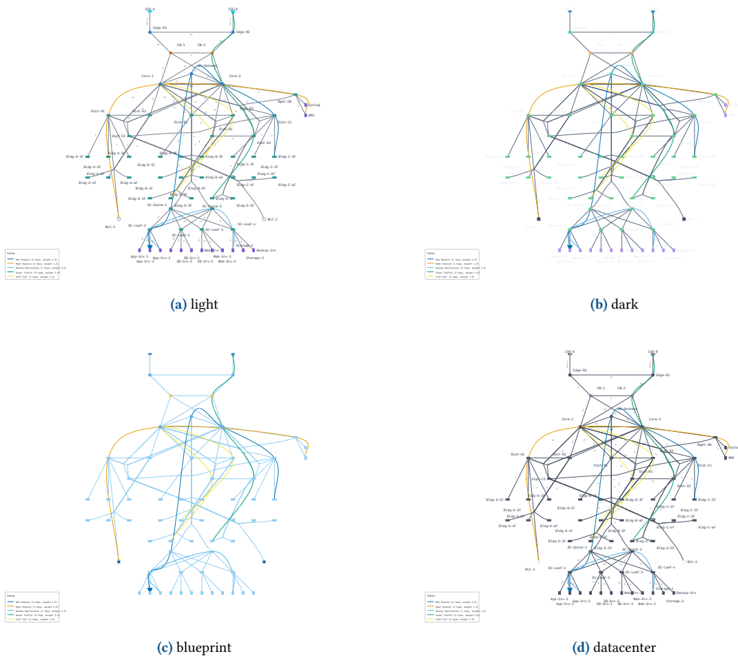
Figure 26. Enterprise campus (72 nodes, 98 edges) in four themes. Each theme adapts node icons, edge colors, label styling, background, glow intensity, and shadow direction. Only the theme: field changes in the YAML.
