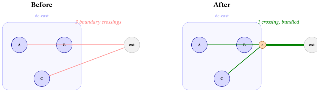
Figure 48. BoundaryBundlingRefiner. Before: three edges from internal nodes to an external node each cross the group boundary independently. After: all edges fan into a shared crossing point on the boundary and exit as a single bundled edge, reducing visual clutter at group borders.
