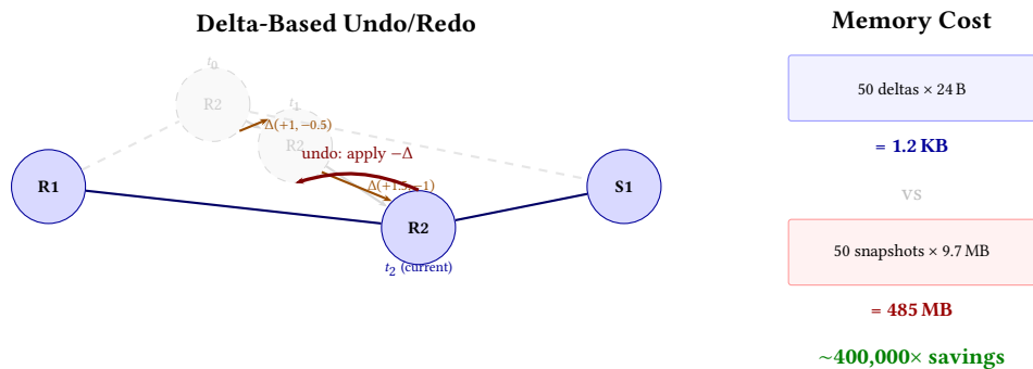
Figure 53. Interactive editor with spatial undo. Node R2 is dragged through three positions; each move stores only a delta ( \Delta x, \Delta y , 24 bytes) rather than a full scene snapshot. Undo applies -\Delta to restore the previous position. At 5,000 nodes the delta approach uses 1.2 KB vs. 485 MB for snapshot-based undo.
