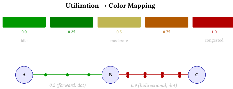
Figure 51. Traffic flow animation. Edge utilization (0.0–1.0) maps to a green–amber–red color ramp. Animated dots travel along the edge path; bidirectional mode shows two opposing dot streams. CSS @keyframes drives the animation in SVG output.
