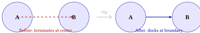
Figure 46. EdgeClippingRefiner: without clipping, edge paths terminate at node centers; with clipping, endpoints dock at the exact node shape boundary, giving correct arrowhead placement regardless of shape.
