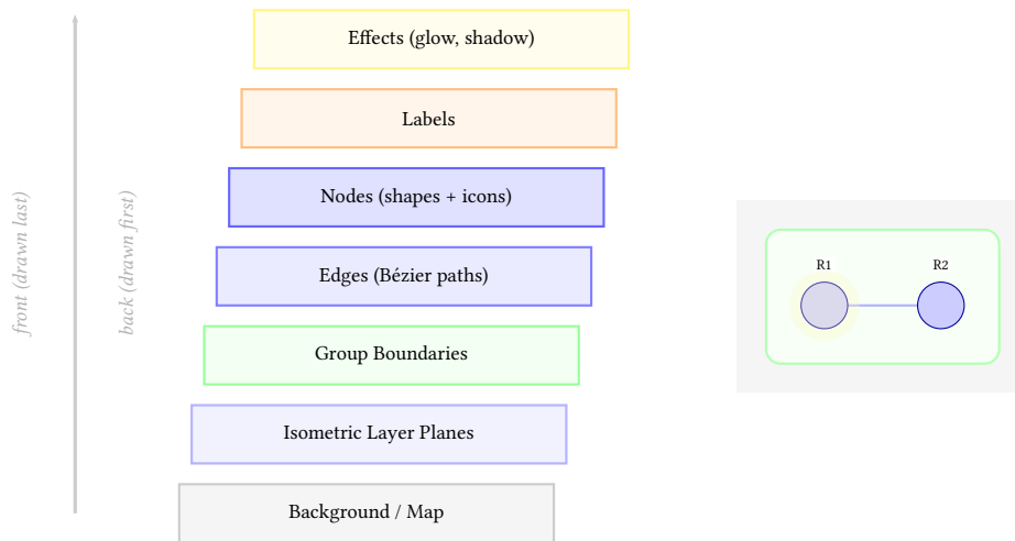
Figure 61. SVG rendering layer order (painter’s model). Elements are drawn back-to-front: background first, effects last. This ensures labels are always readable over edges, nodes always cover edge strokes at endpoints, and effect overlays (glow, shadow) render above all content.
