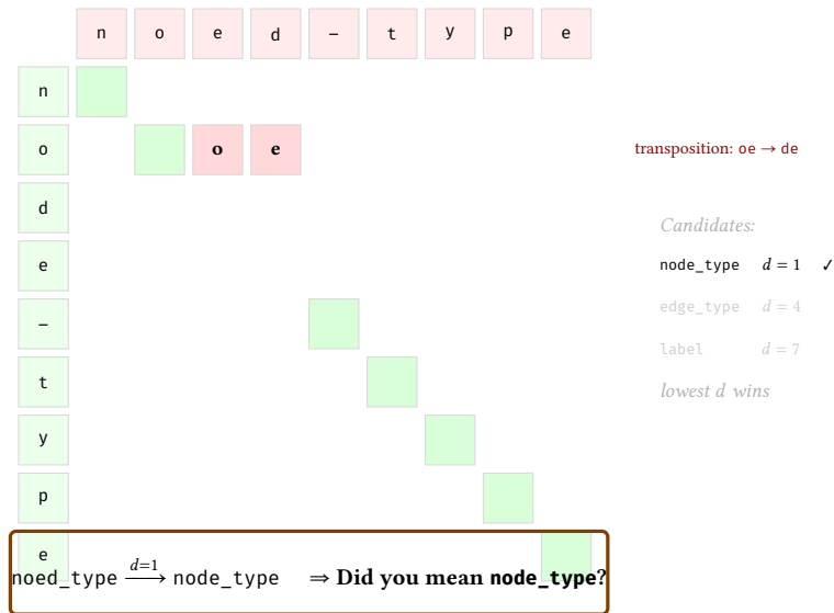
Figure 58. Fuzzy validation with Levenshtein distance. The misspelled field noed_type is compared against all valid schema fields. Character-level alignment reveals a single transposition ( oe → de ), yielding distance d = 1 . The closest match ( node_type ) is suggested as a correction.
