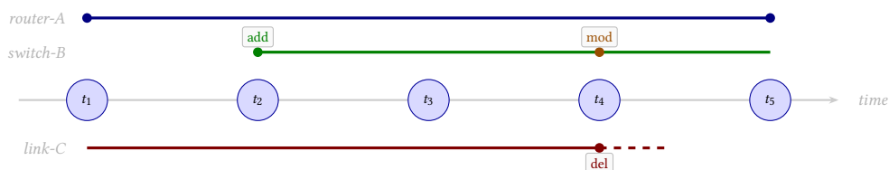
Figure 50. Temporal analysis: entity lifecycle tracking across topology snapshots. Each snapshot ( t_1 – t_5 ) is a YAML file. The timeline module traces first appearance (add), attribute changes (mod), and removal (del) for every node and edge.
