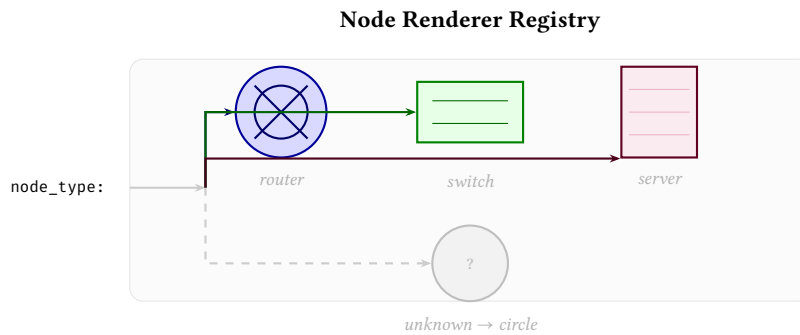
Figure 64. Pluggable node renderer dispatch. The render::registry module maps node_type strings to shape renderers. Built-in types ( router , switch , server , firewall , cloud , l3_switch ) are registered at startup. Unknown types fall back to the default circle renderer, ensuring graceful degradation for unrecognized device types.
