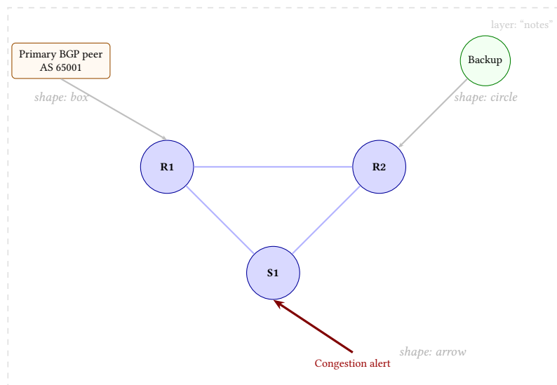
Figure 52. Annotation callout shapes. Each annotation anchors to a node with a pointer line. Three shapes are supported: box (rectangular, for multi-line text), circle (compact labels), and arrow (directional emphasis). Annotations are organized into named layers for selective visibility.
