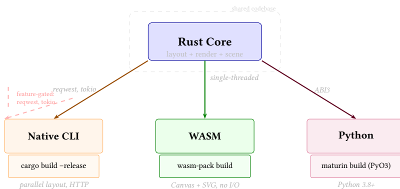
Figure 65. Deployment architecture. A single Rust codebase compiles to three targets via feature flags. WASM-incompatible crates (reqwest, tokio) are gated to native-only. The Python binding uses PyO3 with ABI3 stability for broad version support.
