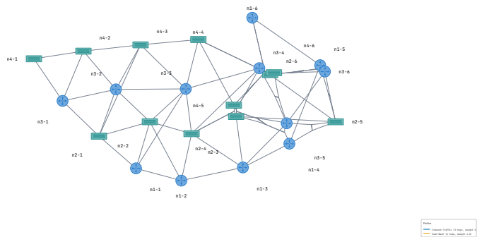
(a) FDEB on a spine-leaf topology
