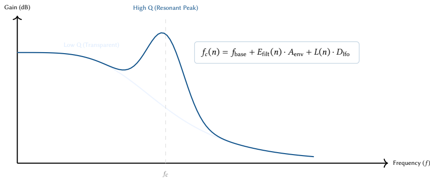
Figure 17. Filter response geometries and modulation sources. The "Acid" character is achieved by a sharp resonant peak at the cutoff frequency ( f_c ). This frequency is dynamically modulated per-sample by the filter envelope and LFO.
