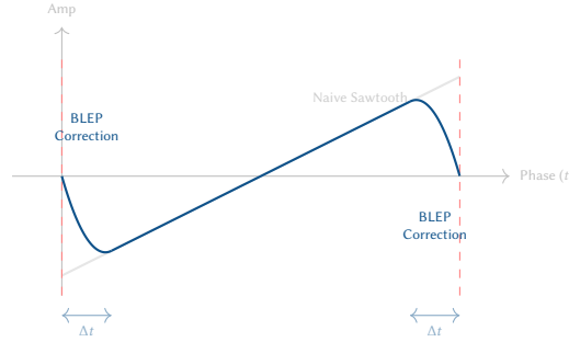
Figure 31. PolyBLEP discontinuity correction. The "naive" sawtooth waveform has an infinite slope at the wrap-around point, which creates aliases across the entire frequency spectrum. The PolyBLEP algorithm subtracts a bandlimited residual (the BLEP) within one sample period ( \Delta t ) of the discontinuity, effectively smoothing the edge and suppressing digital artifacts.
