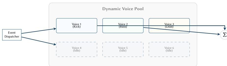
Figure 85. Dynamic voice pool management. The engine maintains a pool of pre-allocated DSP voices. When an event is dispatched, an idle voice is activated and assigned a synthesis model. Once the amplitude envelope reaches silence, the voice returns to the idle state, minimizing real-time allocations.
