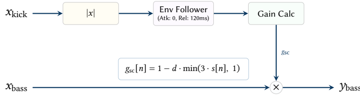
Figure 26. Sidechain compression signal flow. The absolute value of the kick signal drives an envelope follower with instantaneous attack and exponential release. This envelope calculates a dynamic gain reduction ( g_{sc} ) which is multiplied against the bass signal, ducking it to create rhythmic pumping.
