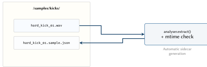
Figure 37. Sidecar caching strategy. For every WAV file in the library, Overtone generates a lightweight JSON metadata file. This prevents expensive FFT re-analysis during application startup, while the modification-time check ensures the cache remains synchronised with the source audio.
