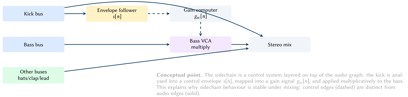
Figure 24. Sidechain compression as a control graph. Dashed arrows carry control signals; solid arrows carry audio. This framing clarifies how the kick shapes bass dynamics without being mixed into the control path.
