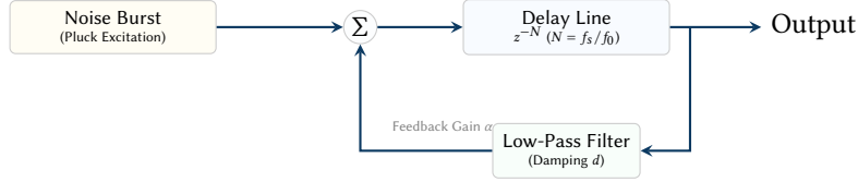
Figure 22. Karplus-Strong physical modeling architecture. A short burst of noise (the "pluck") is fed into a delay line representing the string length. The output is fed back through a low-pass filter, causing higher frequencies to decay faster than fundamental frequencies, realistically simulating a plucked acoustic string.
