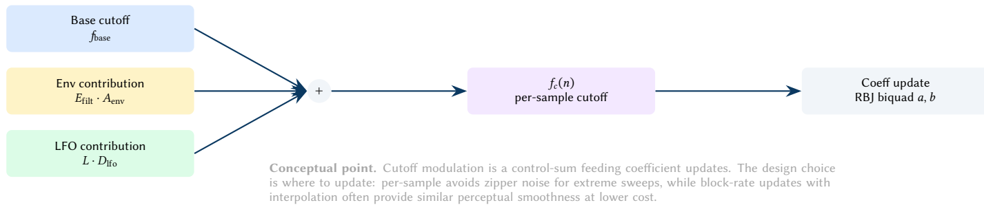
Figure 18. Filter modulation as a control-sum graph. Multiple modulation sources sum into f_c(n) , which drives coefficient updates and then sample processing.
