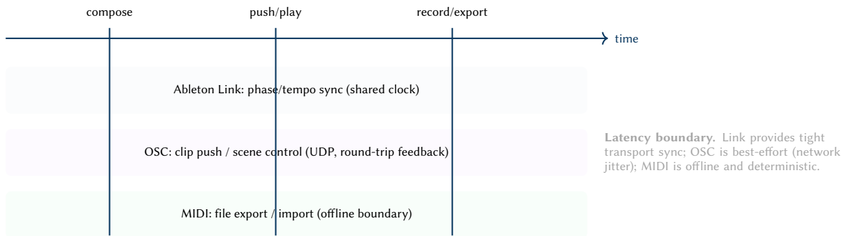
Figure 77. Timing and latency boundaries in Ableton integration. Link synchronises transport phase, OSC provides interactive control with network jitter, and MIDI provides an offline deterministic interchange format.
