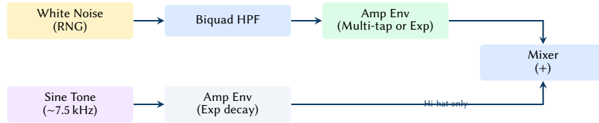
Figure 19. Percussion synthesis model. Hi-hats blend filtered noise with a metallic sine tone, while the clap relies entirely on a multi-tap noise envelope.
