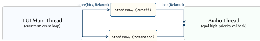
Figure 91. Lock-free concurrency model. The UI thread communicates with the real-time audio thread strictly through atomic variables, preventing priority inversion and guaranteeing that the audio callback never blocks waiting for a mutex.
