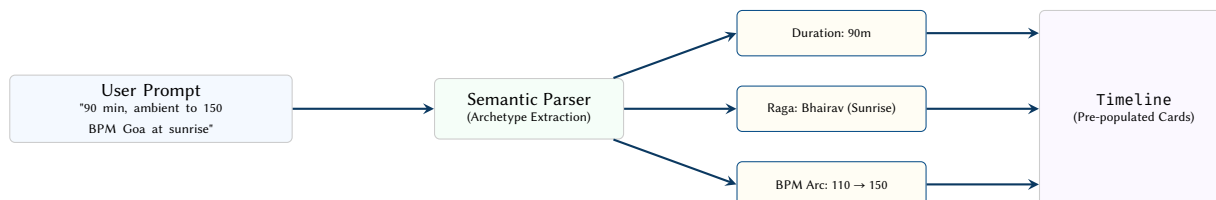
Figure 96. The Oracle Prompt workflow. Natural language is parsed into structural parameters (duration, raga mapping, tempo curves) to algorithmically pre-populate the timeline with thematic cards.
