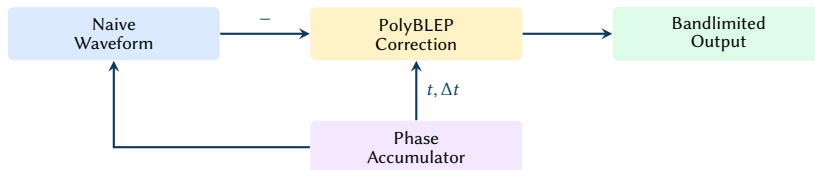
Figure 32. PolyBLEP anti-aliasing: the correction term is subtracted from the naive waveform at phase discontinuities.
