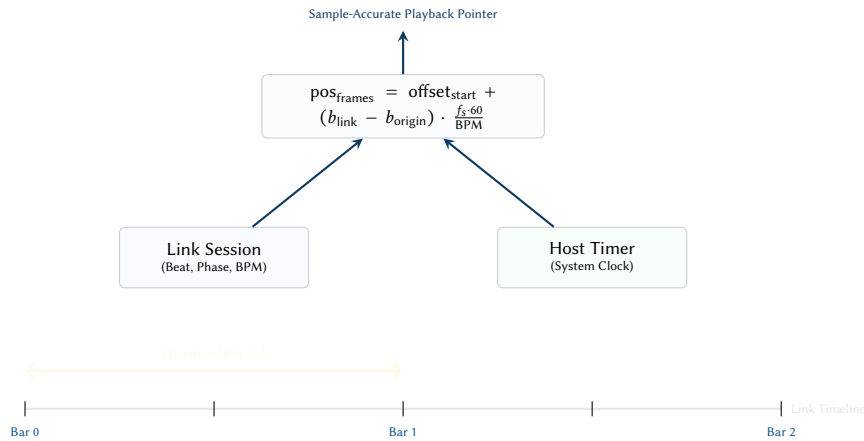
Figure 81. Ableton Link phase-locked synchronisation. The engine maps the shared Link timeline (beats) to local audio buffers using the system’s high-precision timer. Playback is quantized to 4-beat boundaries, ensuring that Overtone’s kick drum aligns perfectly with external peers.
