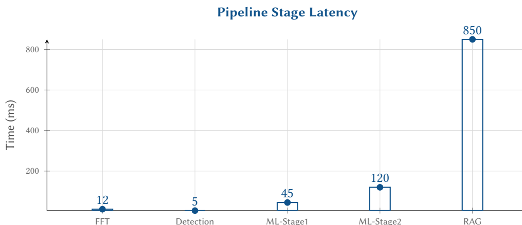
Figure 12. Spectra Pipeline Latency: RAG-based synthesis is the primary bottleneck.
