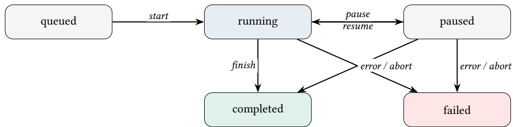
Figure 2. MissionRun state machine used by the autonomy scheduler and clients.
