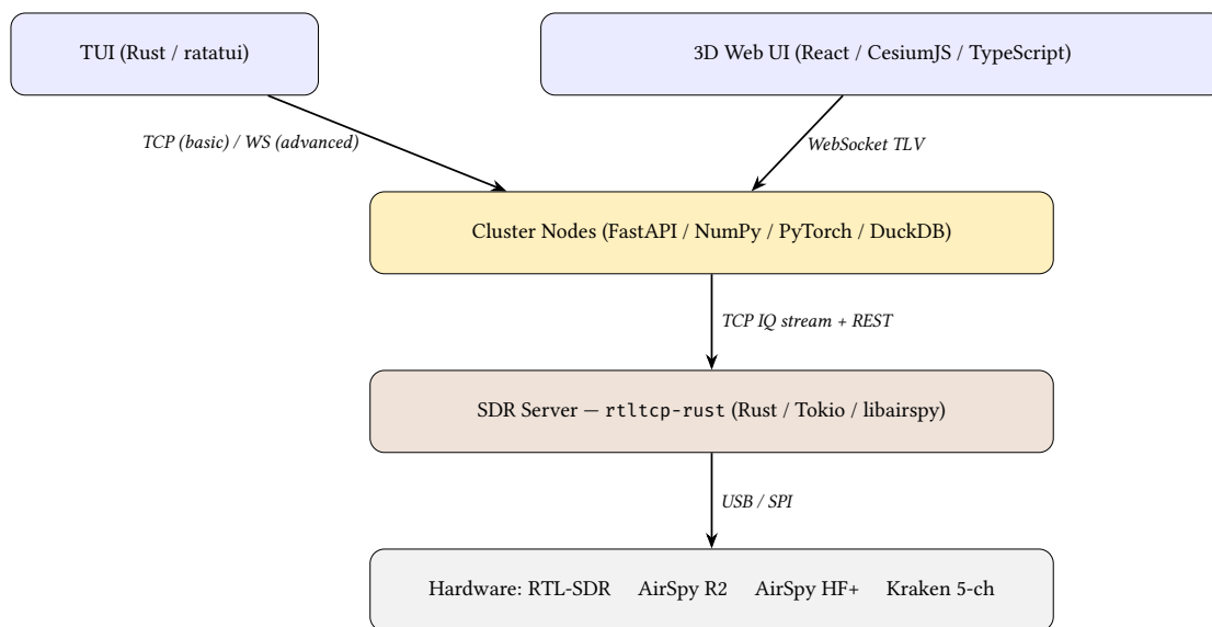
Figure 3. Spectra four-tier architecture. Thin arrows indicate the primary data-flow direction (IQ flows up; commands flow down).
