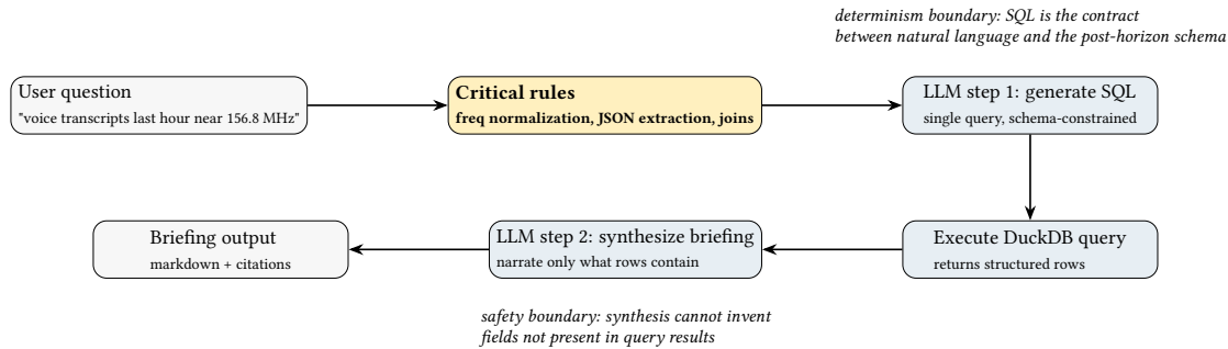
Figure 11. RAG/NLQ as a two-step constrained chain. The first LLM call converts natural language into a schema-valid SQL query under explicit rules; the second LLM call renders only the returned rows into a narrated briefing, preserving Spectra's deterministic AI constraint.
