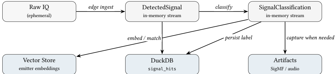
Figure 6. Signal data lifecycle. Raw IQ is treated as ephemeral; persistent storage captures only the distilled outputs and selected artifacts.
