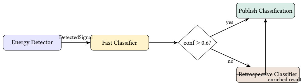
Figure 10. Two-stage classification pipeline. The confidence gate at 0.6 routes low-confidence detections to the retrospective classifier.
