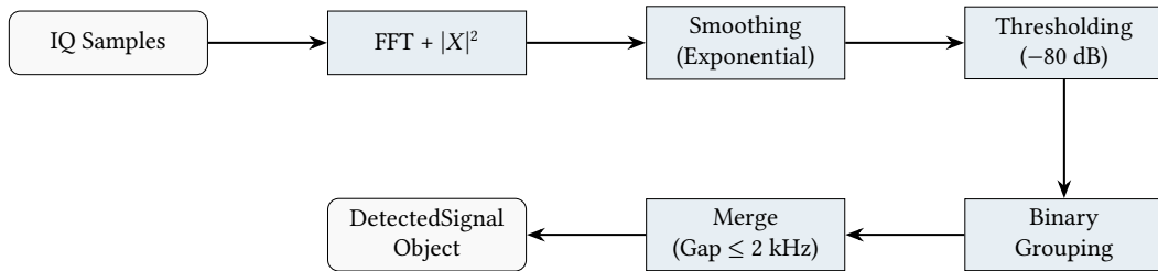
Figure 9. Signal detection pipeline. Raw samples are converted to power spectra, smoothed, and thresholded to produce discrete signal objects.
