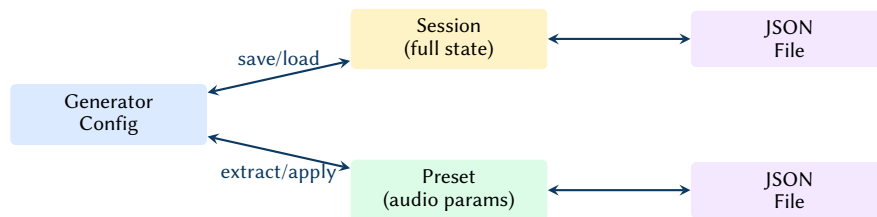
Figure 12. Session and preset persistence: sessions capture full state, presets capture audio parameters only. Both serialise to JSON.
