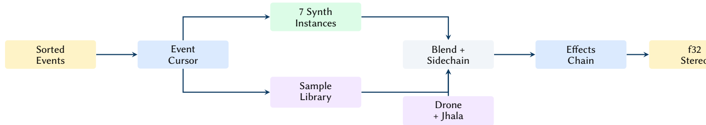
Figure 11. Streaming engine architecture: pre-sorted events are dispatched sample-accurately, blended with energy-aware sample playback, and processed through the effects chain.
