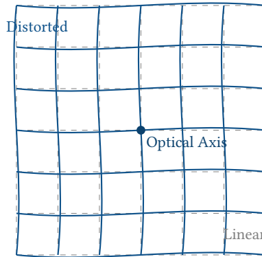
Figure 19. Visualization of SIP polynomial distortion warping the linear TAN projection grid away from the optical axis.
