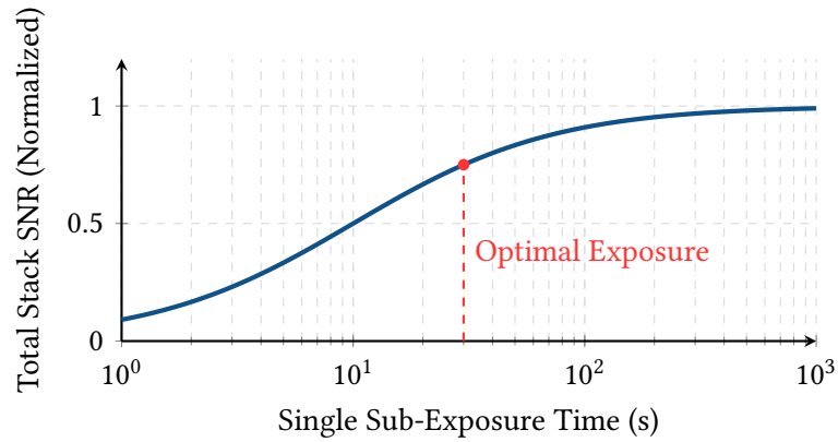
Figure 13. Diminishing returns of sub-exposure time. Once the t_{\text{opt}} threshold is reached (where sky noise swamps read noise), extending the exposure time only increases the risk of ruined frames (e.g., from satellite trails or wind gusts) without improving the final stack’s SNR.
