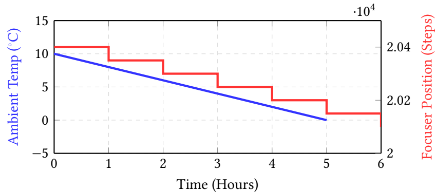
Figure 24. Temperature compensation loop. As the ambient temperature drops steadily (blue), the astro-node daemon autonomously injects computed inward micro-steps to the focuser (red) to maintain critical focus without requiring a sequence-interrupting V-Curve scan.
