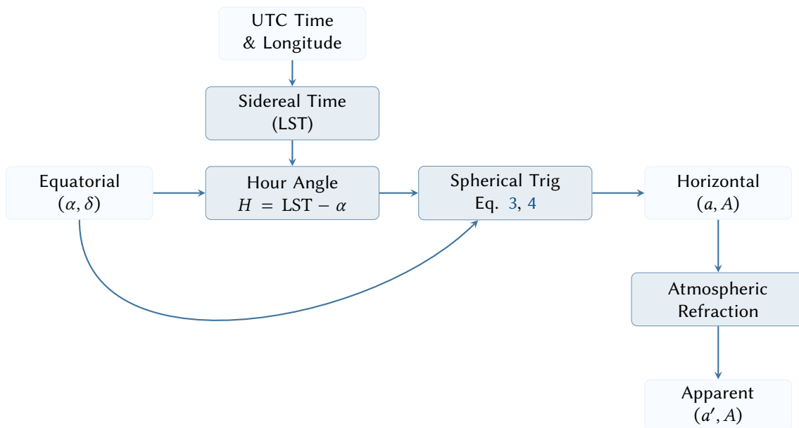
Figure 2. Coordinate transform pipeline mapping equatorial targets to their apparent topocentric positions.
