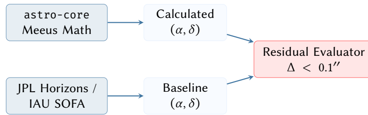
Figure 22. Golden Master CI/CD testing pipeline. The SDK’s coordinate output is dynamically asserted against the gold-standard JPL Horizons ephemeris data [23] to guarantee that the implementation is free from systemic truncations or coordinate frame misinterpretations.
