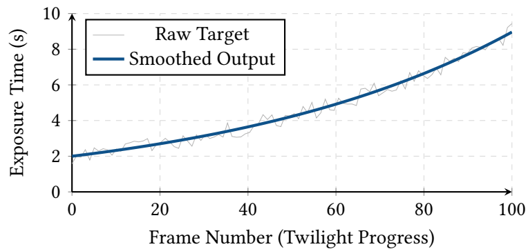
Figure 14. Holy Grail timelapse exposure ramping. The exponential smoothing filter rejects high-frequency noise from passing clouds or atmospheric variations, generating a monotonically increasing exposure schedule that prevents visible flicker.
