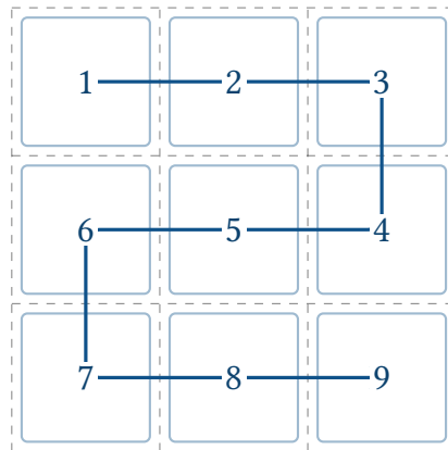
Figure 31. A 3 \times 3 mosaic grid demonstrating the boustrophedon (serpentine) path ordering to minimize mount slew distance.
