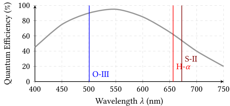
Figure 9. Quantum Efficiency curve of a typical Back-Illuminated (BSI) CMOS sensor. The noise model calculates the expected signal-to-noise ratio by integrating the target's emission spectrum against the sensor's specific QE at key narrowband wavelengths (500.7 nm, 656.3 nm, 672.4 nm).
