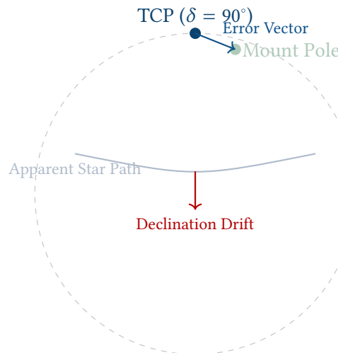
Figure 5. Polar alignment error. A misalignment between the True Celestial Pole (TCP) and the mount’s mechanical polar axis causes stars to exhibit a continuous declination drift over time, which forms the basis of the King drift method.
