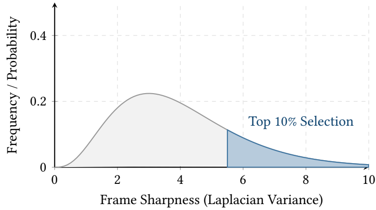
Figure 30. Frame sharpness distribution in a Lucky Imaging sequence. The highly skewed right tail represents the rare frames captured during moments of negligible atmospheric turbulence, which are retained for stacking.
