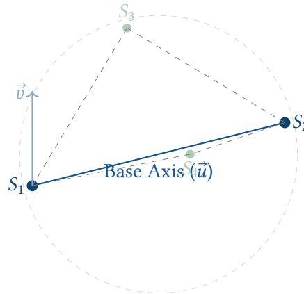
Figure 35. A 4-star geometric “quad” used for blind plate solving. The two most distant stars ( S_1, S_2 ) define a normalized 2D coordinate system ( \vec{u}, \vec{v} ). The internal positions of S_3 and S_4 within this system create a translation-, rotation-, and scale-invariant 4D hash code used to rapidly search the celestial index.
