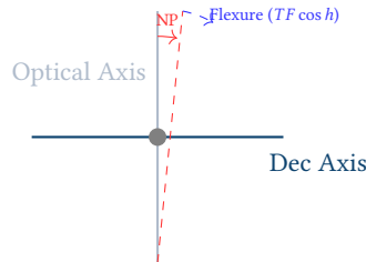
Figure 28. Mount Kinematics. The pointing model corrects for six fundamental mechanical errors: Index errors ( IH , ID ), Polar Elevation/Azimuth ( ME , MA ), Non-perpendicularity ( NP ), and Tube Flexure ( TF ).
