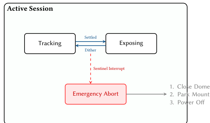
Figure 34. Simplified Harel Statechart of the observatory orchestrator. If the Edge AI Sentinel issues an interrupt (e.g., cloud detected) while the system is nested inside the Exposing or Tracking states, the hierarchy immediately preempts all active futures and transitions to the guaranteed Emergency Abort recovery sequence.
