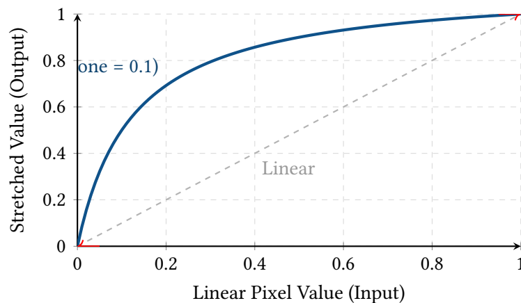
Figure 17. The Midtone Transfer Function (MTF) aggressively expands the dynamic range of the dark background (pulling faint signal up) while compressing the highlights (preventing star cores from blowing out).
