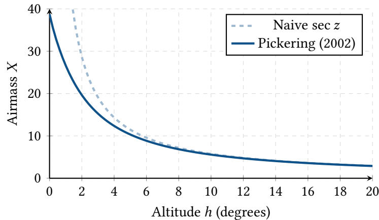
Figure 3. Comparison of airmass models near the horizon. The naive secant approximation diverges to infinity at h = 0^\circ , whereas Pickering's interpolation correctly models atmospheric curvature to match empirical scattering data ( X \approx 38 at the horizon).
