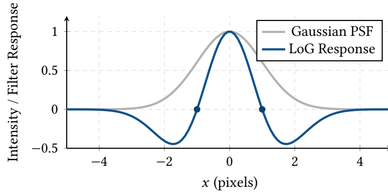
Figure 12. 1D profile of a Gaussian star (grey) and the normalized Laplacian of Gaussian (LoG) filter response (blue). The zero-crossings of the LoG function formally define the inflection edges of the star’s spatial profile, allowing for robust multi-scale star detection invariant to background gradients.
