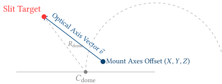
Figure 7. Dome slaving kinematics. Because the telescope mount is offset from the dome's geometric center, the optical axis \vec{v} does not point to the same azimuth as the mount's pointing azimuth. The system must solve the ray-sphere intersection to command the correct dome rotation angle.
