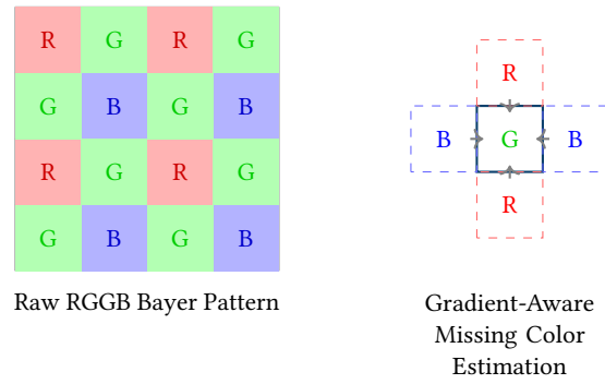
Figure 10. Demosaicing process. The missing color channels at any given pixel are computed using gradient-corrected linear interpolation from neighboring pixels to preserve sharp edges and minimize false-color artifacts.
