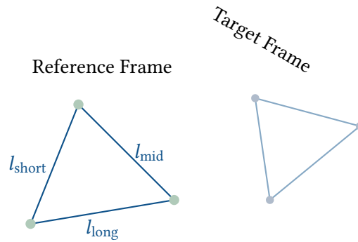
Figure 15. Triangle-similarity matching. The sorted ratios of the sides ( l_{\text{short}}/l_{\text{long}} , l_{\text{mid}}/l_{\text{long}} ) form a scale-, translation-, and rotation-invariant descriptor.
