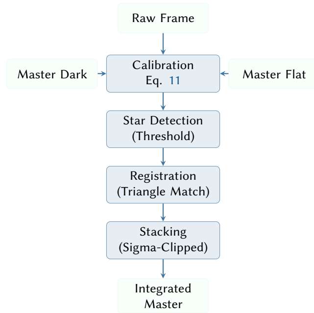
Figure 8. Image processing pipeline from raw sub-exposures to an integrated master frame.
