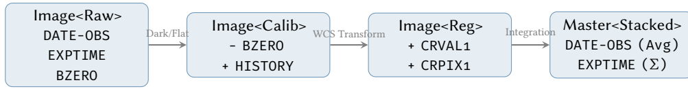
Figure 18. FITS Metadata Provenance. As an image traverses the pipeline, its header keywords are mutated to reflect the mathematical transformations. For example, during stacking, the EXPTIME is summed, while the DATE-OBS is averaged to the exact mid-point of the total integrated exposure span.
