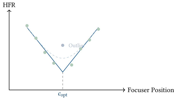
Figure 23. Autofocus V-Curve plotting HFR against focuser position. The robust IRLS fit suppresses the outlier data point.
