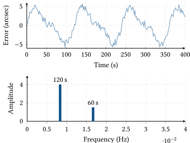
Figure 27. Top: Time-domain simulated tracking error exhibiting a fundamental 120-second worm period and noise. Bottom: FFT frequency-domain spectrum isolating the fundamental frequency (0.0083 Hz) and its first harmonic (0.0166 Hz).
