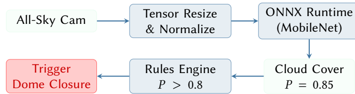
Figure 33. The Sentinel Safety Engine pipeline. Real-time imagery is processed via a cross-platform ONNX inference runtime. The resulting classification probabilities are evaluated against user-defined TOML rules to trigger emergency hardware shutdowns.
