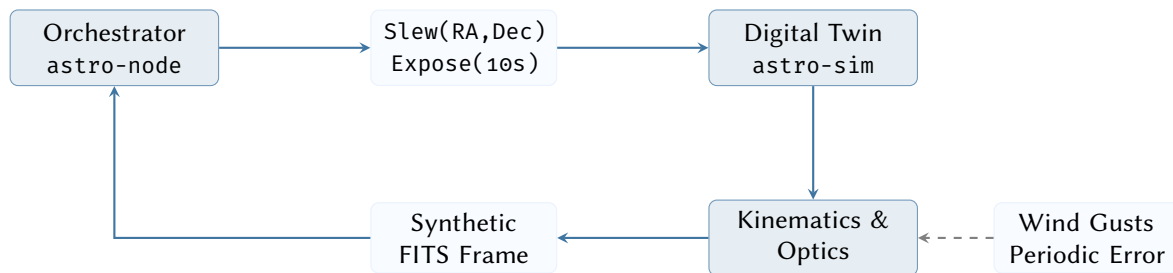
Figure 32. Hardware-in-the-Loop (HITL) closed-loop control simulation. The orchestrator interacts with a digital twin that models telescope kinematics and synthetically renders star fields with injected mechanical tracking errors.
