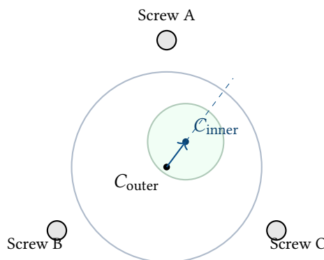
Figure 25. SCT collimation analysis. By computing the eccentricity vector between the outer bounds of the defocused star and the inner central obstruction, the system determines the axis of coma and computes the required secondary mirror screw adjustments.
