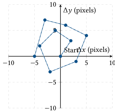
Figure 16. A pseudo-random Dither map over 10 exposures. Between each frame, the mount is commanded to shift slightly. While the stars are re-aligned during registration, the fixed-pattern sensor noise is decoupled and scattered across the grid, allowing the sigma-clipper to successfully reject it.
