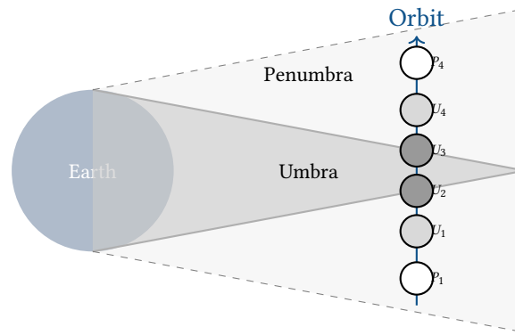
Figure 4. Lunar eclipse shadow geometry showing the Earth’s umbral and penumbral cones. The SDK predicts contact points ( P_1 , U_1 , U_2 , etc.) by stepping through the Moon’s geocentric ecliptic coordinates.
