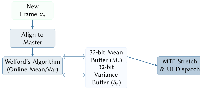
Figure 26. Live Stacking memory architecture. Welford’s single-pass algorithm maintains numerical stability for the running 32-bit mean and variance buffers while preventing Out-of-Memory (OOM) errors during continuous hours-long EAA sessions.
