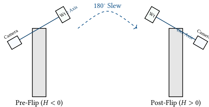
Figure 29. The Meridian Flip. To prevent collision with the pier, the orchestrator halts tracking, rotates the Right Ascension axis by 12 hours ( 180^\circ ), and reverses the Declination axis, effectively placing the camera "above" the mount.
