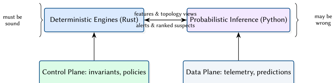
Figure 5. Trust boundary between deterministic analysis and probabilistic inference.
