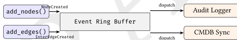
Figure 29. The Reactive Event Pipeline. Mutations in the core engine generate events which are buffered and asynchronously dispatched to Python callbacks.
