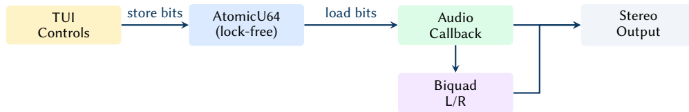
Figure 17. Lock-free live parameter path: the TUI stores f64 bit patterns into atomics; the audio callback loads them each block and updates the biquad filter only when thresholds are exceeded.
