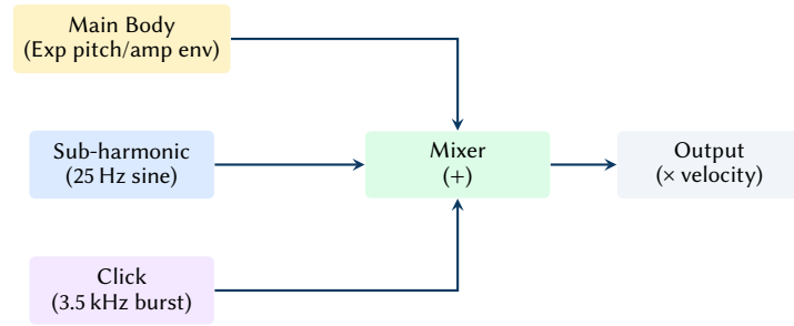
Figure 3. Kick drum synthesis model: parallel summation of main body, sub-harmonic, and click layers.
