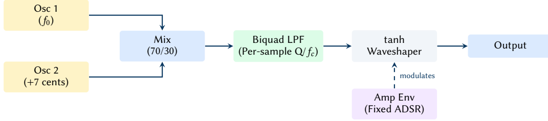
Figure 4. Bass synthesiser signal flow. Oscillators are mixed and passed through a biquad filter with per-sample coefficient updates, followed by soft clipping.
