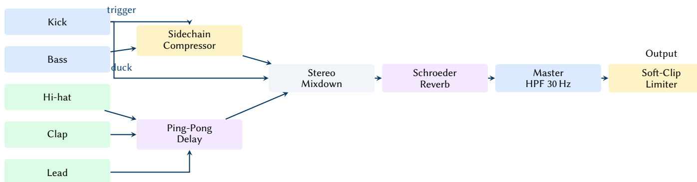
Figure 7. Master effects signal flow. The kick triggers the sidechain compressor which ducks the bass. Hi-hat, clap, and lead pass through the ping-pong delay before joining the stereo bus.
