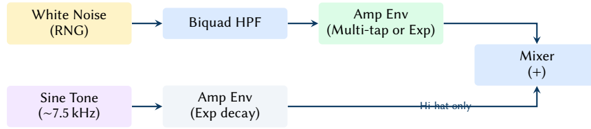
Figure 5. Percussion synthesis model. Hi-hats blend filtered noise with a metallic sine tone, while the clap relies entirely on a multi-tap noise envelope.
