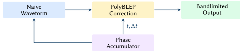
Figure 9. PolyBLEP anti-aliasing: the correction term is subtracted from the naive waveform at phase discontinuities.
