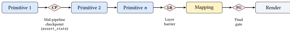
Figure 15. Assertion firing points. CP: mid-pipeline checkpoint (inline assert_state); LB: layer barrier (runs after a layer's primitives complete); FG: final gate (runs before rendering). All three evaluate the same assertion types but fire at different pipeline positions for earlier feedback.
