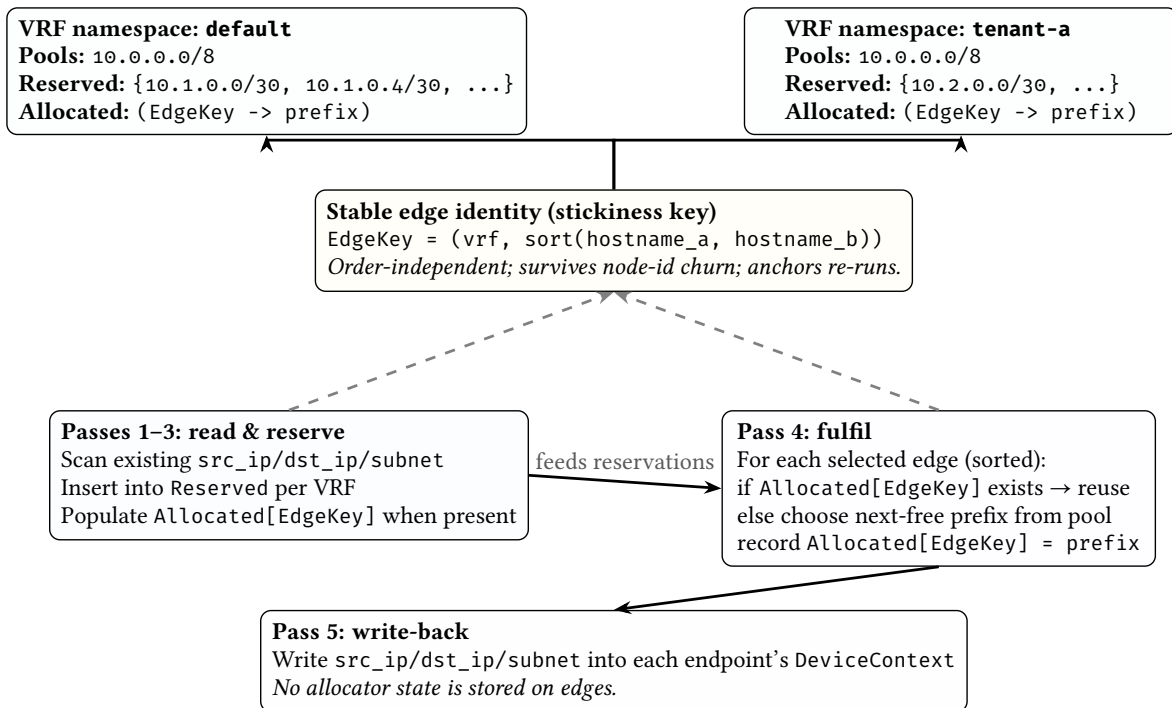
Figure 24. Five-pass IPAM algorithm. Passes 1–3 gather state and reserve existing allocations; pass 4 allocates new subnets; pass 5 writes results to DeviceContext . The two-phase structure (read then write) satisfies Rust’s ownership rules without unsafe code.
