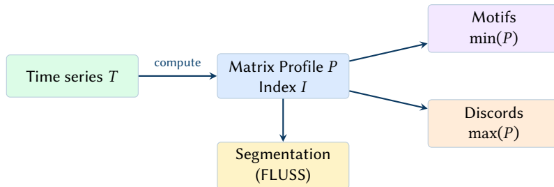
Figure 7. Matrix Profile downstream tasks. The profile vector P supports motif and discord discovery via extrema, while the index vector I supports regime change detection via FLUSS [7].
