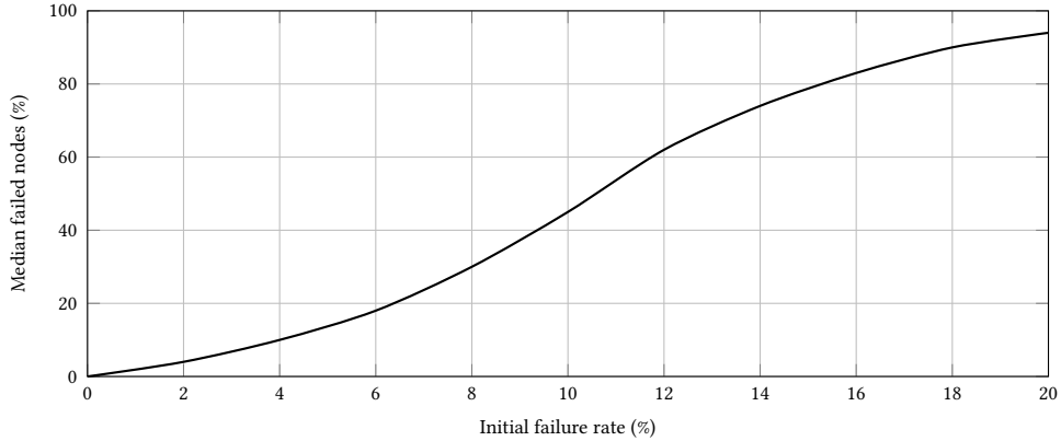
Figure 21. Illustrative resilience curve from Monte Carlo cascade simulation.
