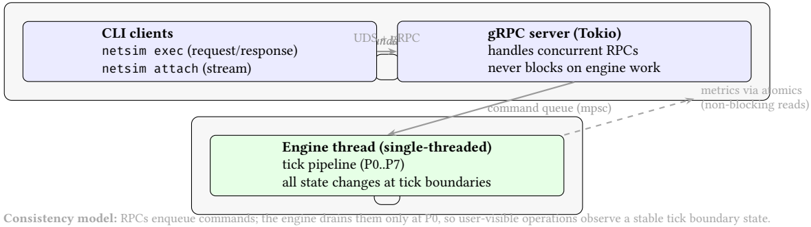
Figure 18. Daemon Architecture as a Consistency Boundary. Concurrency is handled at the RPC layer; determinism is preserved by funneling all mutations through a single-threaded tick loop. Commands are serialized at tick boundary P0, giving the system a clear observable state model.
