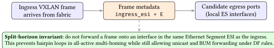
Figure 17. Split-Horizon as an Invariant. EVPN all-active multi-homing relies on explicit ESI metadata to prevent frames from being forwarded back onto the same Ethernet Segment, eliminating hairpin loops without requiring timing-dependent heuristics.
