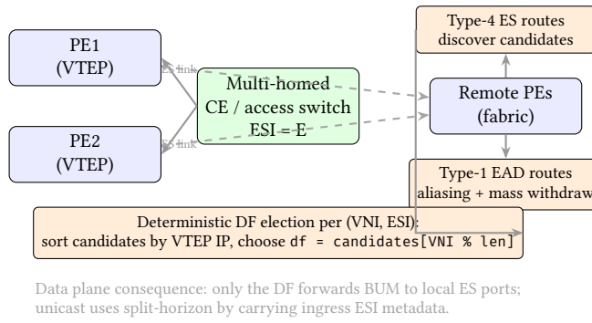
Figure 16. EVPN Multi-Homing as Deterministic Control/Data Coupling. Type-4 routes discover the candidate set for an Ethernet Segment (ESI). A deterministic DF election per VNI selects which PE forwards BUM to local ES ports, while split-horizon prevents loops by dropping frames that would hairpin back onto the same ESI.
