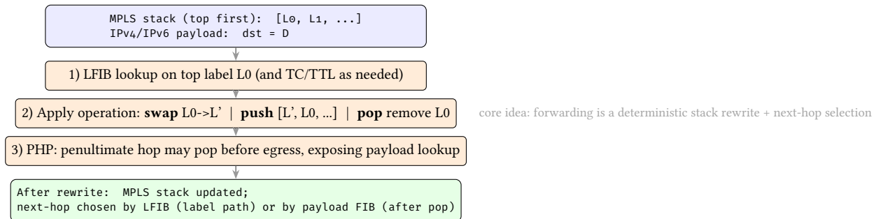
Figure 9. MPLS Forwarding as Label-Stack Rewrite Semantics. The data plane selects an LFIB entry by the top label and then applies a local rewrite (push/swap/pop). PHP is a controlled pop that exposes the payload for final FIB lookup.
