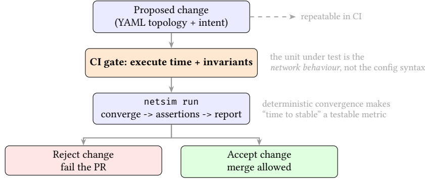
Figure 11. CI Integration as a Behavioural Gate. The topology file encodes both configuration and intent. CI runs netsim to convergence and evaluates assertions, turning routing safety (no loops, no isolation, bounded convergence time) into an automatic merge gate.
