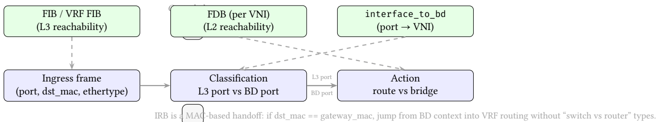
Figure 13. Unified L2/L3 Router as a Conceptual Model. Rather than branching on device type, the data plane classifies each ingress by port-to-bridge-domain membership and then selects an action (route via FIB/VRF or bridge via per-VNI FDB). IRB is a deterministic MAC-based handoff from L2 to L3.
