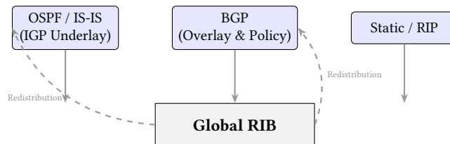
Figure 8. Control Plane Protocol Interactions. Protocols independently compute routes and submit them to the Global RIB, which arbitrates conflicts using administrative distance. The RIB can also redistribute routes back into protocols.
