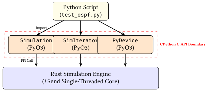
Figure 22. Python Bindings Architecture. The PyO3 wrappers expose the single-threaded Rust Engine directly to the Python interpreter, allowing zero-copy, in-process access to the simulation state.
