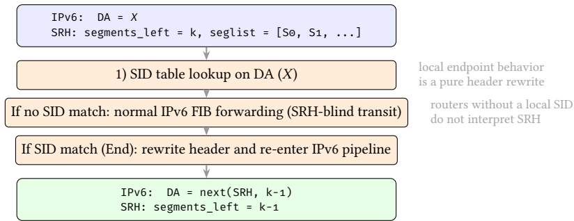
Figure 10. SRv6 Packet Walk as a Header-Rewrite Semantics. A local SID match triggers endpoint behavior that deterministically rewrites (DA, segments_left) and loops back into the IPv6 forwarding pipeline. Routers without a matching local SID forward on the outer DA only.
