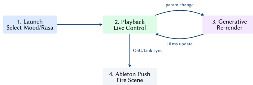
Figure 45. The user workflow journey. Selecting a mood configures the global state. Adjustments during playback trigger an instantaneous generative re-render, with structural updates pushed seamlessly to Ableton Live.
