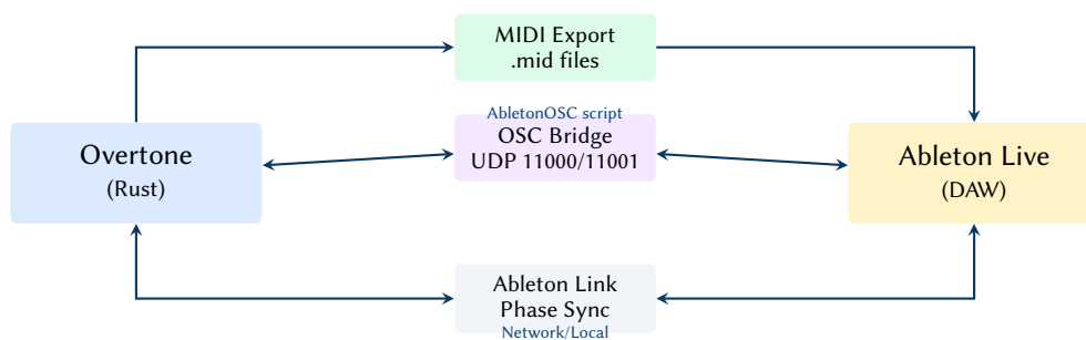
Figure 44. Ableton Live integration architecture. Overtone communicates via Standard MIDI Files for static export, bidirectional OSC for clip pushing and scene control, and Ableton Link for phase-locked transport synchronisation.
