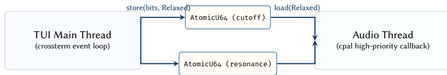
Figure 49. Lock-free concurrency model. The UI thread communicates with the real-time audio thread strictly through atomic variables, preventing priority inversion and guaranteeing that the audio callback never blocks waiting for a mutex.
