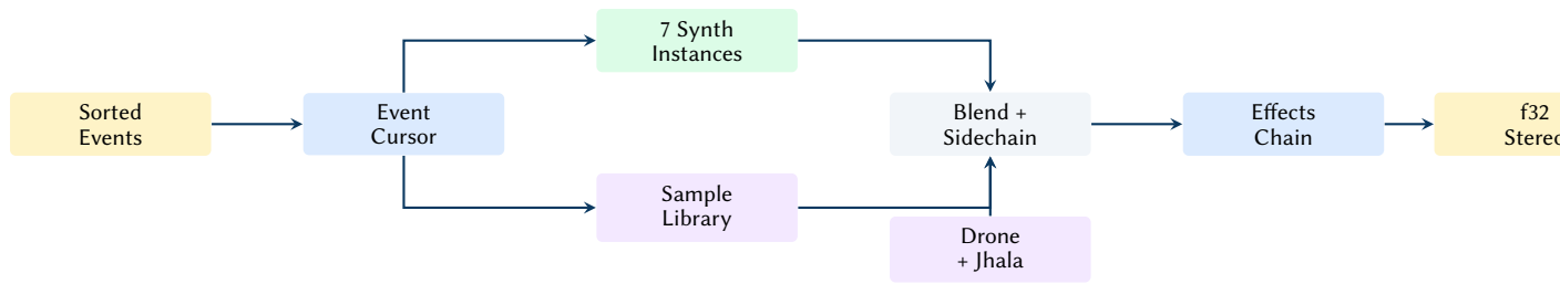
Figure 46. Streaming engine architecture: pre-sorted events are dispatched sample-accurately, blended with energy-aware sample playback, and processed through the effects chain.
