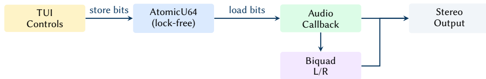
Figure 47. Lock-free live parameter path: the TUI stores f64 bit patterns into atomics; the audio callback loads them each block and updates the biquad filter only when thresholds are exceeded.
