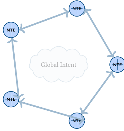
Figure 4. Swarm NTE Architecture. Decentralized nodes negotiate local subgraphs to satisfy global intent constraints.
