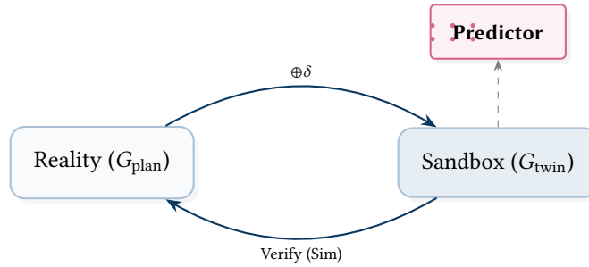
Figure 3. Digital Twin Verification. Parallel graph instances are used to test remediation stability before deployment.
