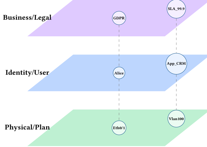
Figure 2. The Semantic Knowledge Graph. Intent is propagated from business constraints (e.g., GDPR data residency) through user identity down to the physical plan topology.
