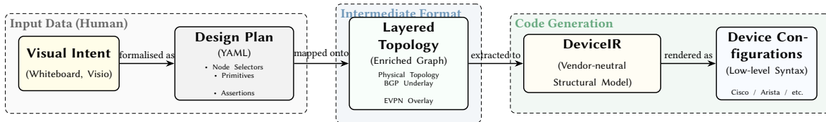
Figure 3. The Configuration Synthesis Pipeline. The operator formalises high-level Visual Intent into a declarative Design Plan . The primitives in this plan are mapped onto a Layered Topology , which is extracted into a DeviceIR and rendered as low-level Device Configurations .
