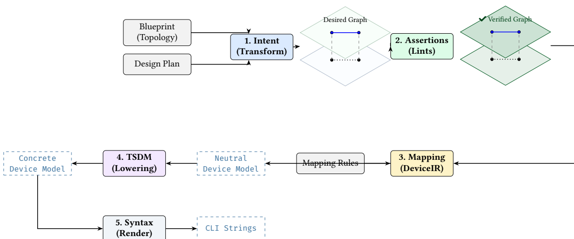
Figure 5. NetCfg compilation pipeline. High-level intent is progressively lowered through three distinct mathematical graph representations (Verified Graph, Neutral Device Model, Concrete Device Model) before serialisation.
