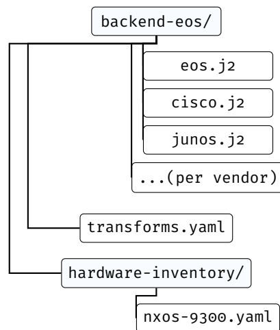
Figure 9. Target backend package structure. Templates render per-vendor syntax; transforms.yaml declares TSDM lowering rules; hardware-inventory/ maps chassis models to slot layouts. Most organisations author this once per platform and reuse it across sites.
