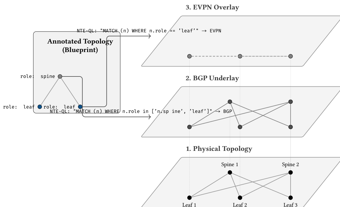
Figure 6. Intent Mapping to Layered Topology. Rather than compiling unstructured templates, operators declare intent in a Design Plan. Primitives in the plan directly map logical intent onto orthogonal topology layers.
