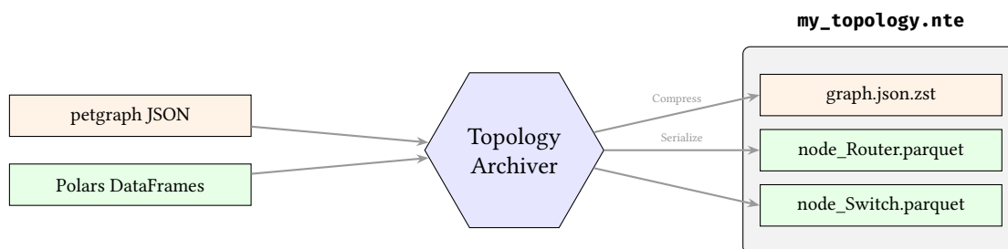
Figure 27. The .nte archive format. Structural graph data is compressed via zstd , while DataFrames are serialised directly to columnar Parquet files, all packaged into a standard ZIP archive.
