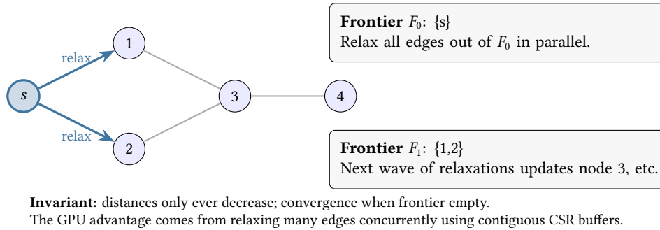
Figure 49. GPU SSSP as wavefront relaxation. Each iteration processes a frontier of active vertices and relaxes outgoing edges in parallel. This maps naturally onto GPU execution when adjacency is stored in compact buffers.
