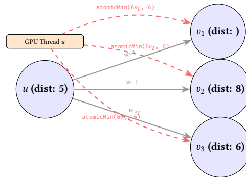
Figure 58. GPU SSSP relaxation. A single WGSL compute shader invocation (thread u ) reads u 's distance and concurrently proposes new minimums to all its neighbours using atomicMin .
