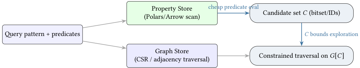
Figure 47. Filter-first planning as candidate-set narrowing. Property predicates are evaluated first to produce a set C of eligible nodes/edges. Structural traversal then runs against the induced subgraph G[C] , avoiding work on irrelevant regions of the topology.
