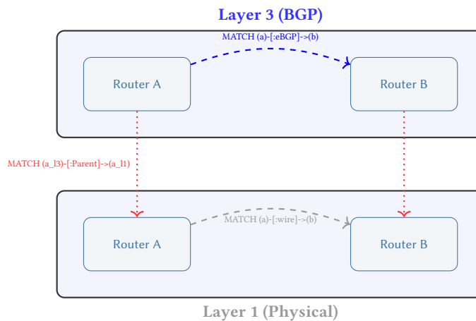
Figure 16. Cross-Layer Semantic Querying. Users can independently query the semantic graph of each layer and trace dependencies across them using the Parent edges, entirely abstracted from the underlying port complexities.
