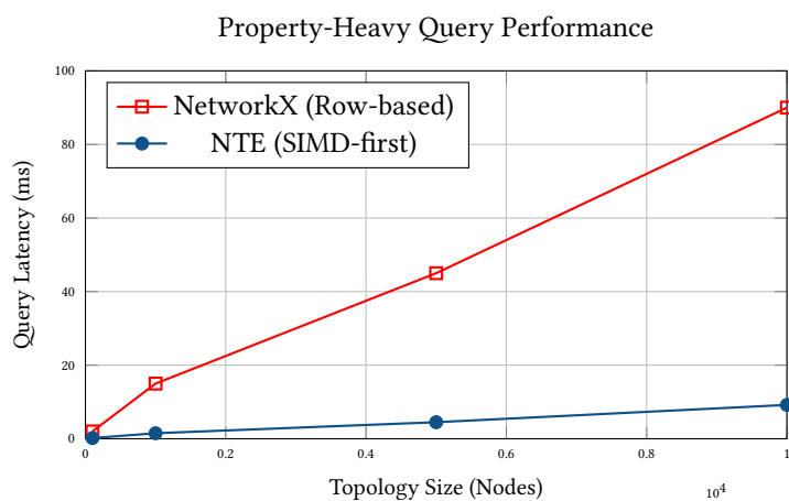
Figure 64. Scaling Performance: NTE vs. NetworkX for complex property filters. NTE’s Polars-backed SIMD scans maintain linear scaling with a significantly lower constant factor compared to row-based alternatives.
