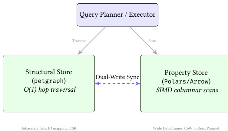
Figure 37. Dual-write architecture synergy. Structural queries target the graph engine, while property-heavy predicates target the columnar store.
