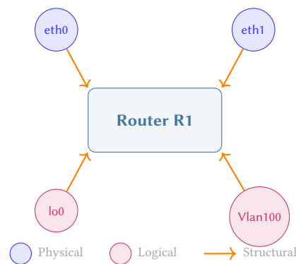
Figure 5. A device with mixed physical and logical endpoints. Physical endpoints ( eth0 , eth1 ) represent hardware ports; logical endpoints ( lo0 , Vlan100 ) represent software-defined connection points. All are owned by the same node via Structural edges.
