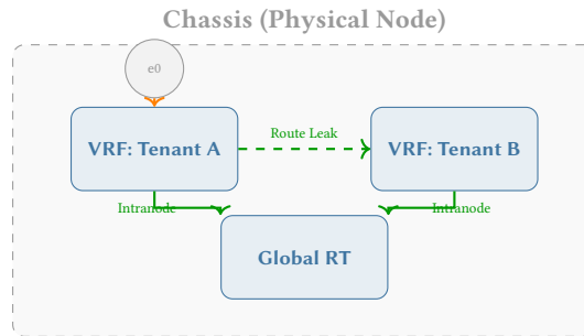
Figure 9. Intranode edges within a chassis. VRF sub-nodes connect to the Global Routing Table via Intranode edges. Each sub-node can optionally own its own Endpoints (shown on VRF: Tenant A). The dashed edge represents a route-leak relationship.
