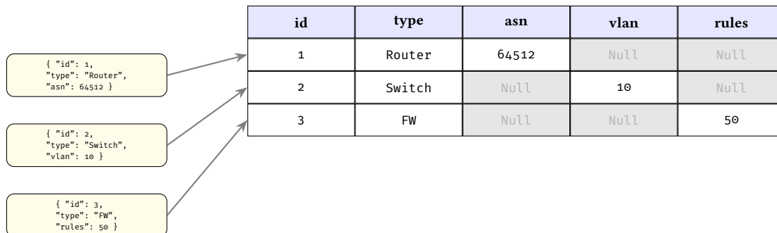
Figure 38. The Wide-Column Sparsity Matrix. Heterogeneous JSON properties are flattened into a single wide DataFrame. Arrow’s validity bitmaps efficiently compress the resulting Null regions.
