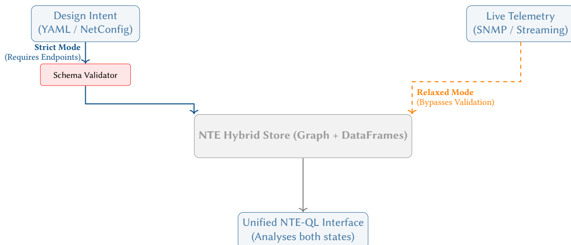
Figure 21. Bimodal Execution Architecture. Strict mode forces design intent through schema validation (ensuring the Endpoints model is perfectly adhered to). Relaxed mode bypasses validation, allowing live telemetry to stream directly into the engine. Both modes share the same unified NTE-QL interface.
