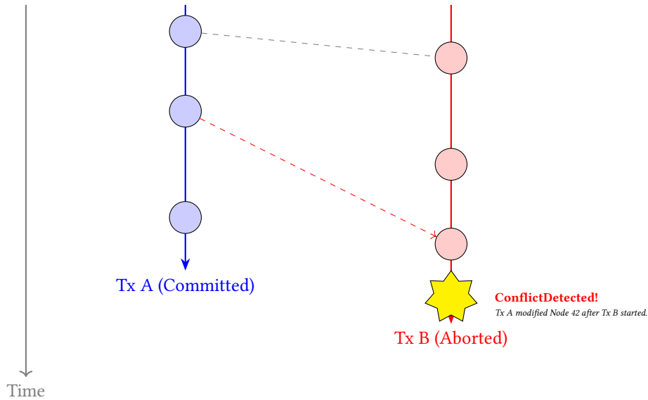
Figure 25. MVCC Transaction Timeline. Both transactions read from the same initial snapshot S_0 . Because Tx A commits a mutation to Node 42 before Tx B attempts to mutate it, the Conflict Engine safely aborts Tx B to prevent a Write-Write conflict.
