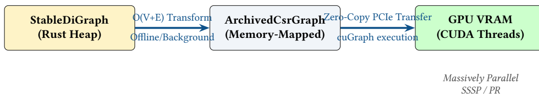
Figure 57. The Graph-to-GPU Pipeline. Because pointer-based graphs cannot be sent to the GPU, the adjacency list is serialised into a flattened Compressed Sparse Row (CSR) structure, which is then DMA-transferred to the GPU for parallel analytics.
