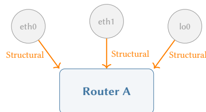
Figure 7. Structural (Ownership) edges. Three Endpoints are owned by a single Node. Arrows point from Endpoint to Node, expressing the “belongs to” relationship.
