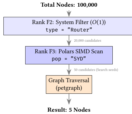
Figure 53. The Cardinality Funnel (Filter-First Execution). Cheap columnar operations aggressively prune candidates, ensuring the more expensive graph traversal engine only visits a tiny fraction of the topology.
