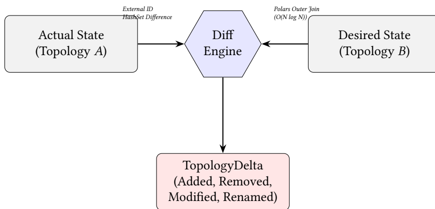
Figure 28. Topology Diffing Pipeline. The engine combines structural set operations with vectorized relational joins to identify deviations between Actual and Desired network states.
