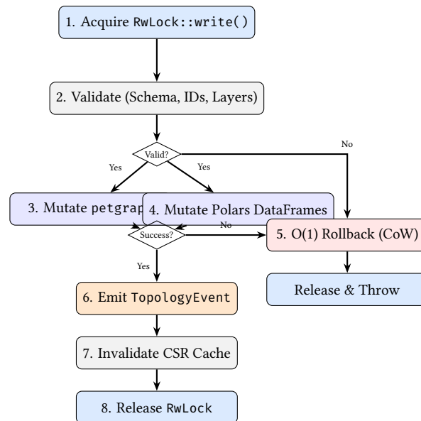
Figure 41. The dual-write transaction lifecycle. Copy-on-Write semantics allow O(1) rollback if either the graph or the DataFrame mutation fails.
