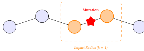
Figure 20. Incremental Validation via Impact Radius. By identifying the nodes physically and logically adjacent to a mutation, NTE avoids the O(V) cost of global policy re-evaluation.
