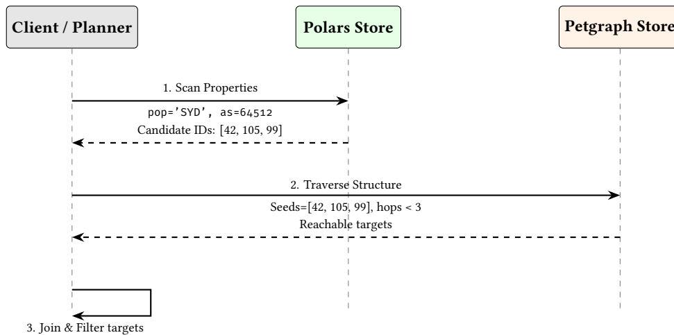
Figure 56. The Filter-First Pipeline. Relational scans prune the search space before expensive graph traversals are initiated.
