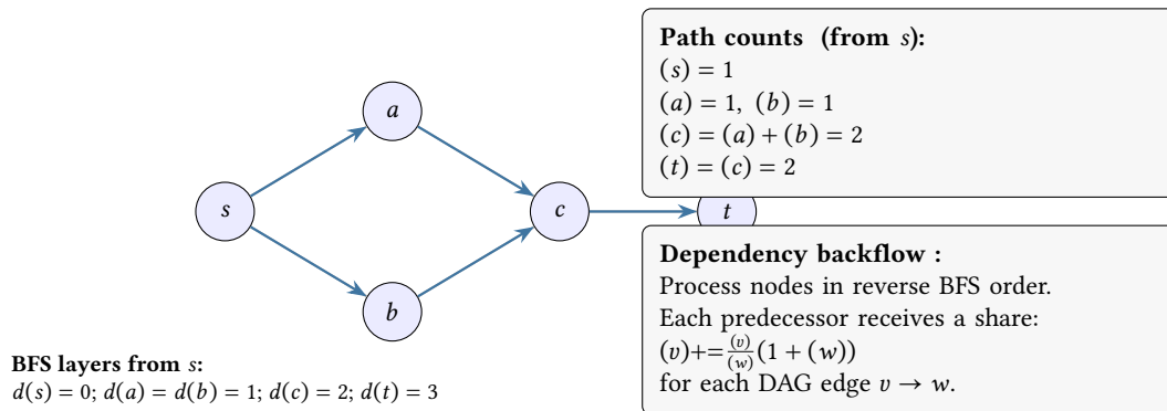
Figure 45. Brandes betweenness centrality as a conserved "flow" on the shortest-path DAG. The forward BFS counts how many shortest paths reach each node ( \sigma ). The reverse accumulation distributes dependency ( \delta ) back to predecessors in proportion to their contribution.
