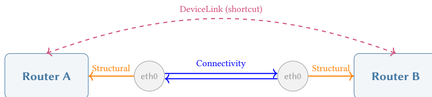
Figure 10. The DeviceLink shortcut. The dashed purple edge bypasses the three-hop Structural–Connectivity–Structural path, providing direct device-to-device adjacency for common queries.
