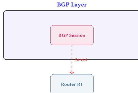
Figure 6. A LogicalNode (BGP Session) residing within a layer plane, linked to its parent physical Node via a Parent edge. Logical nodes are excluded from default queries unless their layer is explicitly targeted.
