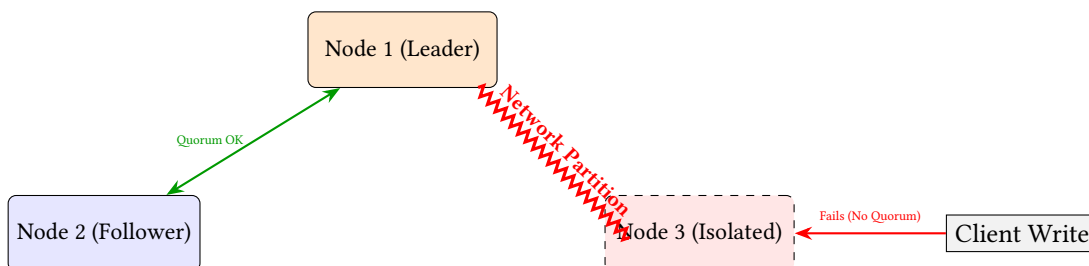
Figure 35. Split-Brain Resolution. In a partition, the isolated Node 3 rejects writes because it cannot replicate logs to a majority quorum. Nodes 1 and 2 continue processing safely.
