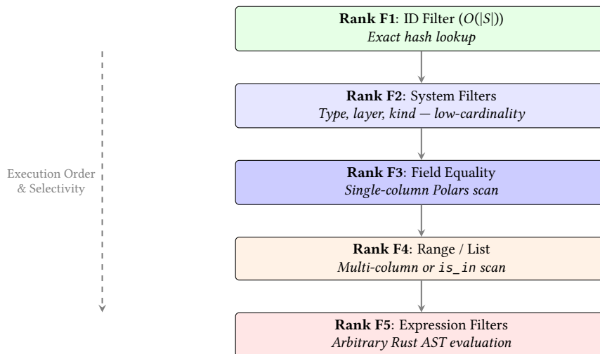
Figure 54. Query Planner Execution Ranks. Predicates are sorted and executed from cheapest (F1) to most expensive (F5) to continuously reduce the candidate set.
