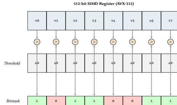
Figure 40. Hardware-Level Predicate Evaluation. A single AVX-512 instruction evaluates multiple property values in parallel, producing a bitmask that drives the subsequent graph traversal filter.
