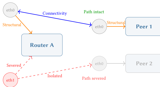
Figure 23. Blast Radius Propagation. When Line Card 2 fails, its outgoing Structural edge is severed. The connection to Peer 2 is isolated whilst Peer 1 remains unaffected because eth0 and eth1 reside on different endpoints with intact Structural edges. A naive (Router)-[CONNECTED_TO]->(Router) model cannot express this partial failure.
