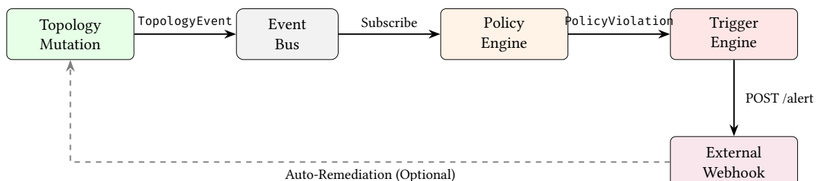
Figure 63. Proposed Reactive Topology workflow: Automated policy validation pushing events to the Trigger Engine rather than waiting for pull-based queries.
