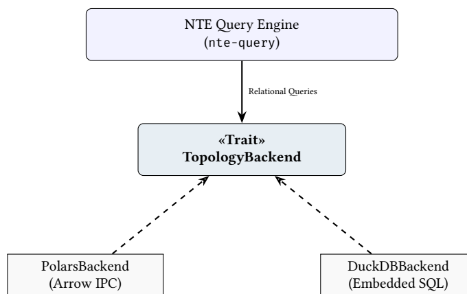
Figure 43. Trait-Based Abstraction. The core query engine interacts only with the TopologyBackend interface, allowing the physical columnar storage (Polars vs. DuckDB) to be swapped at compile time.
