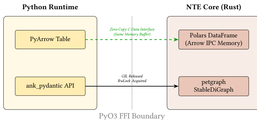
Figure 42. The FFI Zero-Copy Boundary. Unlike traditional RPC-based graph databases, NTE embeds directly in the Python process. The Arrow C Data Interface allows Python tools to read the Rust memory buffers without any serialisation overhead.
