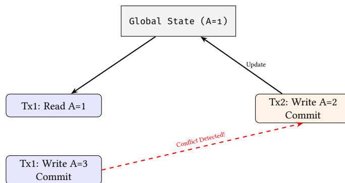
Figure 26. Serializable isolation conflict detection. Tx1 fails to commit because its read-set ( A=1 ) was invalidated by Tx2's concurrent write.
