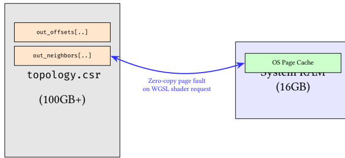
Figure 29. Mmap CSR Execution. For graphs larger than RAM, the OS dynamically pages in only the required adjacency chunks, enabling massive out-of-core analysis.
