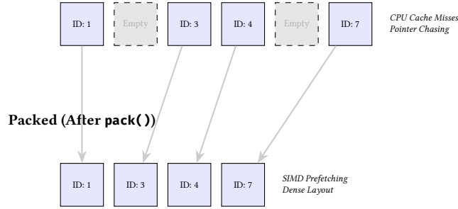
Figure 39. Memory Defragmentation (Graph Packing). The pack() operation removes tombstone slots from the internal adjacency arrays, restoring linear CPU cache locality and reducing memory overhead.
