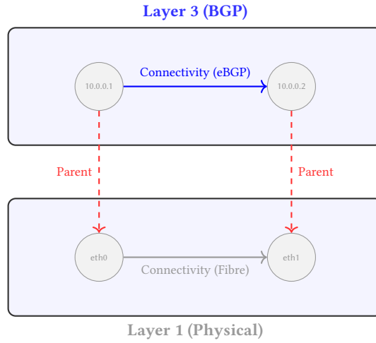
Figure 11. Cross-Layer Relationships. L3 BGP Endpoints are bound to L1 Physical Endpoints via Parent edges. If eth0 fails, the engine traverses the incoming Parent edge to deterministically tear down the dependent BGP session.
