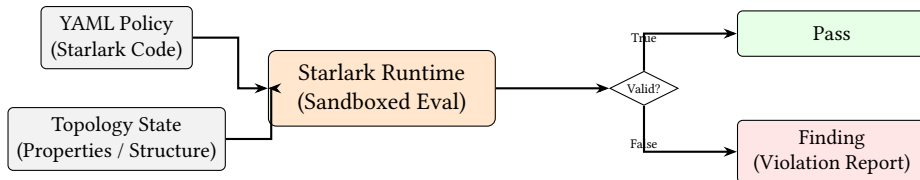
Figure 17. Starlark Policy Evaluation. The sandboxed runtime safely evaluates Python-like policy code against the topology state to generate deterministic compliance findings.
