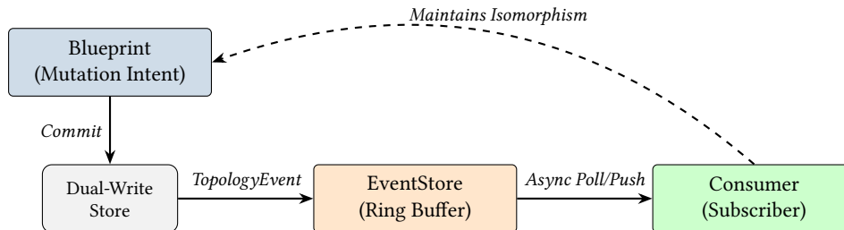
Figure 30. The Reactive Event Pipeline. Structural and relational changes are emitted as typed events, which bridge the physical storage layer back to the Intent Specification domain.
