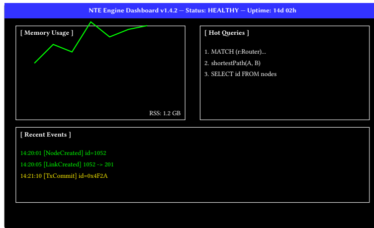
Figure 60. Mockup of the nte-cli TUI Dashboard. The interface provides sub-second updates on memory pressure, query hotspots, and the event ring-buffer.
