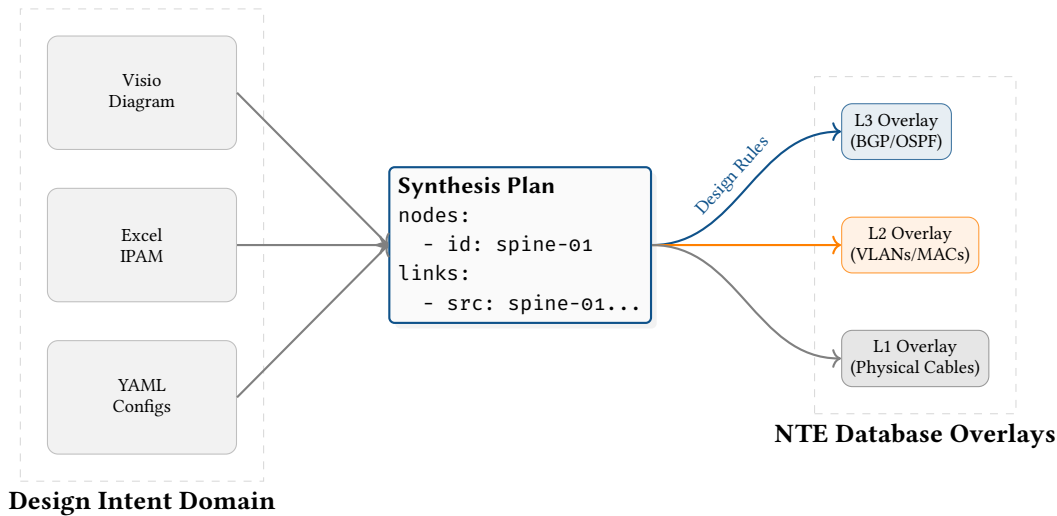
Figure 22. Multi-source aggregation: diverse input sources are normalised into a singular formal Blueprint, which the engine compiles and fans out into rigorous, multi-layered topology overlays.
