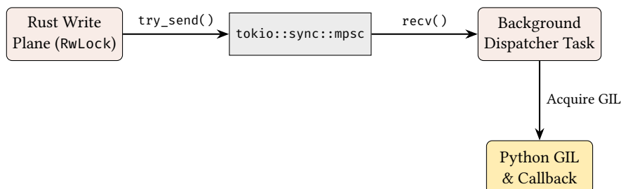
Figure 62. Proposed Async Decoupling: Removing the Python GIL acquisition from the critical Rust database mutation path.
