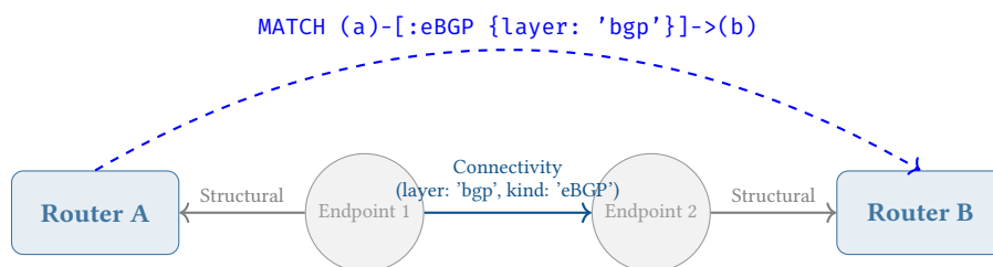
Figure 14. Virtual Cypher Translation. The user specifies a semantic device-to-device relationship (dashed line). The query planner intercepts this and automatically compiles it into the three-hop endpoint traversal (solid lines) required by the structural data model.
