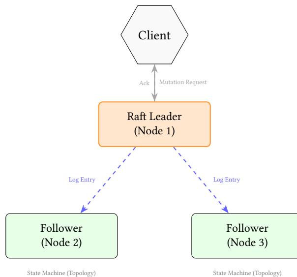
Figure 34. Distributed Raft consensus flow. Mutations are proposed to the leader, replicated to followers, and applied only after reaching a quorum.
