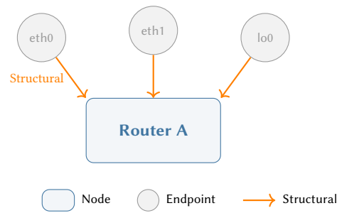
Figure 4. A Node with three Endpoints. Each Structural edge points from the Endpoint to its owning Node, expressing the ownership relationship.
