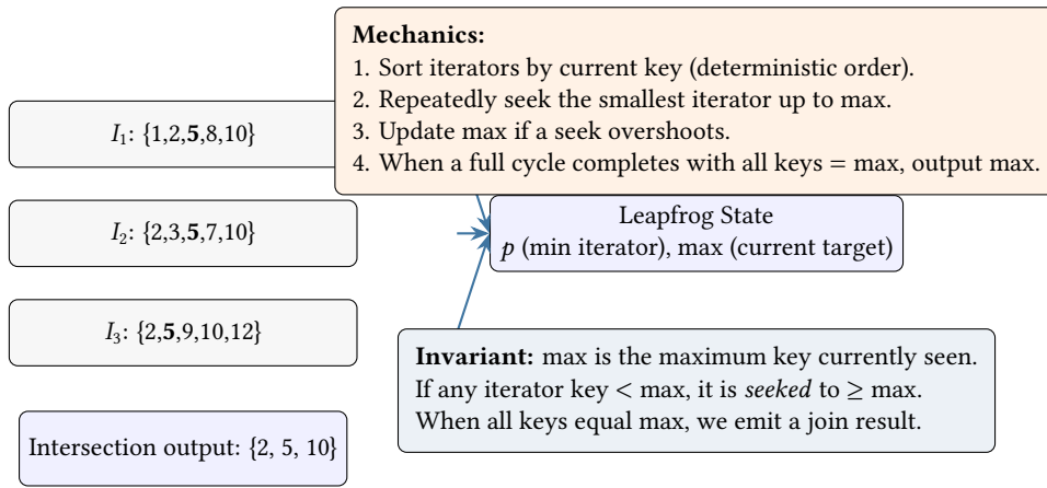
Figure 44. Leapfrog Triejoin as a stateful multi-way intersection. The algorithm maintains a single target (max) and advances the smallest iterator until all iterators align on the same key. This avoids intermediate-result explosion on cyclic patterns by intersecting all constraints simultaneously.
