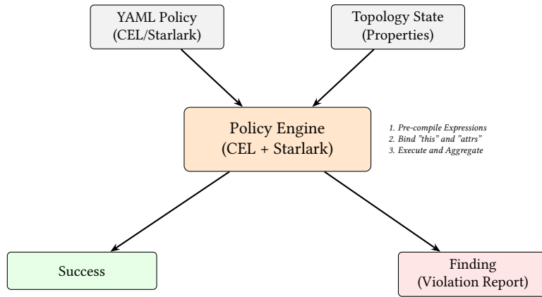
Figure 18. Policy Evaluation Pipeline. The engine pre-compiles declarative CEL expressions and procedural Starlark logic, executing them against a unified topology context to generate structured findings.
