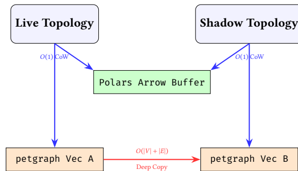
Figure 19. The Hybrid Snapshot Reality. While property DataFrames share memory instantly via CoW pointers, the underlying petgraph adjacency lists must be physically deep-copied into new memory allocations.
