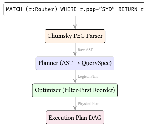
Figure 55. The NTE-QL compilation pipeline. String queries are parsed, converted into programmatic QuerySpec structures, and fed into the same optimizer as the Python APIs.
