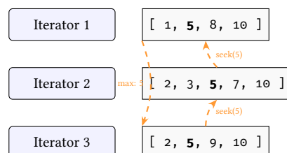
Figure 61. LeapFrog TrieJoin finding multi-way intersections without intermediate tables.
