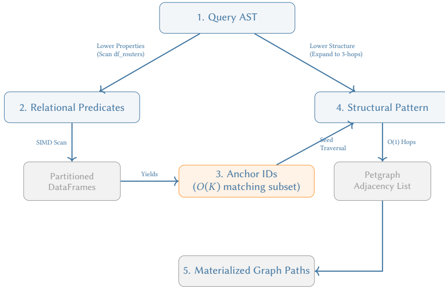
Figure 52. The Filter-First Hybrid Execution Pipeline. During the AST compilation phase, the engine splits the query. It executes highly-selective property predicates against partitioned columnar storage first , yielding a tiny subset of Anchor IDs. These anchors seed the expanded 3-hop structural graph traversal, guaranteeing that the engine never traces paths from irrelevant nodes.
