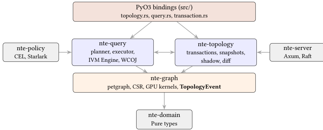
Figure 36. The Layered Crate Architecture. Shared foundation types (Events) are pushed down to nte-graph to enable clean, uni-directional dependency flow between the query engine and topology manager.
