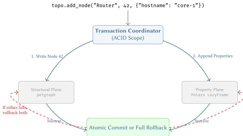
Figure 24. The Dual-Write Transaction Model. Mutations are coordinated atomically across the divergent storage engines. If a node is added to the graph but the properties fail schema validation in Polars, the entire transaction aborts, ensuring the digital twin never enters a split-brain state.
