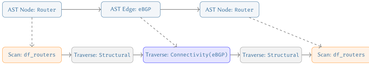
Figure 15. AST Compilation to Execution Plan. The semantic Cypher AST (top) is mathematically expanded by the Query Planner into a deterministic traversal plan (bottom) across the normalised Endpoints graph and partitioned DataFrames.
