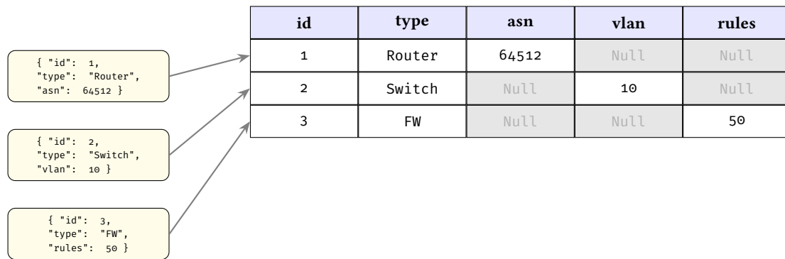
Figure 10. The Wide-Column Sparsity Matrix. Heterogeneous JSON properties are flattened into a single wide DataFrame. Arrow’s validity bitmaps efficiently compress the resulting Null regions.
