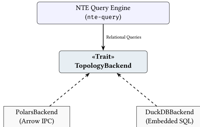
Figure 14. Trait-Based Abstraction. The core query engine interacts only with the TopologyBackend interface, allowing the physical columnar storage (Polars vs. DuckDB) to be swapped at compile time.
