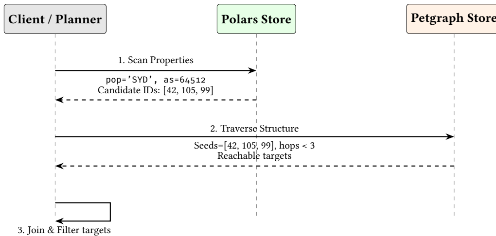
Figure 19. The Filter-First Pipeline. Relational scans prune the search space before expensive graph traversals are initiated.
