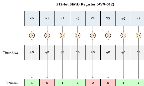
Figure 11. Hardware-Level Predicate Evaluation. A single AVX-512 instruction evaluates multiple property values in parallel, producing a bitmask that drives the subsequent graph traversal filter.
