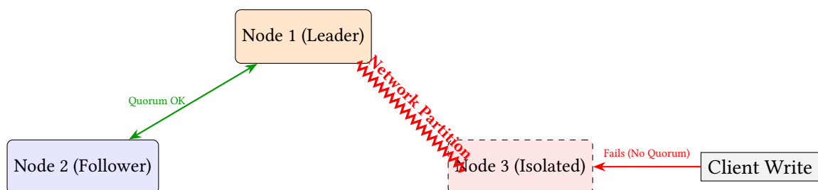
Figure 33. Split-Brain Resolution. In a partition, the isolated Node 3 rejects writes because it cannot replicate logs to a majority quorum. Nodes 1 and 2 continue processing safely.
