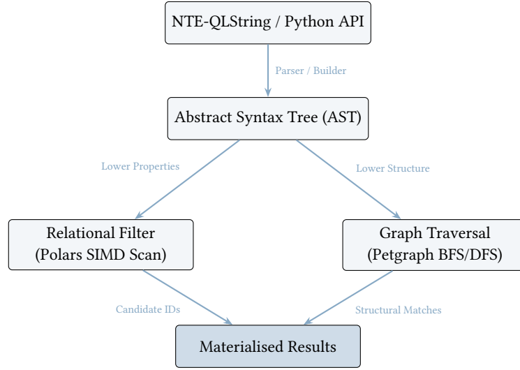
Figure 15. The Query Lowering Pipeline. High-level intent is decomposed into parallel relational and structural execution tasks.
