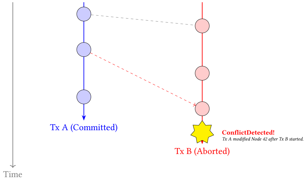
Figure 20. MVCC Transaction Timeline. Both transactions read from the same initial snapshot S_0 . Because Tx A commits a mutation to Node 42 before Tx B attempts to mutate it, the Conflict Engine safely aborts Tx B to prevent a Write-Write conflict.
