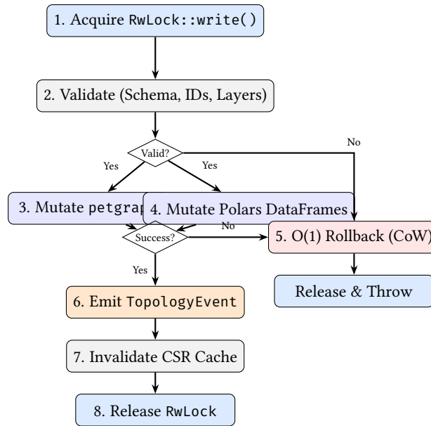
Figure 12. The dual-write transaction lifecycle. Copy-on-Write semantics allow O(1) rollback if either the graph or the DataFrame mutation fails.
