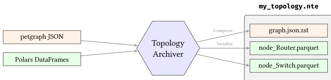
Figure 22. The .nte archive format. Structural graph data is compressed via zstd , while DataFrames are serialised directly to columnar Parquet files, all packaged into a standard ZIP archive.
