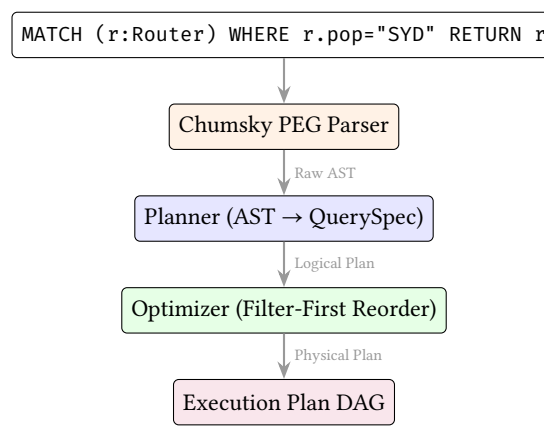
Figure 18. The NTE-QL compilation pipeline. String queries are parsed, converted into programmatic QuerySpec structures, and fed into the same optimizer as the Python APIs.
