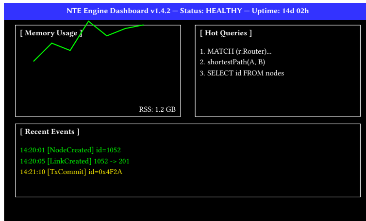
Figure 31. Mockup of the nte-cli TUI Dashboard. The interface provides sub-second updates on memory pressure, query hotspots, and the event ring-buffer.
