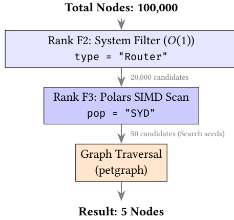
Figure 16. The Cardinality Funnel (Filter-First Execution). Cheap columnar operations aggressively prune candidates, ensuring the more expensive graph traversal engine only visits a tiny fraction of the topology.
