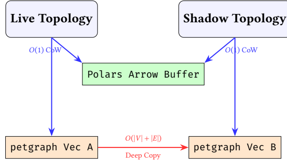
Figure 7. The Hybrid Snapshot Reality. While property DataFrames share memory instantly via CoW pointers, the underlying petgraph adjacency lists must be physically deep-copied into new memory allocations.
