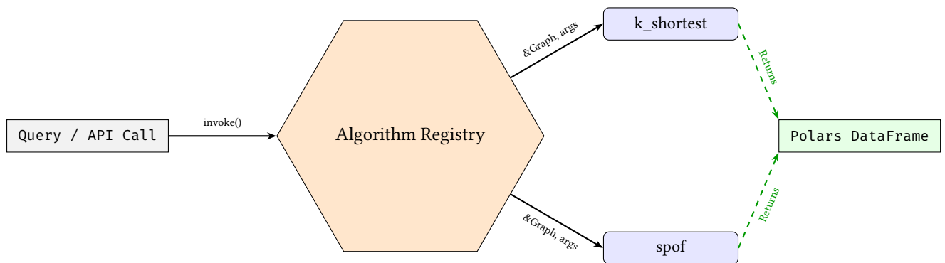
Figure 26. Graph Algorithm Plugin Architecture. Algorithms are invoked by namespace, operate on the shared graph reference, and uniformly return results as Polars DataFrames.
