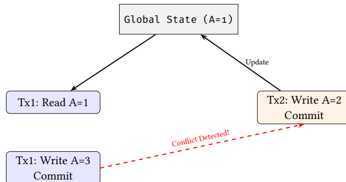
Figure 21. Serializable isolation conflict detection. Tx1 fails to commit because its read-set ( A=1 ) was invalidated by Tx2's concurrent write.
