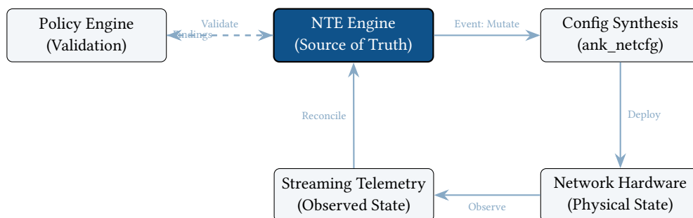
Figure 30. The Autonomous Closed-Loop Cycle. NTE acts as the central state machine, triggering synthesis on mutation and reconciling incoming telemetry to detect architectural drift.
