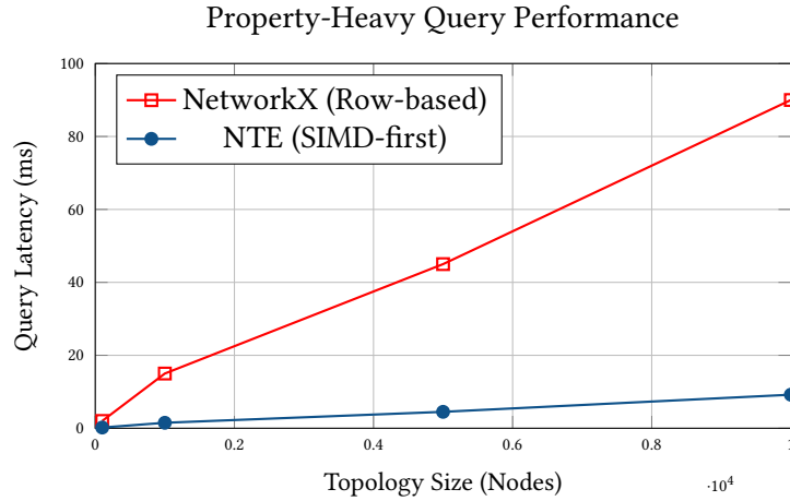
Figure 36. Scaling Performance: NTE vs. NetworkX for complex property filters. NTE’s Polars-backed SIMD scans maintain linear scaling with a significantly lower constant factor compared to row-based alternatives.
