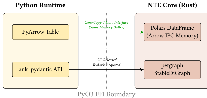
Figure 13. The FFI Zero-Copy Boundary. Unlike traditional RPC-based graph databases, NTE embeds directly in the Python process. The Arrow C Data Interface allows Python tools to read the Rust memory buffers without any serialization overhead.
