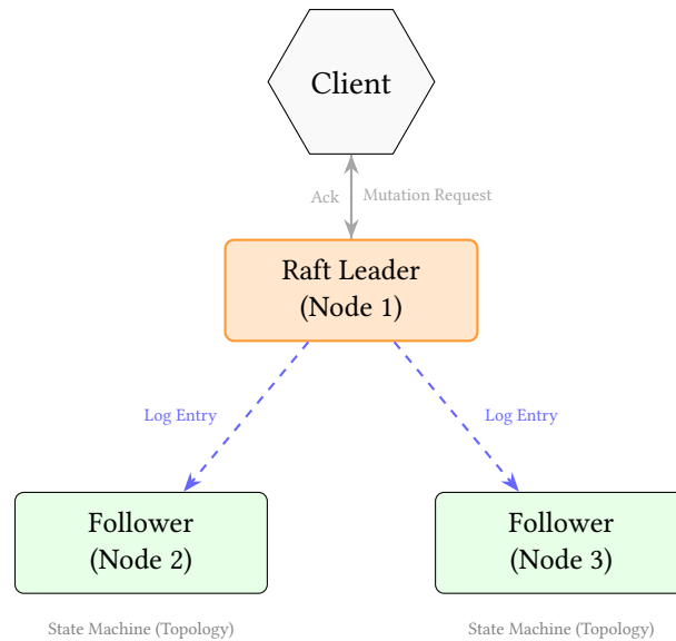
Figure 32. Distributed Raft consensus flow. Mutations are proposed to the leader, replicated to followers, and applied only after reaching a quorum.
