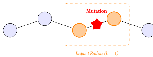
Figure 8. Incremental Validation via Impact Radius. By identifying the nodes physically and logically adjacent to a mutation, NTE avoids the O(V) cost of global policy re-evaluation.
