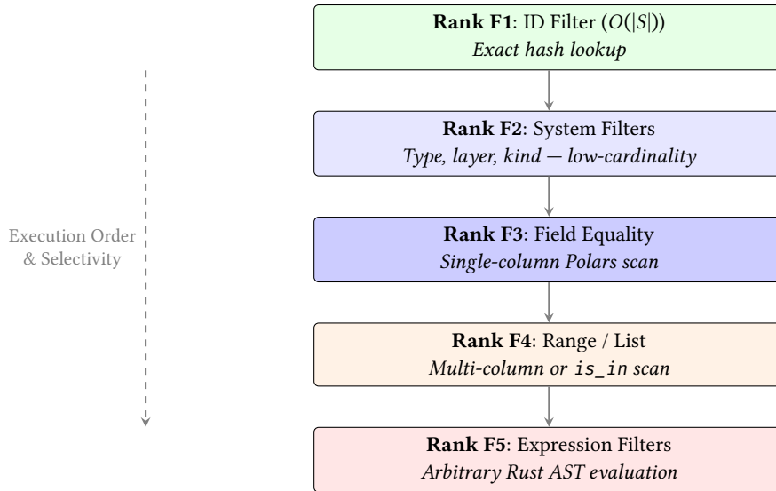
Figure 17. Query Planner Execution Ranks. Predicates are sorted and executed from cheapest (F1) to most expensive (F5) to continuously reduce the candidate set.
