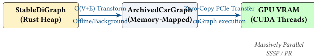
Figure 24. The Graph-to-GPU Pipeline. Because pointer-based graphs cannot be sent to the GPU, the adjacency list is serialized into a flattened Compressed Sparse Row (CSR) structure, which is then DMA-transferred to the GPU for parallel analytics.
