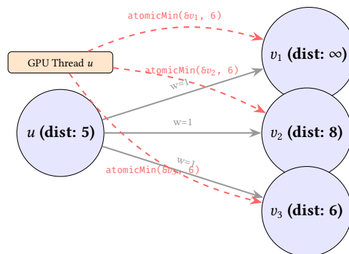
Figure 25. GPU SSSP relaxation. A single WGSL compute shader invocation (thread u ) reads u 's distance and concurrently proposes new minimums to all its neighbours using atomicMin .
