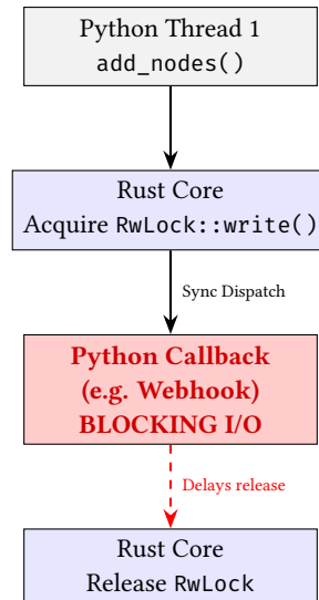
Figure 28. The Event Callback Danger Zone. Synchronous callbacks hold the engine’s global write lock. Future versions will move to a lock-free async queue design.
