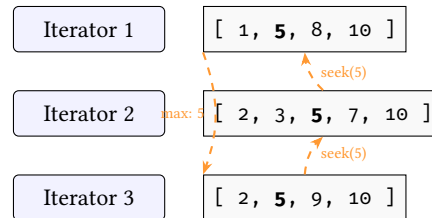
Figure 35. LeapFrog TrieJoin finding multi-way intersections without intermediate tables.
