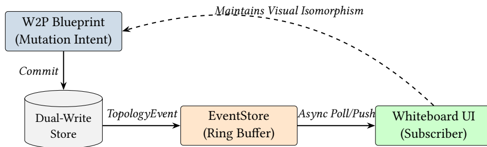
Figure 27. The Reactive Event Pipeline. Structural and relational changes are emitted as typed events, which bridge the physical storage layer back to the visual Blueprint domain.
