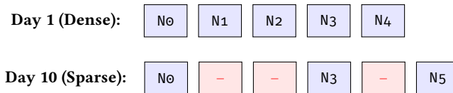
Figure 34. StableDiGraph Fragmentation. Deletions leave index holes. Over time, heavy mutation destroys spatial locality in memory, degrading CPU cache performance.
