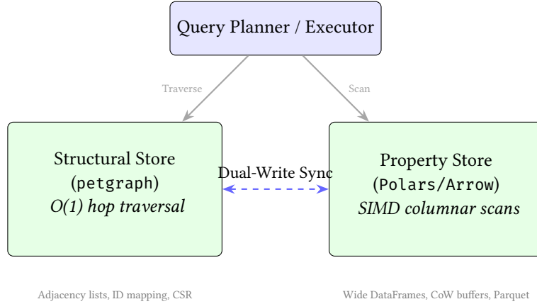
Figure 9. Dual-write architecture synergy. Structural queries target the graph engine, while property-heavy predicates target the columnar store.
