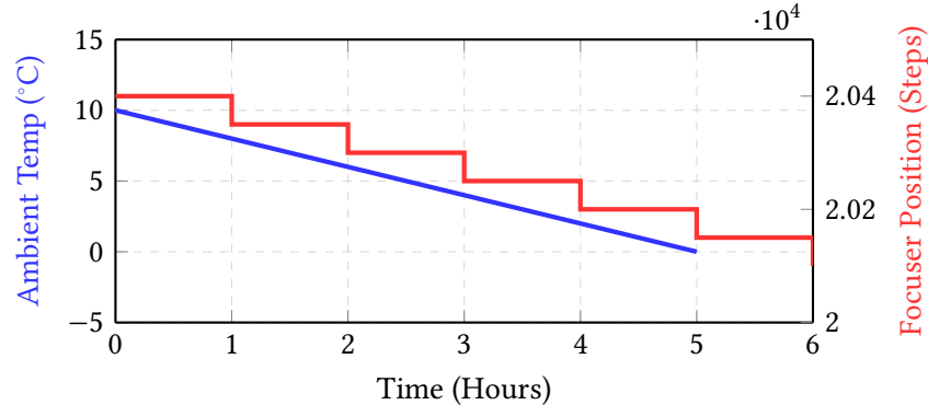
Figure 24. Temperature compensation loop. As the ambient temperature drops steadily (blue), the astro-node daemon autonomously injects computed inward micro-steps to the focuser (red) to maintain critical focus without requiring a sequence-interrupting V-Curve scan.
