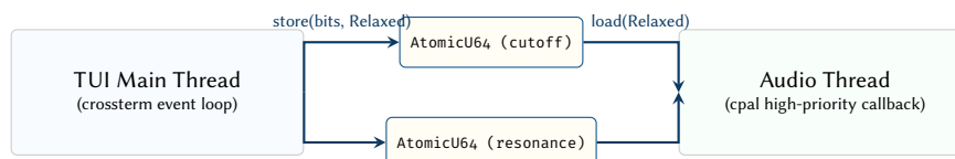
Figure 35. Lock-free concurrency model. The UI thread communicates with the real-time audio thread strictly through atomic variables, preventing priority inversion and guaranteeing that the audio callback never blocks waiting for a mutex.
