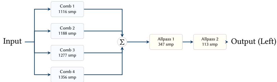
Figure 11. Schroeder Reverb topology (Left Channel). The input signal is fed in parallel to four comb filters with mutually prime delay lengths. Their outputs are summed and passed serially through two allpass filters to increase echo density without coloring the sound.
