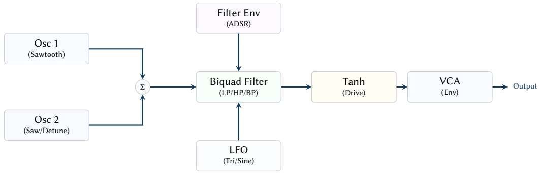
Figure 7. The bass synth signal flow. Dual sawtooth oscillators are summed and passed through a multi-mode biquad filter. Cutoff frequency is modulated by both an ADSR envelope and a free-running LFO. The signal is then saturated via a tanh function and shaped by the VCA envelope.
