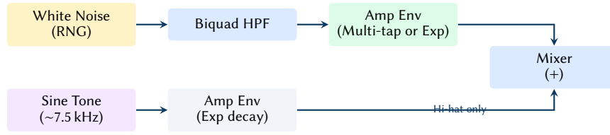
Figure 8. Percussion synthesis model. Hi-hats blend filtered noise with a metallic sine tone, while the clap relies entirely on a multi-tap noise envelope.
