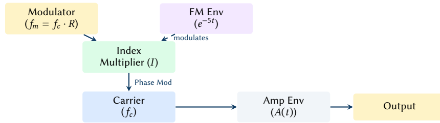
Figure 9. Lead synthesiser signal flow using 2-operator FM.
