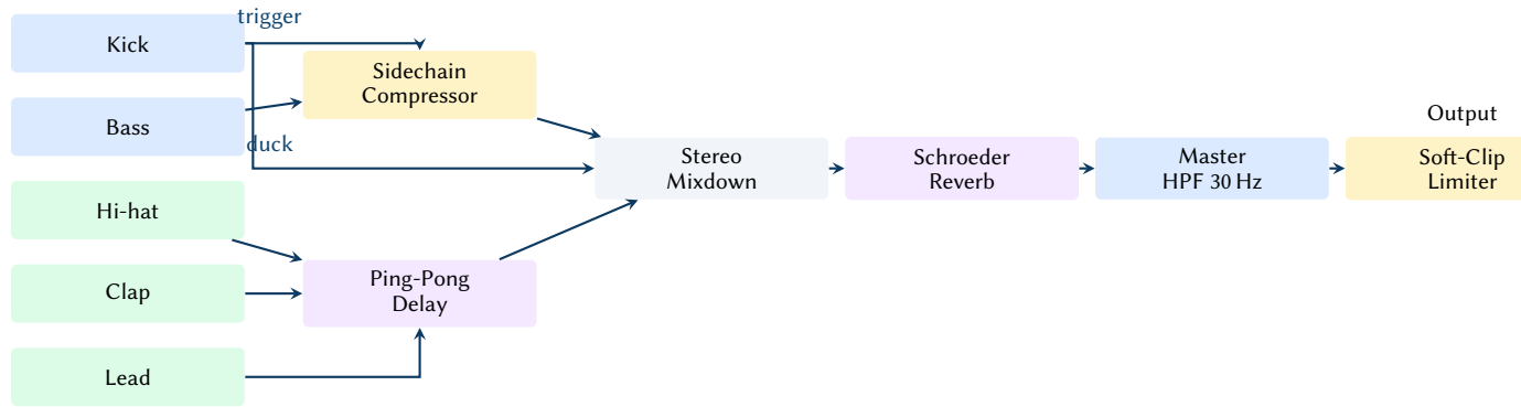
Figure 10. Master effects signal flow. The kick triggers the sidechain compressor which ducks the bass. Hi-hat, clap, and lead pass through the ping-pong delay before joining the stereo bus.
