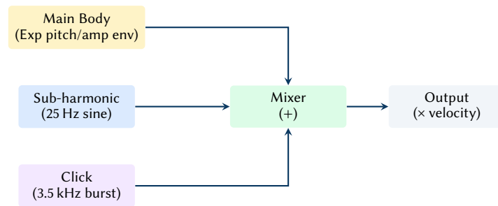
Figure 6. Kick drum synthesis model: parallel summation of main body, sub-harmonic, and click layers.
