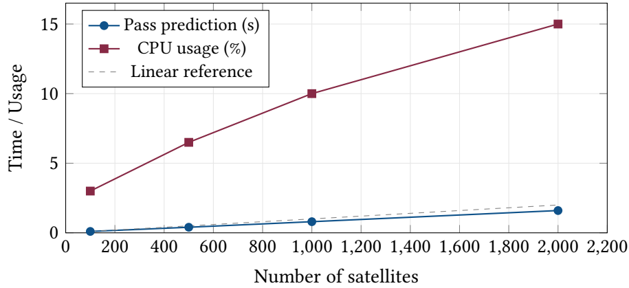
Figure 3. Resource scaling with satellite count. Both CPU usage (mid-range values) and pass prediction time scale linearly. The dashed line shows ideal linear scaling from the 100-satellite baseline.
