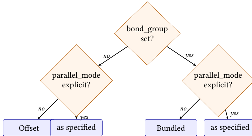
Figure 18. Parallel edge mode selection logic. Bond groups default to Bundled; non-bonded parallel edges default to Offset. An explicit parallel_mode always overrides the default.
