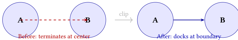
Figure 27. EdgeClippingRefiner: without clipping, edge paths terminate at node centers; with clipping, endpoints dock at the exact node shape boundary, giving correct arrowhead placement regardless of shape.
