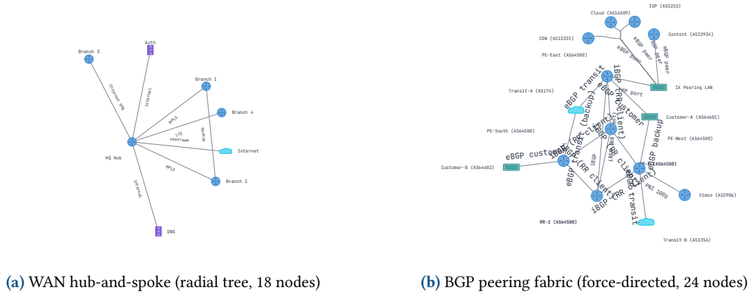
Figure 1. Representative NetVis outputs. All diagrams generated automatically from YAML with no manual adjustment.
