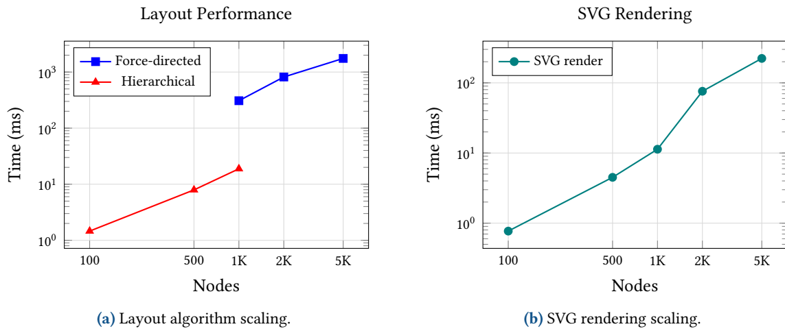
Figure 31. NetVis benchmark results on spine-leaf topologies. Left: layout computation time for force-directed (Barnes–Hut) and hierarchical (Sugiyama) engines. Right: SVG rendering time including label placement. Both axes are log-scaled; data points are median wall-clock times.
