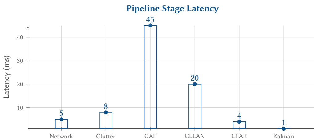
Figure 4. Real-time latency breakdown per beam (CIT = 100ms). The FFT-based CAF computation dominates processing time.
