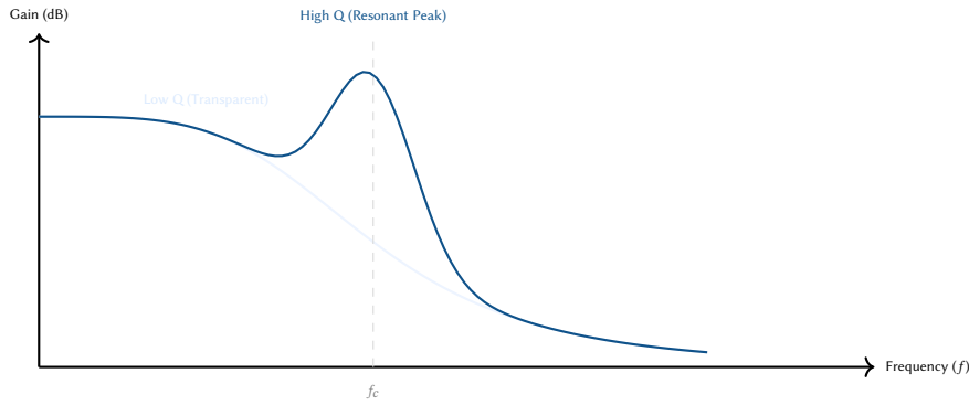
Figure 11. Filter response geometries. The "Acid" character is achieved by a sharp resonant peak at the cutoff frequency ( f_c ). When the cutoff is modulated by a fast envelope, this peak sweeps through the harmonics of the sawtooth oscillator, creating the characteristic "wow" and "squelch" textures.
