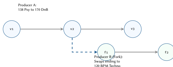
Figure 61. The Generative Git-Tree. Sets can be forked and collaboratively edited. When Producer B swaps the ending chapter, the engine automatically recalculates the transition bridges without requiring the transfer of massive audio stems.
