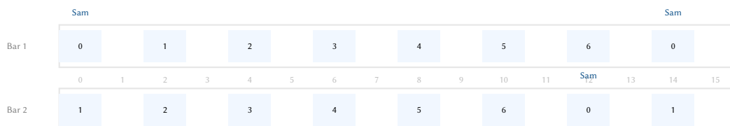
Figure 27. Tala-to-grid alignment. A 7-beat Rupak cycle (mapped here to 8th-note steps) drifts relative to the 16-step bar boundary. The Sam (beat 0) moves from step 0 in Bar 1 to step 14 in Bar 1, and step 12 in Bar 2, creating evolving syncopation.
