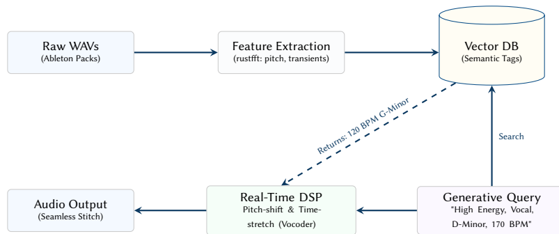
Figure 64. The Semantic Sample Stitching pipeline. During ingestion, samples are analyzed and stored in a vector database. During generation, the engine queries the DB based on the current thematic context, retrieves the best match, and dynamically time-stretches and pitch-shifts the audio to fit the active pocket.
