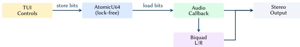
Figure 57. Lock-free live parameter path: the TUI stores f64 bit patterns into atomics; the audio callback loads them each block and updates the biquad filter only when thresholds are exceeded.
