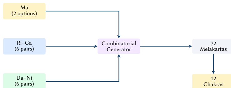
Figure 33. Melakarta generation: three independent pitch choices yield 72 canonical ragas grouped into 12 chakras.
