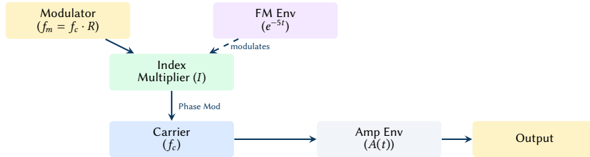
Figure 14. Lead synthesiser signal flow using 2-operator FM.
