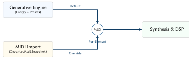
Figure 53. MIDI Import overriding architecture. Users can selectively replace the generative output of specific elements (e.g., locking in a custom bassline) while allowing the engine to continue generating the rest of the arrangement (drums, leads, drones).
