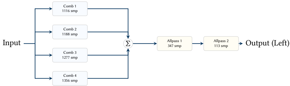
Figure 19. Schroeder Reverb topology (Left Channel). The input signal is fed in parallel to four comb filters with mutually prime delay lengths. Their outputs are summed and passed serially through two allpass filters to increase echo density without coloring the sound.
