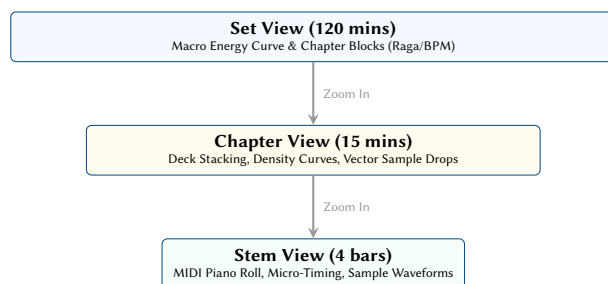
Figure 62. The Semantic Zoom interface. At the macro level, users arrange the global energetic flow. At the micro level, they edit precise MIDI syncopation. Edits made at the stem level automatically recalculate the structural tension displayed at the set level.
