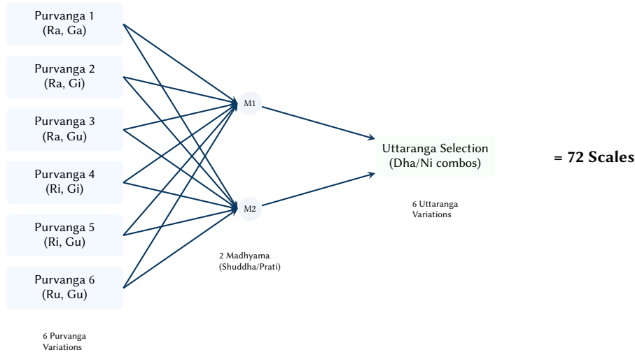
Figure 32. The combinatorial logic of the 72 Melakartas. Six purvanga variations are multiplied by two madhyama positions and six uttaranga variations ( 6 \times 2 \times 6 = 72 ). Each group of six purvanga/madhyama combinations forms a Chakra .
