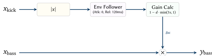
Figure 17. Sidechain compression signal flow. The absolute value of the kick signal drives an envelope follower with instantaneous attack and exponential release. This envelope calculates a dynamic gain reduction ( g_{\text{sc}} ) which is multiplied against the bass signal, ducking it to create rhythmic pumping.
