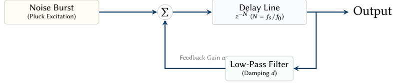
Figure 15. Karplus-Strong physical modeling architecture. A short burst of noise (the "pluck") is fed into a delay line representing the string length. The output is fed back through a low-pass filter, causing higher frequencies to decay faster than fundamental frequencies, realistically simulating a plucked acoustic string.
