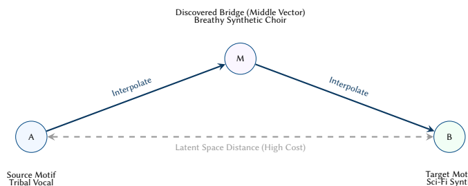
Figure 65. Latent space motif interpolation. When bridging two structurally distant chapters, the engine calculates the latent vector between their respective samples (A and B). It queries the database for a sample (M) that sits mathematically between them, creating a sonically logical bridge that a human might never have searched for.
