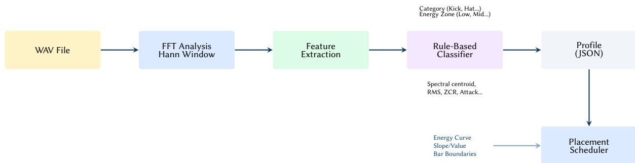
Figure 23. The sample intelligence pipeline. Raw audio is processed via spectral analysis to extract acoustic features, classified into categories and energy zones, and stored as JSON profiles. The scheduler then uses macro energy state to place samples across the arrangement.
