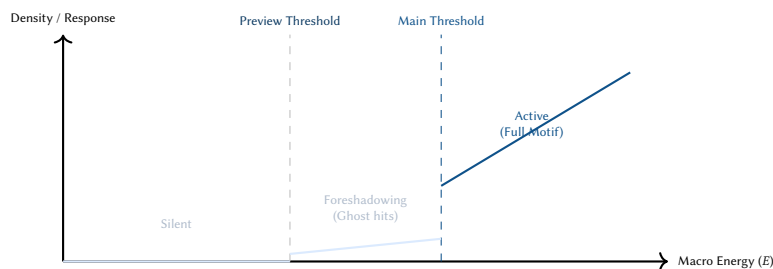
Figure 29. The Sub-Channel Preview mechanism. Instead of an abrupt binary switch when an element becomes active, the engine provides a "preview window." In this energy band, the element emits occasional low-velocity hits, telegraphing its arrival to the listener before full activation.
