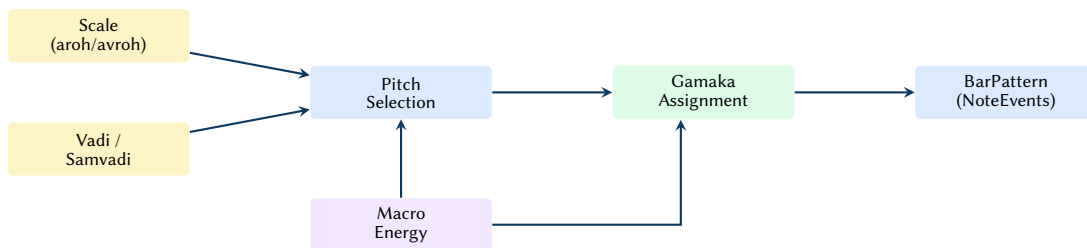
Figure 25. Raga melody generation: scale constraints and vadi/samvadi weighting feed pitch selection, energy controls density and ornamentation depth, and gamaka rules produce per-note ornaments.
