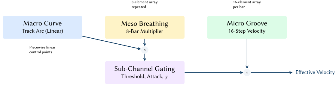
Figure 8. The four-level energy hierarchy. Macro and meso levels combine to drive the sub-channel gate, which is then modulated by the micro groove to produce the final step velocity.
