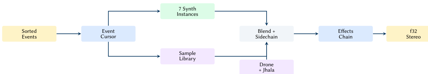
Figure 56. Streaming engine architecture: pre-sorted events are dispatched sample-accurately, blended with energy-aware sample playback, and processed through the effects chain.
