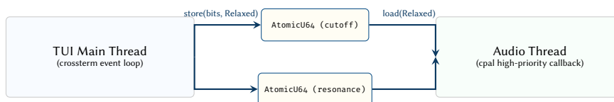
Figure 59. Lock-free concurrency model. The UI thread communicates with the real-time audio thread strictly through atomic variables, preventing priority inversion and guaranteeing that the audio callback never blocks waiting for a mutex.
