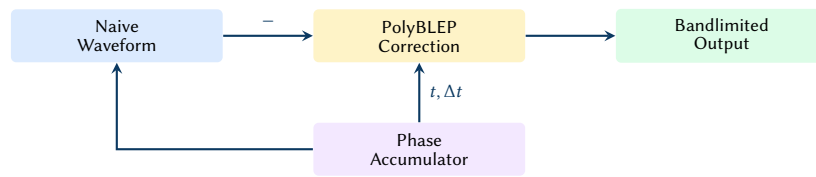
Figure 22. PolyBLEP anti-aliasing: the correction term is subtracted from the naive waveform at phase discontinuities.
