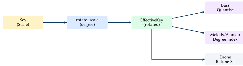
Figure 34. Murchhana integration: the original scale is rotated by degree, producing an EffectiveKey that is threaded through bass quantisation, melody generation, and drone retuning.
