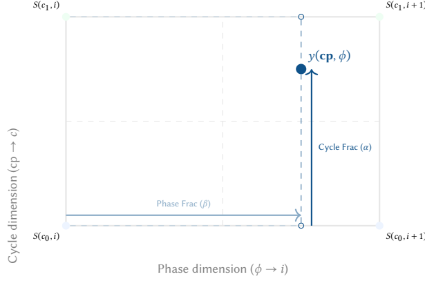
Figure 20. Bilinear cross-cycle interpolation in the Wavetable Oscillator. To prevent zipper noise when sweeping wavetables and aliasing when playing high pitches, the engine first interpolates horizontally between adjacent samples ( i and i + 1 ) within two adjacent wave cycles ( c_0 and c_1 ), and then interpolates vertically between the resulting values.
