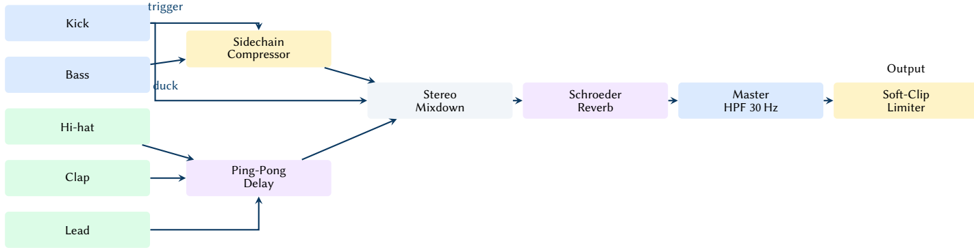
Figure 16. Master effects signal flow. The kick triggers the sidechain compressor which ducks the bass. Hi-hat, clap, and lead pass through the ping-pong delay before joining the stereo bus.
