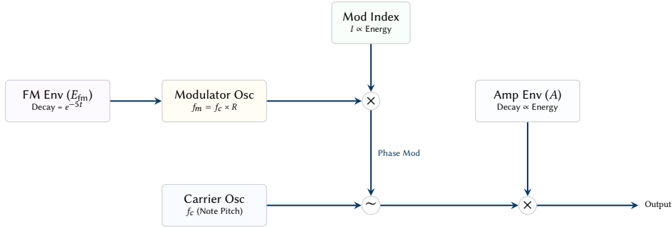
Figure 13. Two-operator FM Synthesis architecture. The modulator oscillator frequency ( f_m ) is a ratio ( R ) of the carrier pitch. The modulation depth (Index I ) is dynamically scaled by the macro energy level, meaning higher energy sections produce much brighter, richer sideband harmonics. The FM envelope ( E_{fm} ) creates a "pluck" or "wow" transient.
