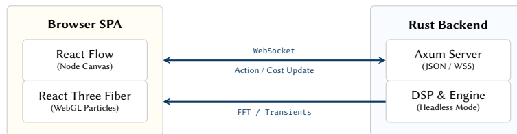
Figure 68. The Web UI Architecture. The Rust backend runs headless, exposing an Axum server. The React frontend syncs the Timeline state via WebSockets. The audio engine streams FFT and transient data directly to the Three.js particle system for zero-latency audio-reactive visuals.
