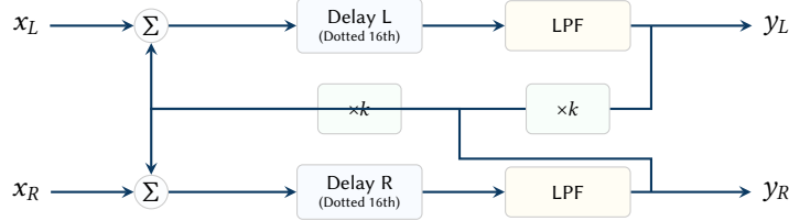
Figure 18. Ping-Pong Delay topology. Left and right channel inputs ( x_L , x_R ) are fed into independent delay lines. The output of each delay line is low-pass filtered (for analog-style damping), multiplied by the feedback coefficient k , and routed into the input sum of the opposite channel's delay line, creating a stereo bouncing effect.
