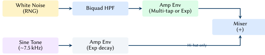
Figure 12. Percussion synthesis model. Hi-hats blend filtered noise with a metallic sine tone, while the clap relies entirely on a multi-tap noise envelope.
