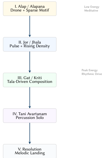
Figure 30. The performance arc implemented in Overtone. The engine maps the traditional Indian classical progression onto the EDM energy model, moving from non-metered melodic exploration to high-density rhythmic cycles.
