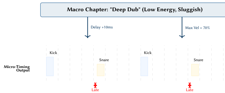
Figure 66. Macro-driven micro-timing. The global thematic state cascades down to the lowest level of the engine, algorithmically pushing notes off the rigid 16th-note grid and scaling absolute MIDI velocities to match the emotional intent of the chapter.
