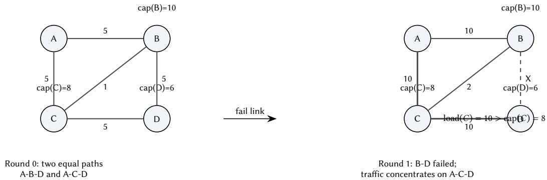
Figure 24. Toy cascade: rerouting after a single failure can overload a different component and trigger secondary failures.
