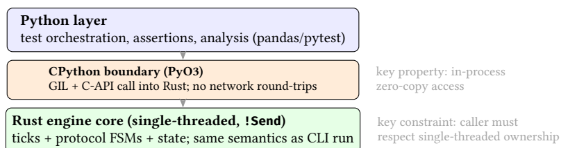
Figure 27. Python Bindings as a Process Boundary, Not a Protocol Boundary. PyO3 exposes the same single-threaded engine core directly to Python. The integration cost is GIL/FFI semantics, while the benefit is in-process access without serialization or RPC latency.
