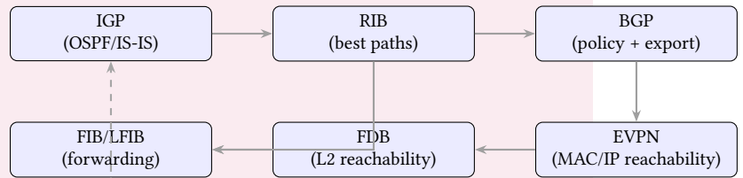
Figure 17. EVPN Synchronisation as a Consistency Model. Per-message queuing exposes the simulation to ordering-dependent behaviour. netsim instead snapshots all EVPN Loc-RIBs once per tick (Phase P2.5) and applies the same snapshot everywhere, providing a deterministic barrier that preserves “simultaneous” control-plane state replication.
