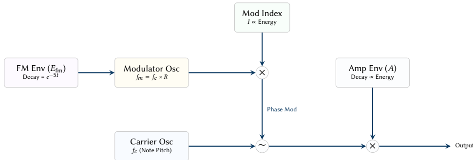
Figure 17. Two-operator FM Synthesis architecture. The modulator oscillator frequency ( f_m ) is a ratio ( R ) of the carrier pitch. The modulation depth (Index I ) is dynamically scaled by the macro energy level, meaning higher energy sections produce much brighter, richer sideband harmonics. The FM envelope ( E_{fm} ) creates a “pluck” or “wow” transient.
