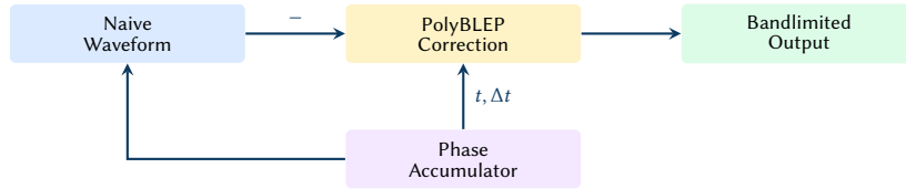
Figure 27. PolyBLEP anti-aliasing: the correction term is subtracted from the naive waveform at phase discontinuities.
