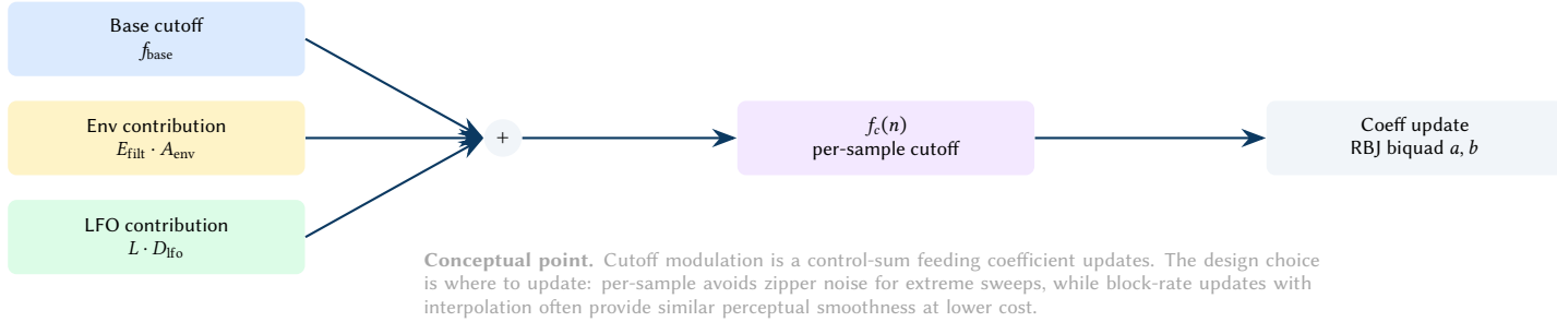
Figure 15. Filter modulation as a control-sum graph. Multiple modulation sources sum into f_c(n) , which drives coefficient updates and then sample processing.
