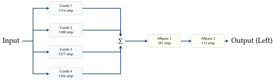
Figure 24. Schroeder Reverb topology (Left Channel). The input signal is fed in parallel to four comb filters with mutually prime delay lengths. Their outputs are summed and passed serially through two allpass filters to increase echo density without coloring the sound.
