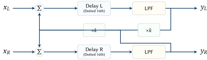
Figure 23. Ping-Pong Delay topology. Left and right channel inputs ( x_L , x_R ) are fed into independent delay lines. The output of each delay line is low-pass filtered (for analog-style damping), multiplied by the feedback coefficient k , and routed into the input sum of the opposite channel's delay line, creating a stereo bouncing effect.
