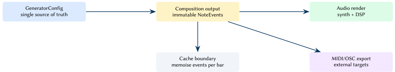
Figure 8. The decoupled pipeline architecture. The Composition stage (I) is deterministic and produces a structured event set. This set can then be rendered to high-precision audio (IIa) or exported directly to external environments (IIb).
