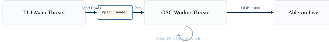
Figure 67. Non-blocking OSC Push architecture. The TUI sends sequences of commands (Delete → Create → Add Notes) via a channel. The background worker consumes this queue and handles the necessary network sleeps without stalling the rendering loop.
