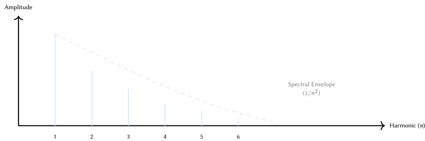
Figure 60. Additive synthesis model for the Shruti Box. The engine sums the first six harmonics of the tonic (Sa) and the fifth (Pa) with amplitudes decaying at a rate of 1/n^2 . A slow bellows-like amplitude LFO is applied to simulate the manual pumping of the instrument.
