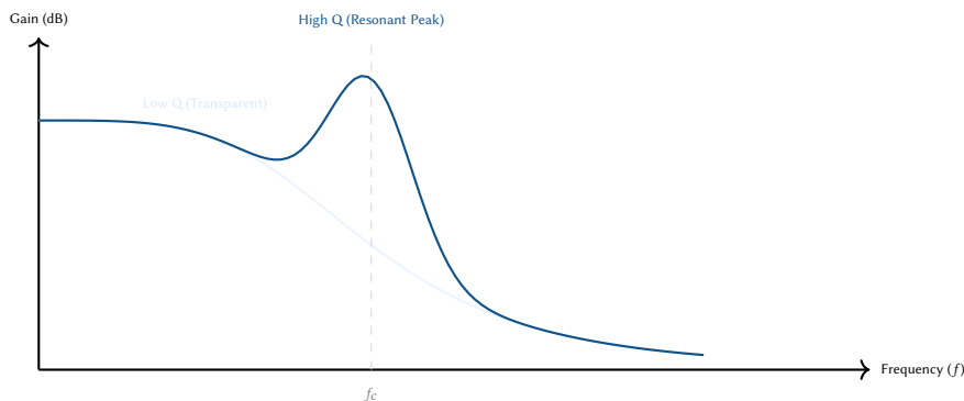
Figure 14. Filter response geometries. The "Acid" character is achieved by a sharp resonant peak at the cutoff frequency ( f_c ). When the cutoff is modulated by a fast envelope, this peak sweeps through the harmonics of the sawtooth oscillator, creating the characteristic "wow" and "squelch" textures.
