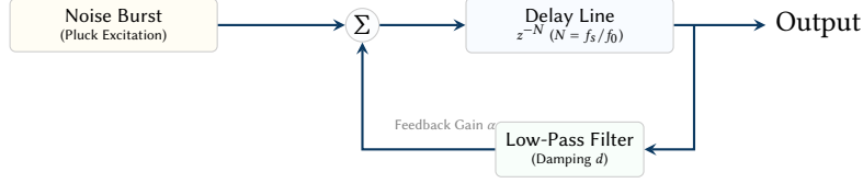
Figure 19. Karplus-Strong physical modeling architecture. A short burst of noise (the "pluck") is fed into a delay line representing the string length. The output is fed back through a low-pass filter, causing higher frequencies to decay faster than fundamental frequencies, realistically simulating a plucked acoustic string.
