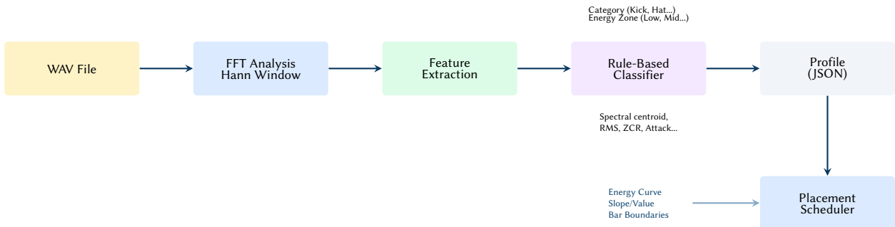
Figure 29. The sample intelligence pipeline. Raw audio is processed via spectral analysis to extract acoustic features, classified into categories and energy zones, and stored as JSON profiles. The scheduler then uses macro energy state to place samples across the arrangement.
