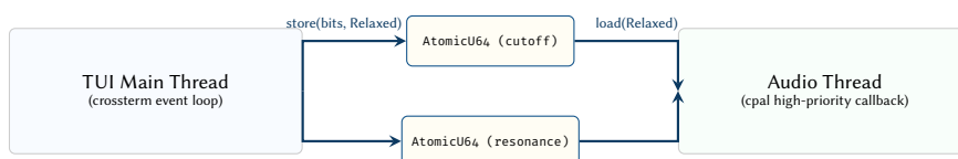
Figure 74. Lock-free concurrency model. The UI thread communicates with the real-time audio thread strictly through atomic variables, preventing priority inversion and guaranteeing that the audio callback never blocks waiting for a mutex.
