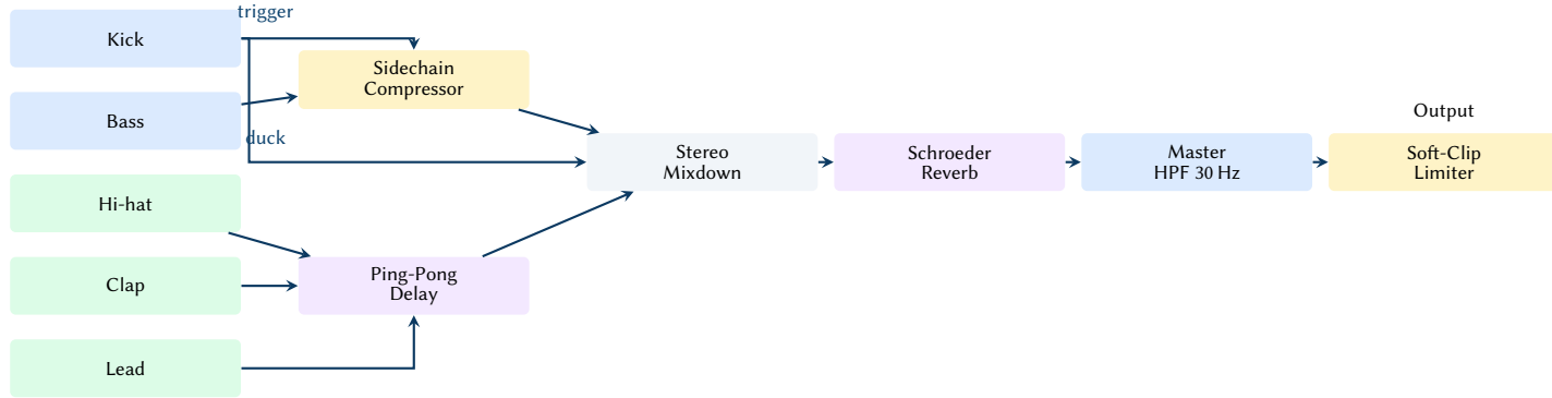
Figure 20. Master effects signal flow. The kick triggers the sidechain compressor which ducks the bass. Hi-hat, clap, and lead pass through the ping-pong delay before joining the stereo bus.
