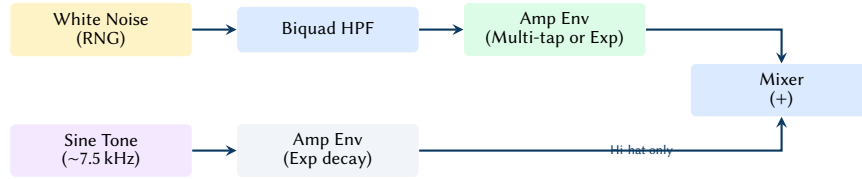
Figure 16. Percussion synthesis model. Hi-hats blend filtered noise with a metallic sine tone, while the clap relies entirely on a multi-tap noise envelope.
