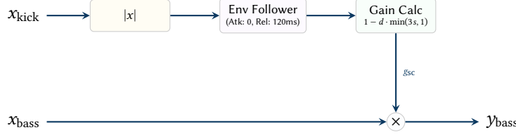
Figure 22. Sidechain compression signal flow. The absolute value of the kick signal drives an envelope follower with instantaneous attack and exponential release. This envelope calculates a dynamic gain reduction ( g_{sc} ) which is multiplied against the bass signal, ducking it to create rhythmic pumping.
