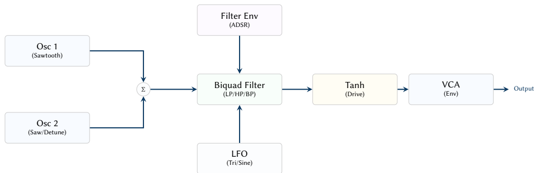
Figure 13. The bass synth signal flow. Dual sawtooth oscillators are summed and passed through a multi-mode biquad filter. Cutoff frequency is modulated by both an ADSR envelope and a free-running LFO. The signal is then saturated via a tanh function and shaped by the VCA envelope.
