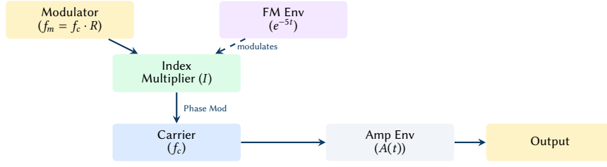
Figure 18. Lead synthesiser signal flow using 2-operator FM.
