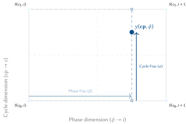
Figure 25. Bilinear cross-cycle interpolation in the Wavetable Oscillator. To prevent zipper noise when sweeping wavetables and aliasing when playing high pitches, the engine first interpolates horizontally between adjacent samples ( i and i + 1 ) within two adjacent wave cycles ( c_0 and c_1 ), and then interpolates vertically between the resulting values.
